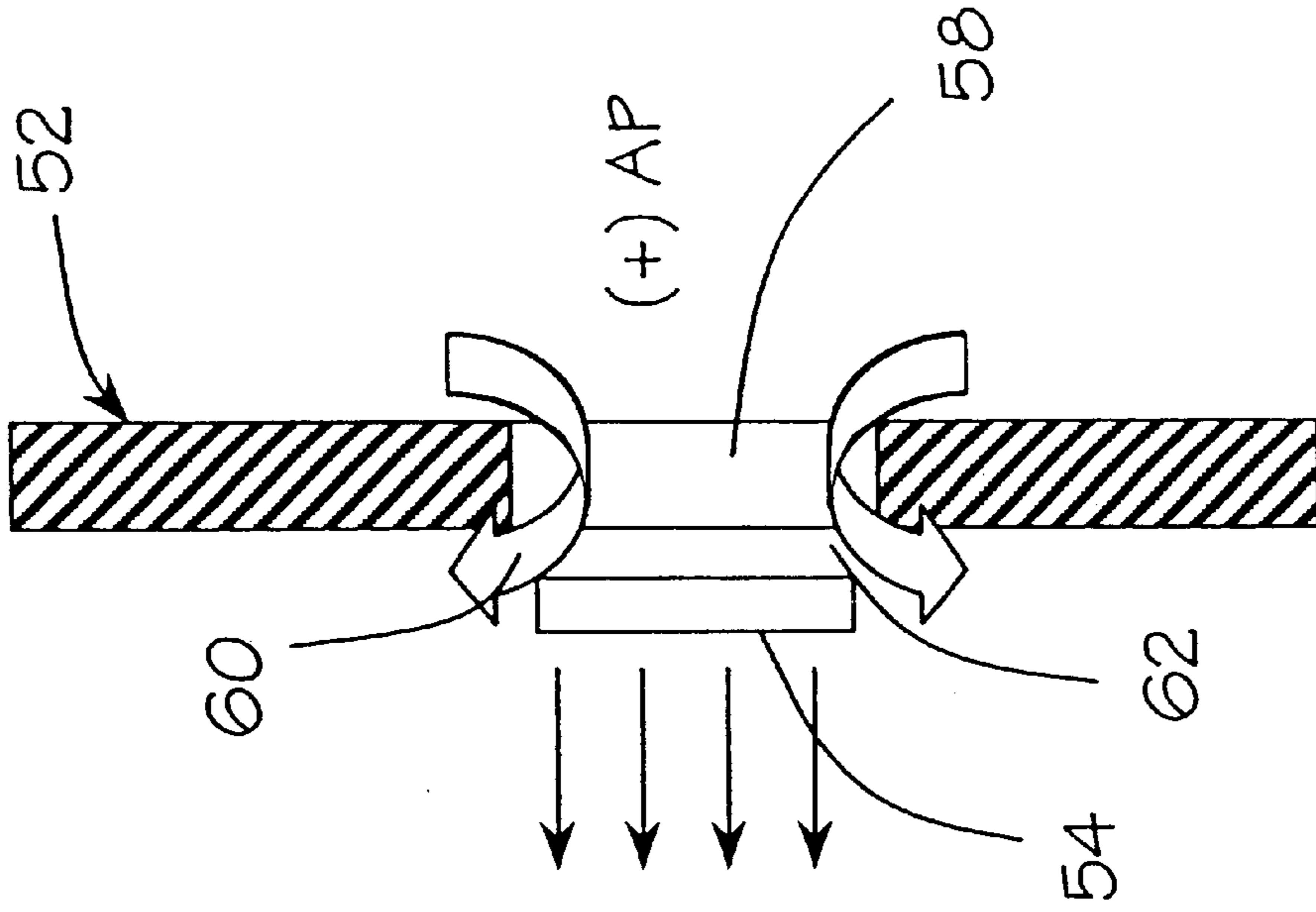
FIG. 6 (Prior Art)
