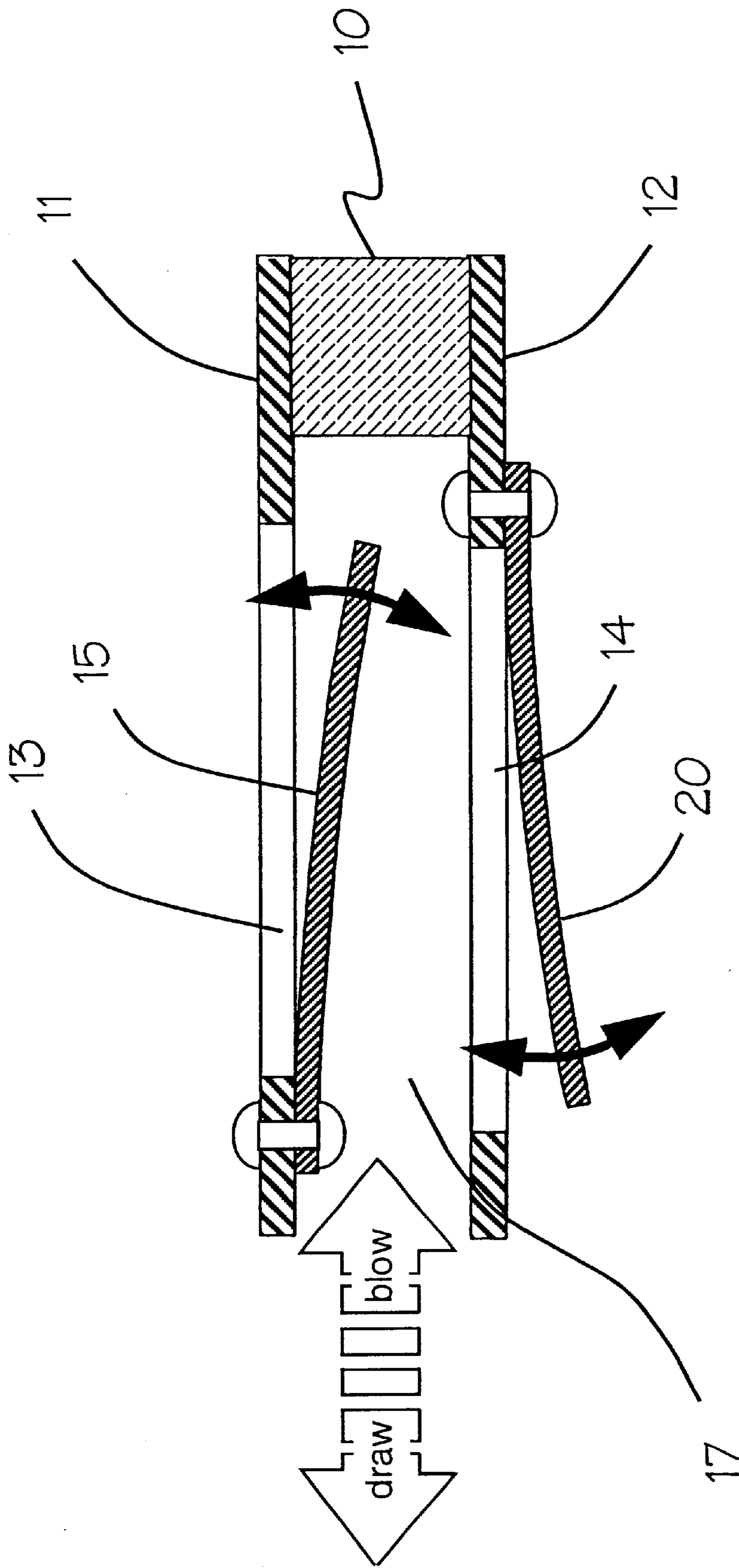
FIG. 2 (Prior Art)
