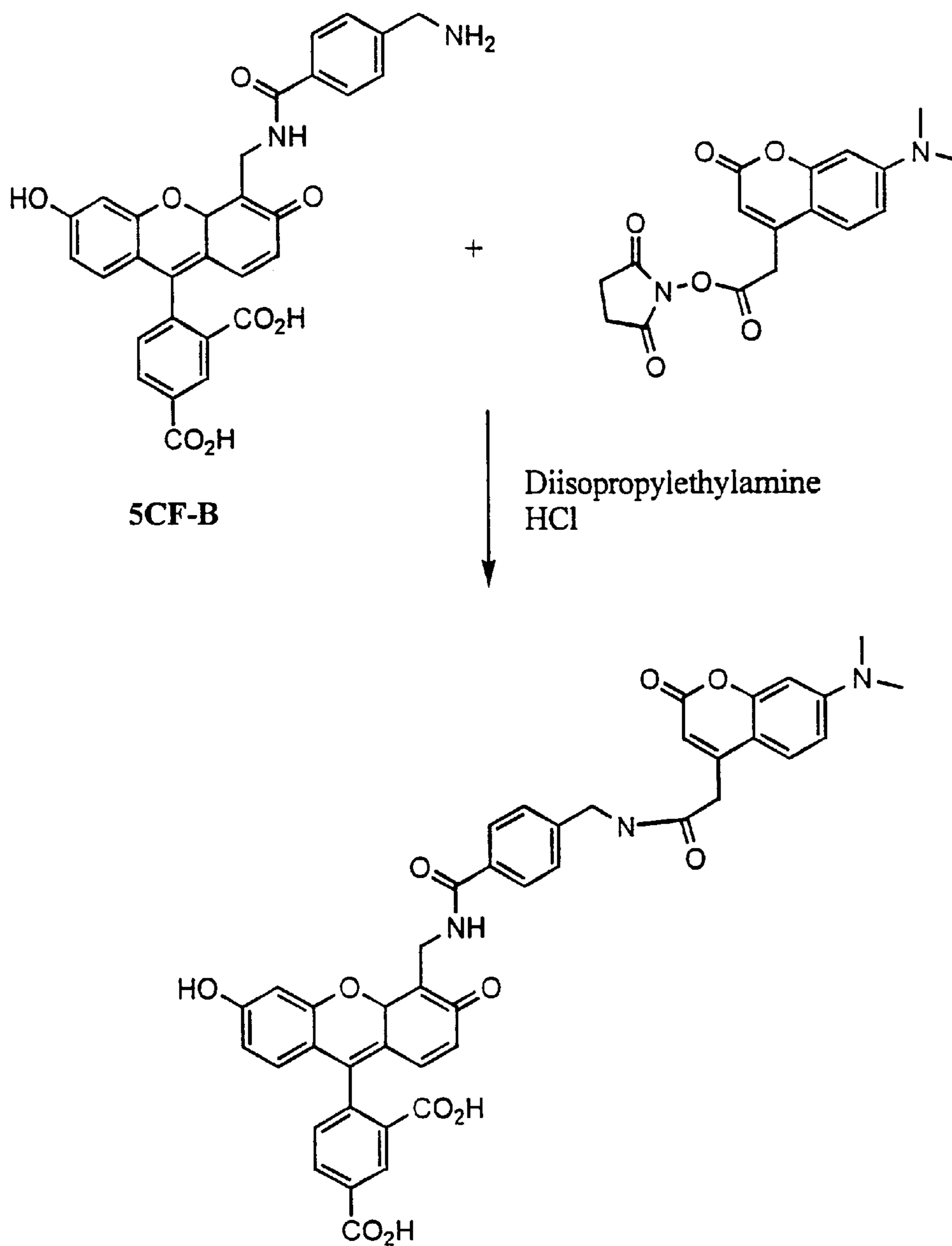
DYE106
