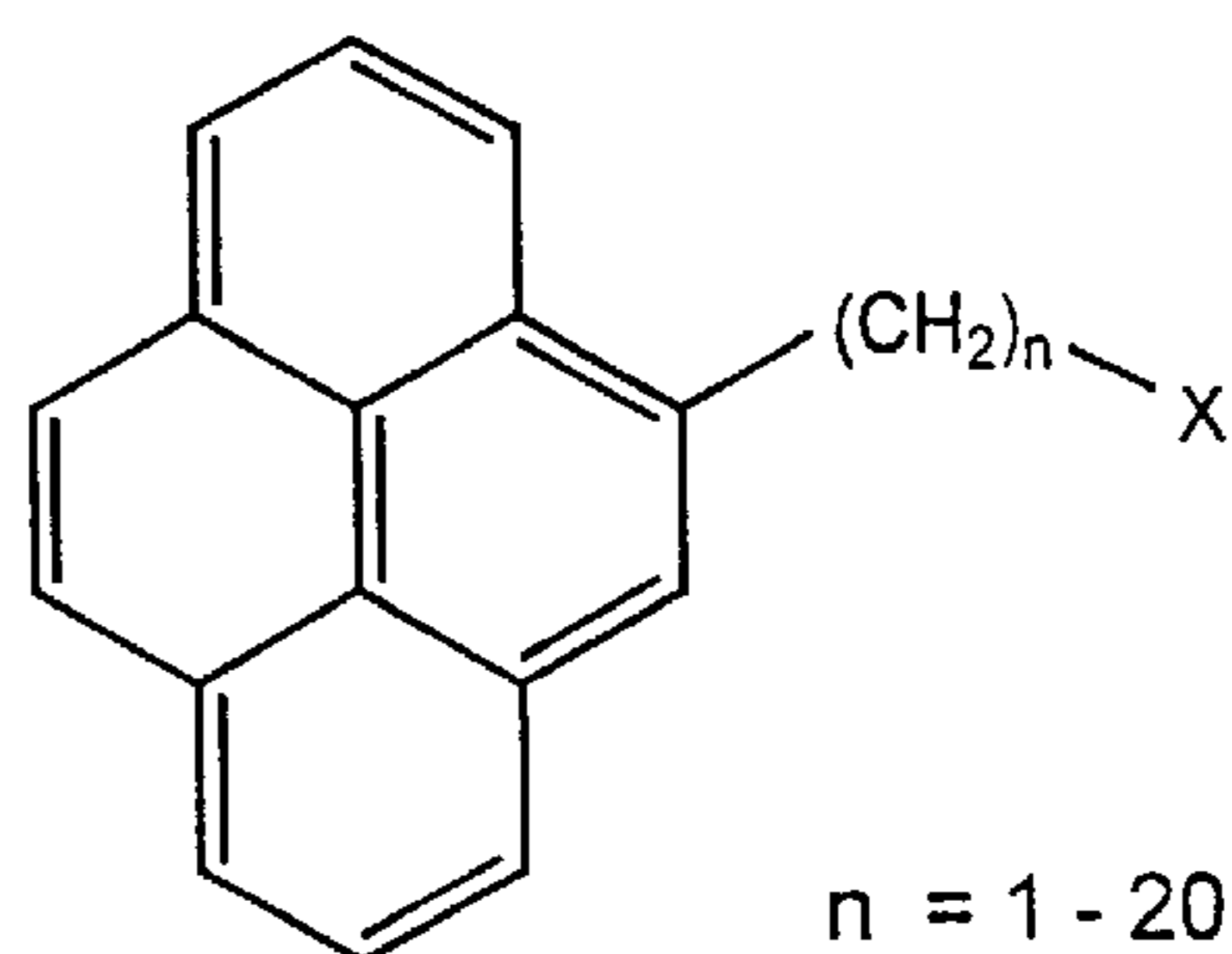
DYE126
