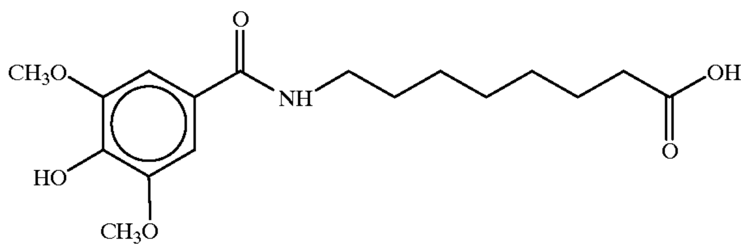
8-(N-(3,5-Dimethoxy 4-hydroxybenzoyl)aminocaprylic acid
