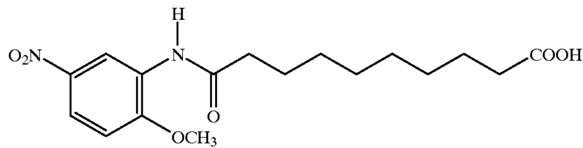
N-(2-methoxy-5-nitrophenyl) sebecoyl amide acid
