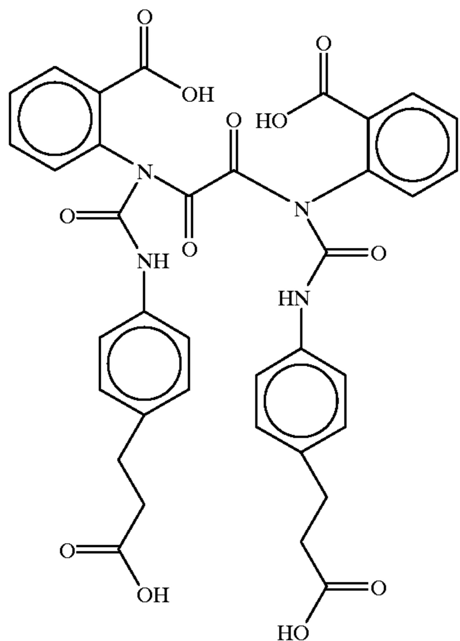
Bis(N-2-carboxyphenyl-N-(N'-3(4-aminophenyl)propionic acid)urea)oxalyl diamide
