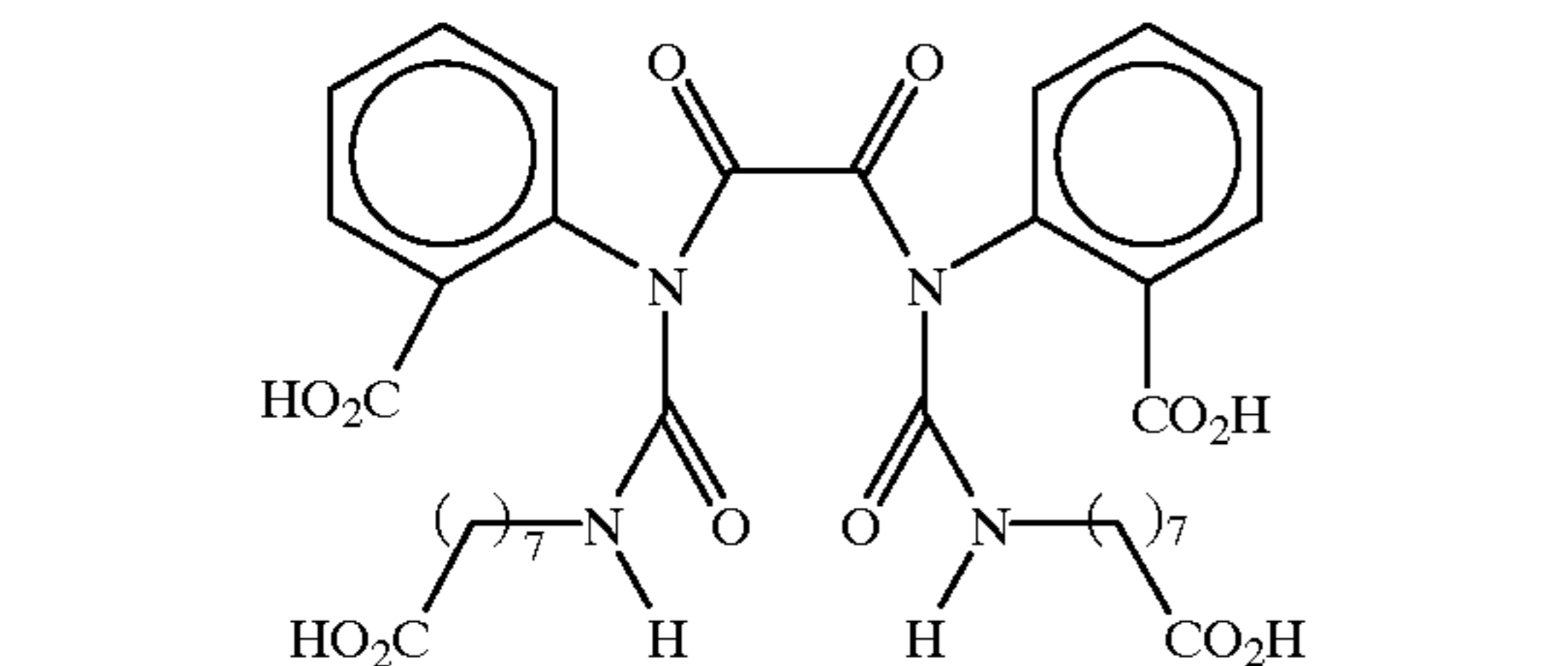
Bis(N-2-carboxylphenyl-N-(N'-8-octanoic acid)ureal)oxalyl diamide
