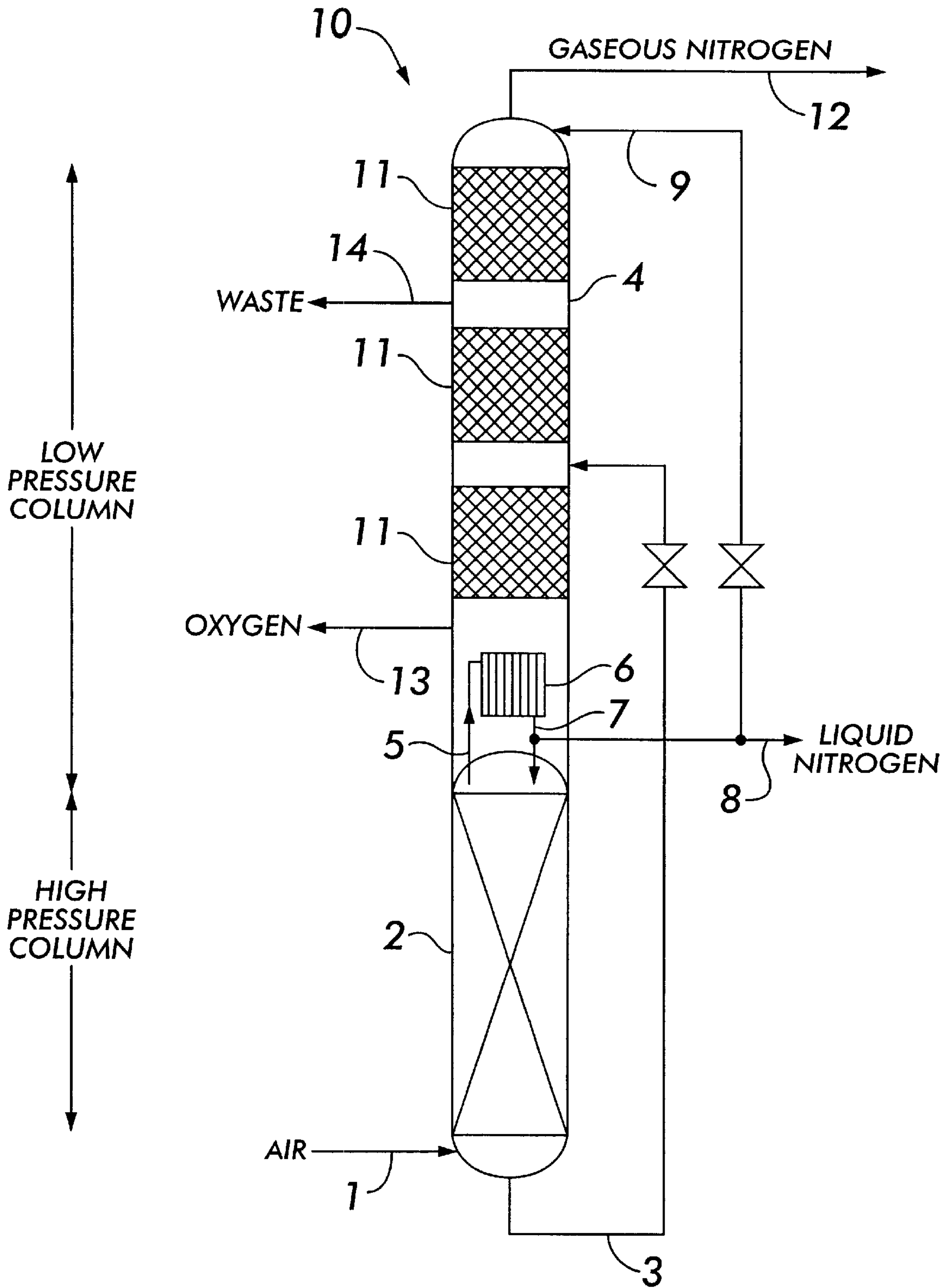
FIG. 1 PRIOR ART
