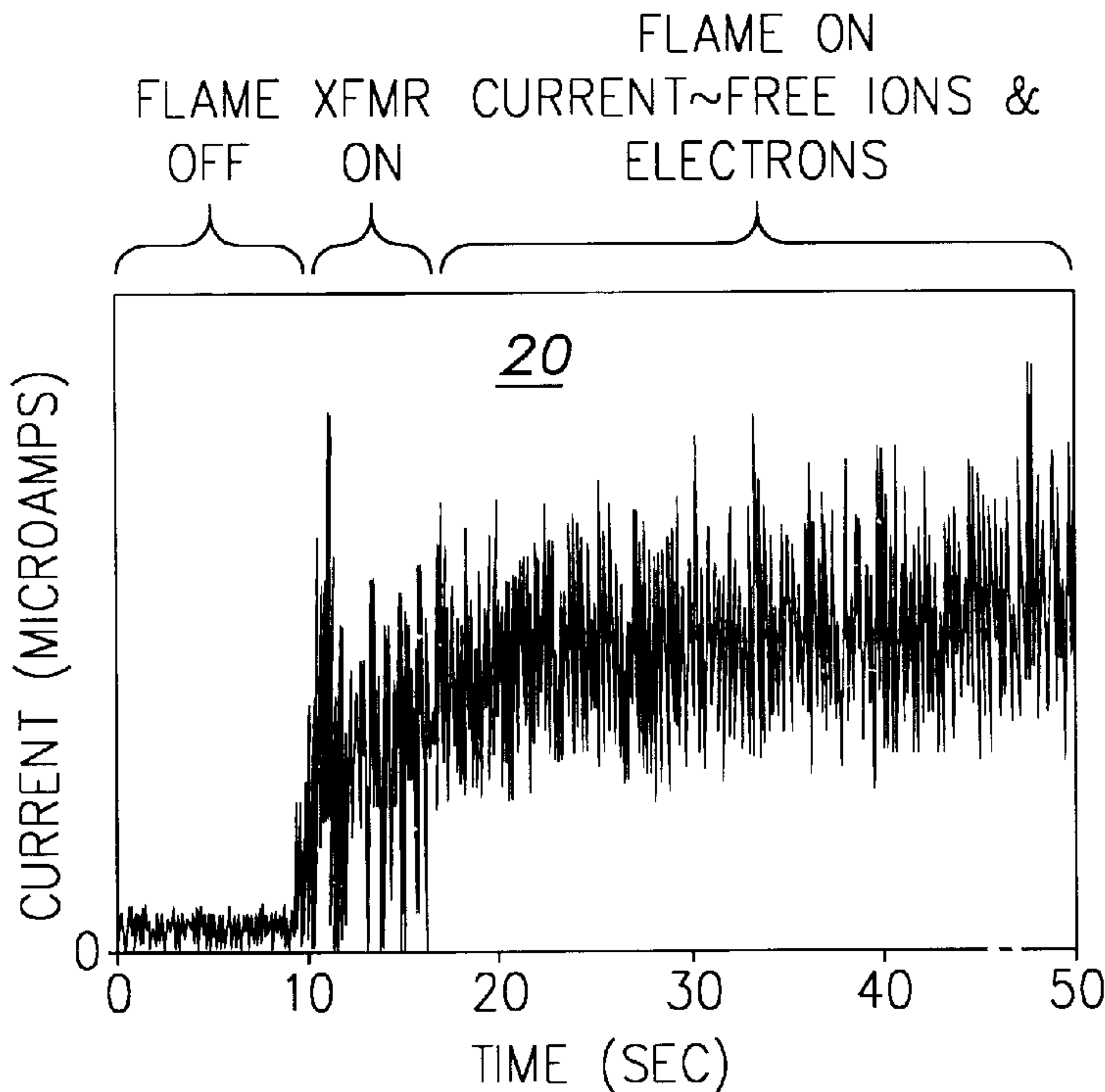
IONIZATION CURRENT FROM 1FM ROD IN IGNITOR FLAME
