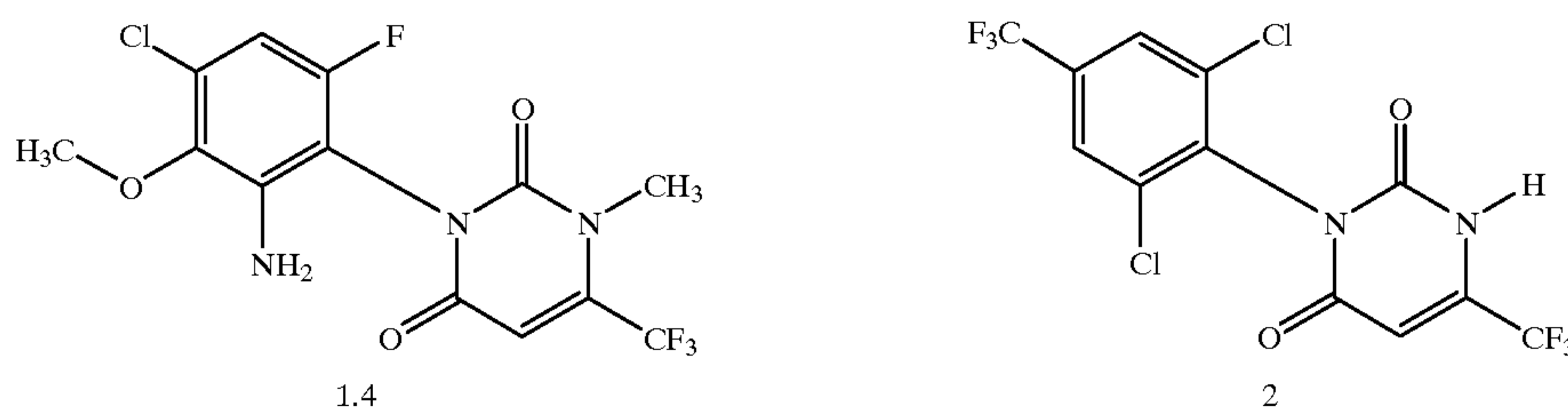
Comparative herbicidal activity of compounds 1.4 and 2
