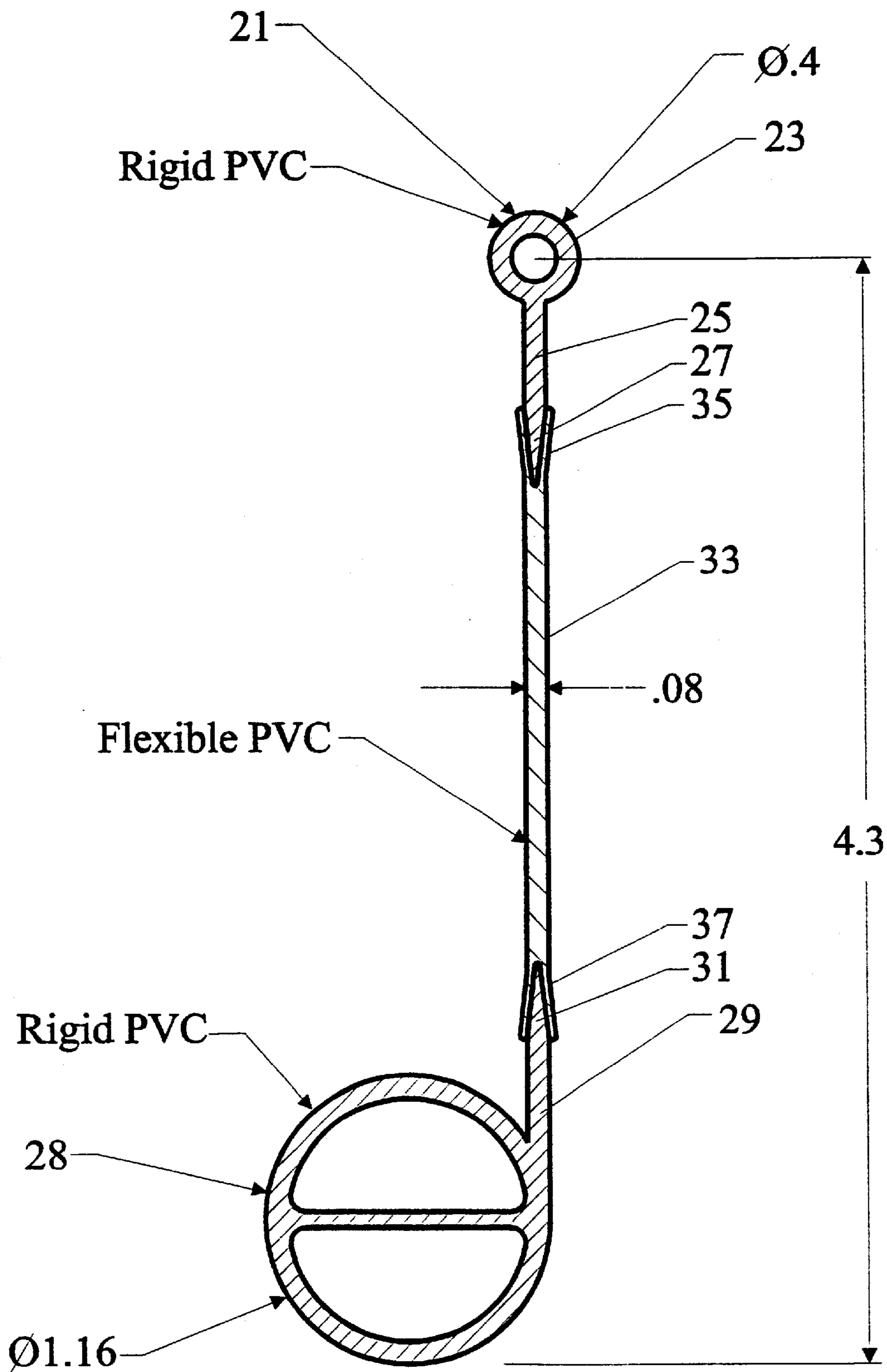
Figure 2 (PRIOR ART)
