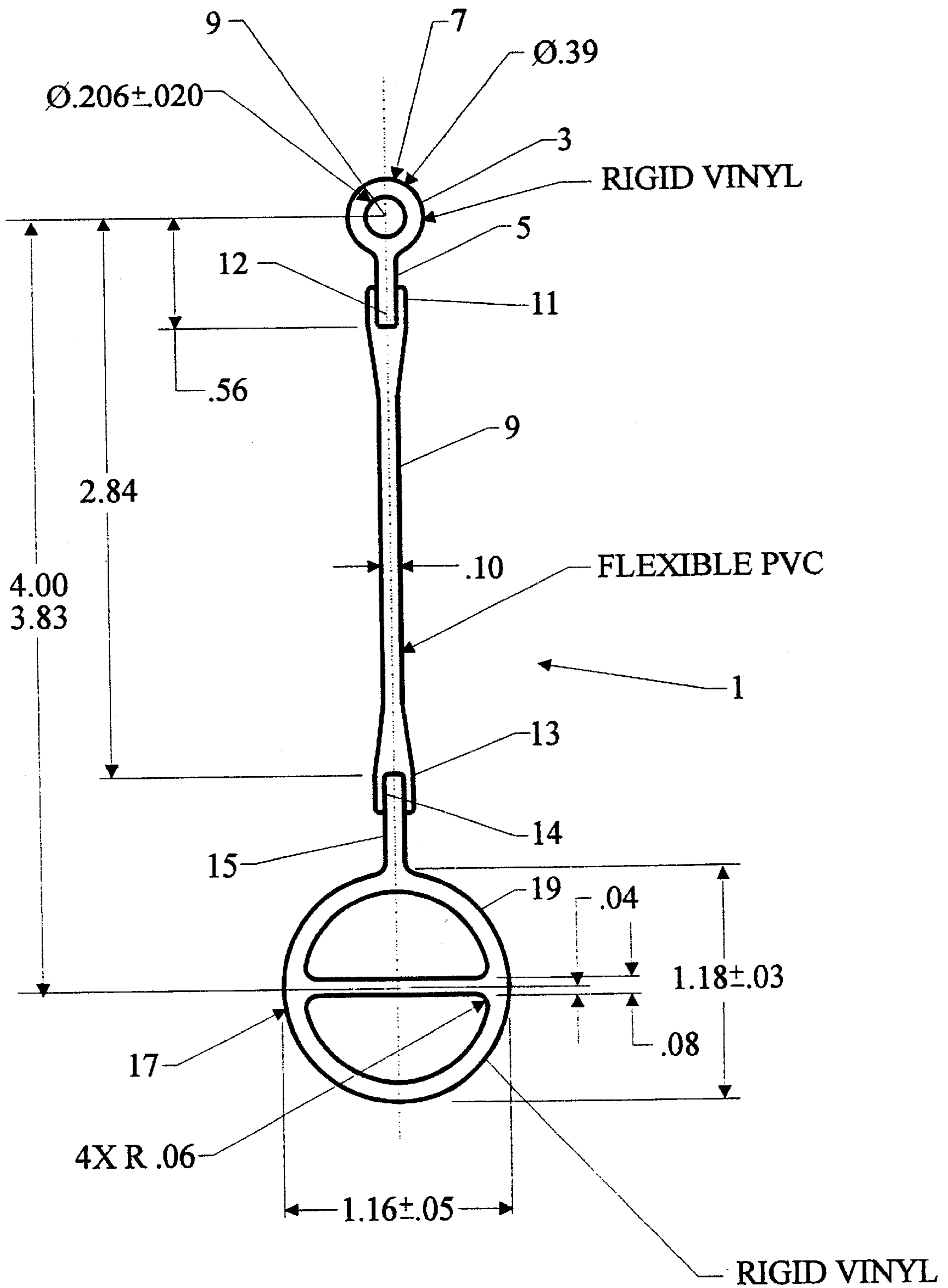
Figure 1 (PRIOR ART)
