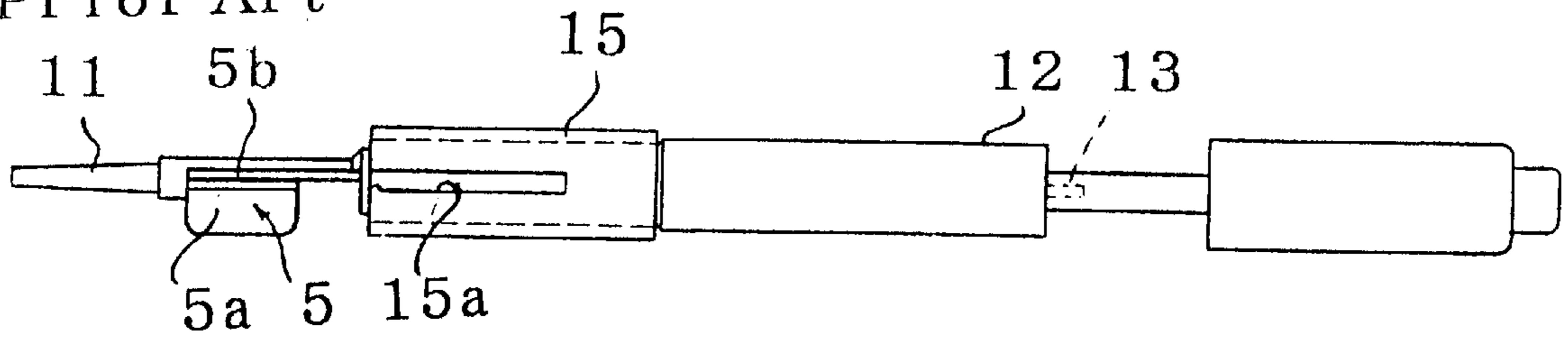
FIG. 26b Prior Art
