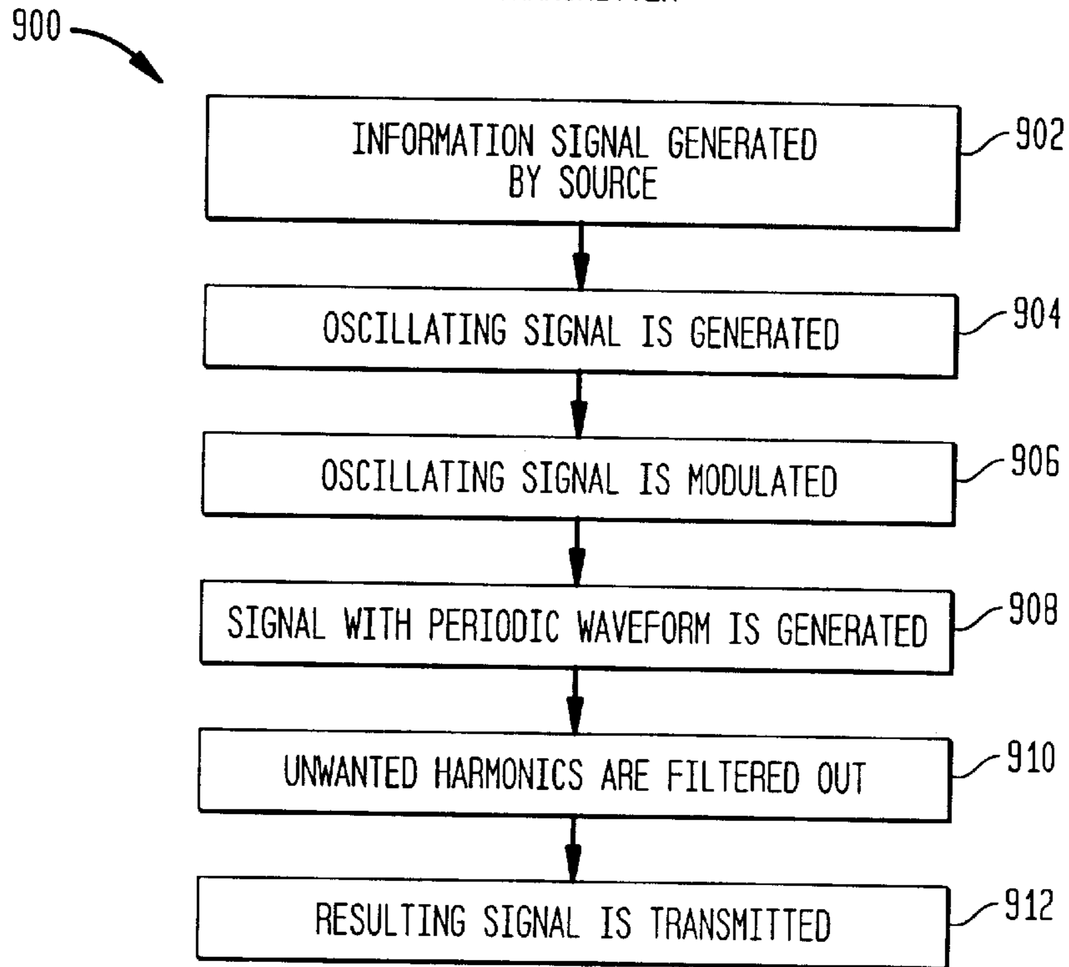
TRANSMITTER
