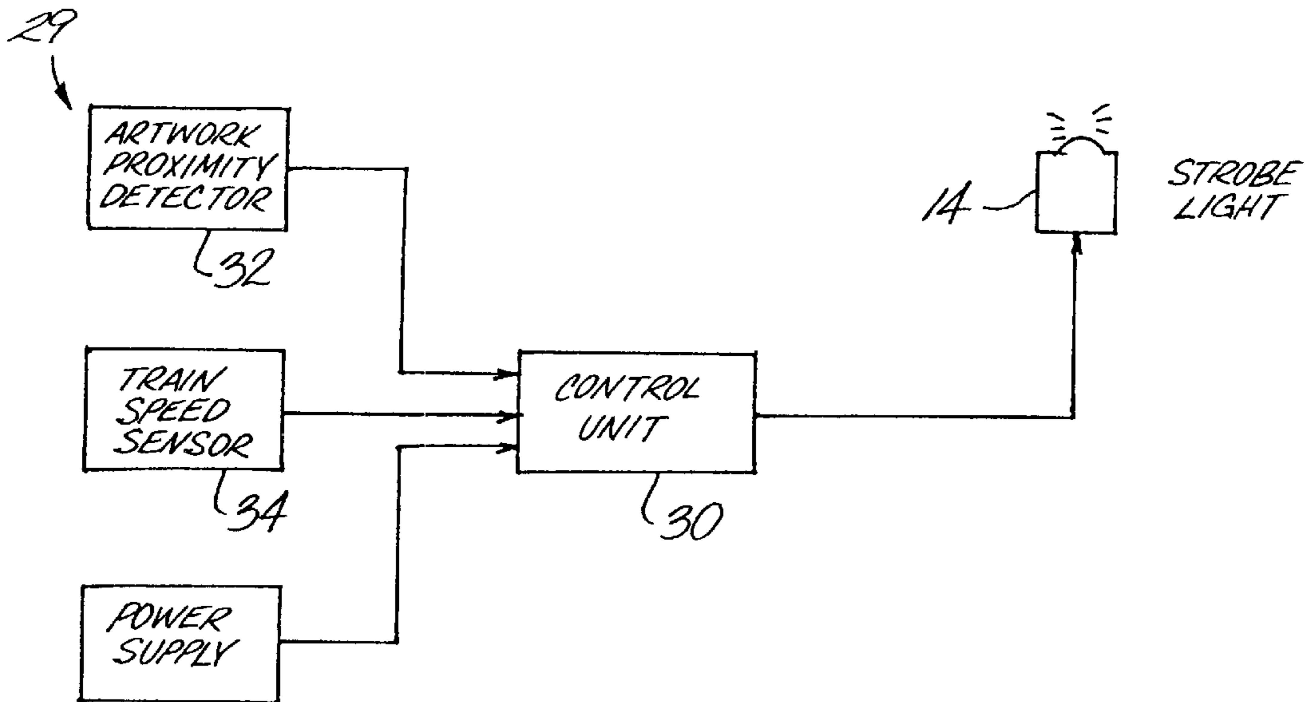
BLOCK DIAGRAM OF STROBE LIGHT CONTROL SYSTEM
