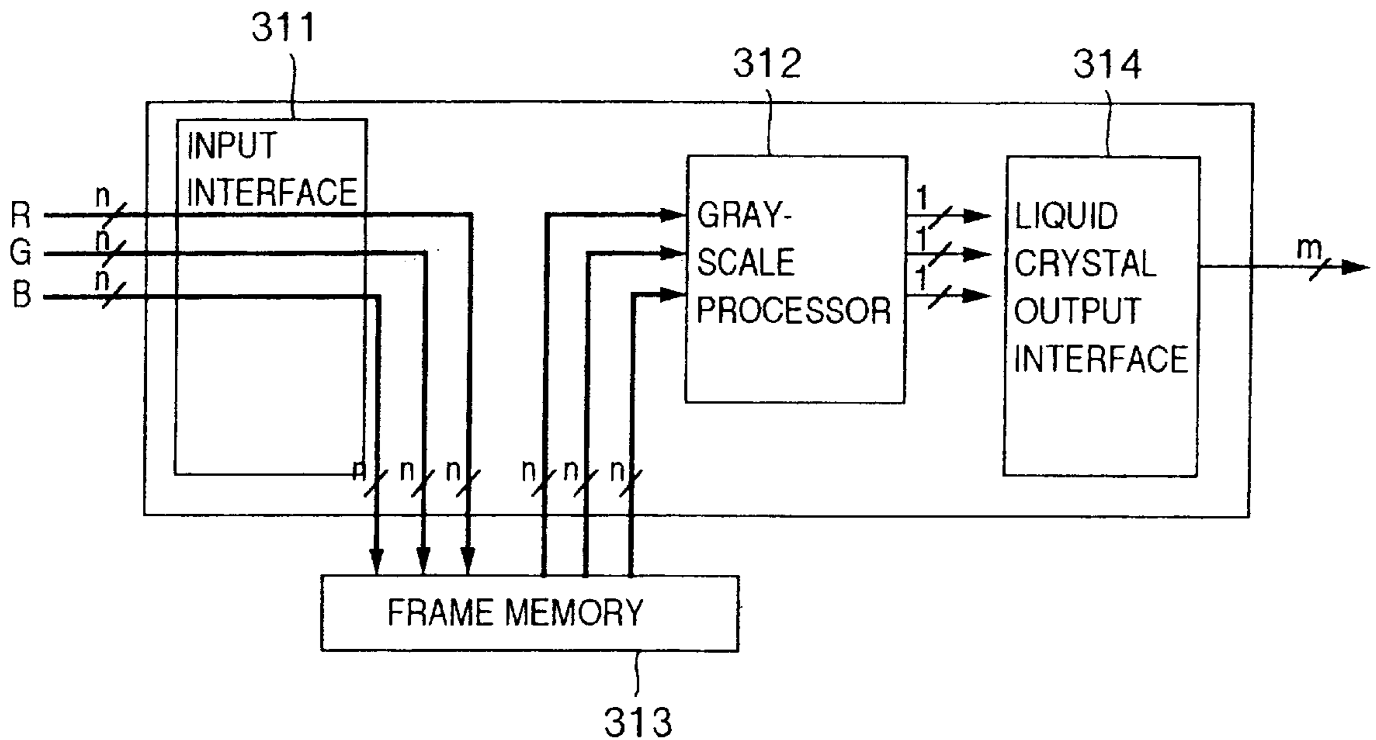
FIG.32 (PRIOR ART)
