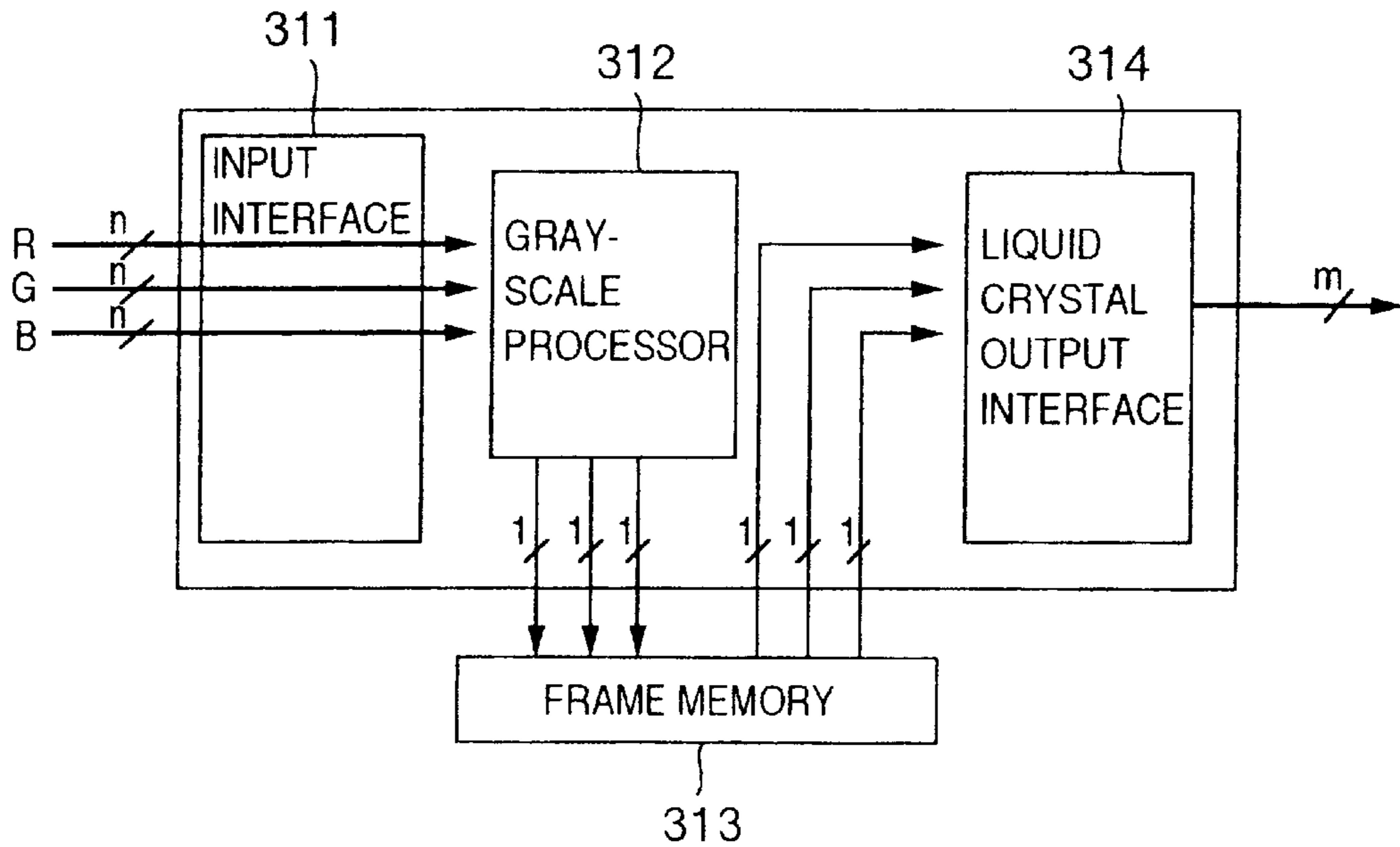
FIG.31 (PRIOR ART)
