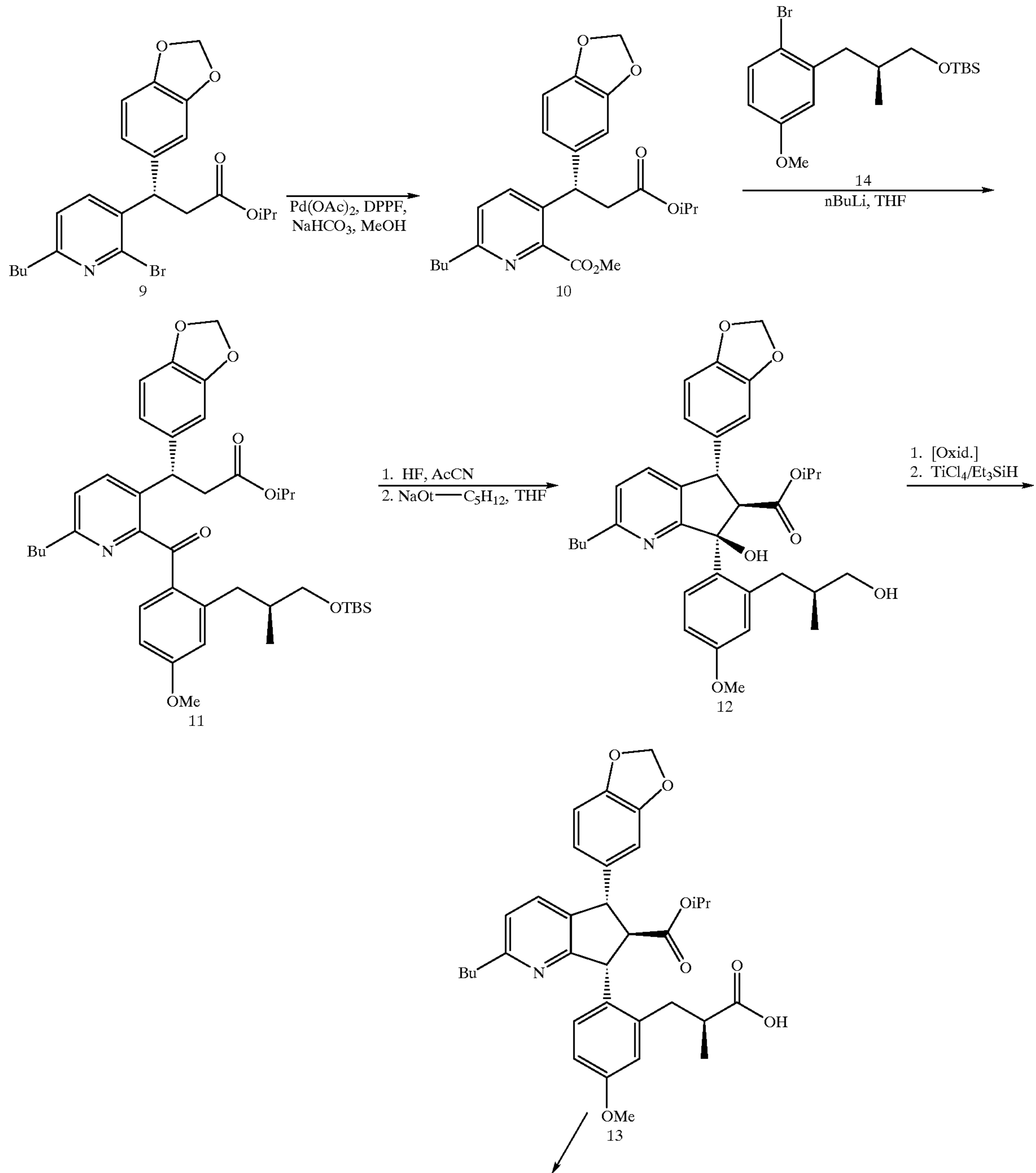
SCHEME 4
