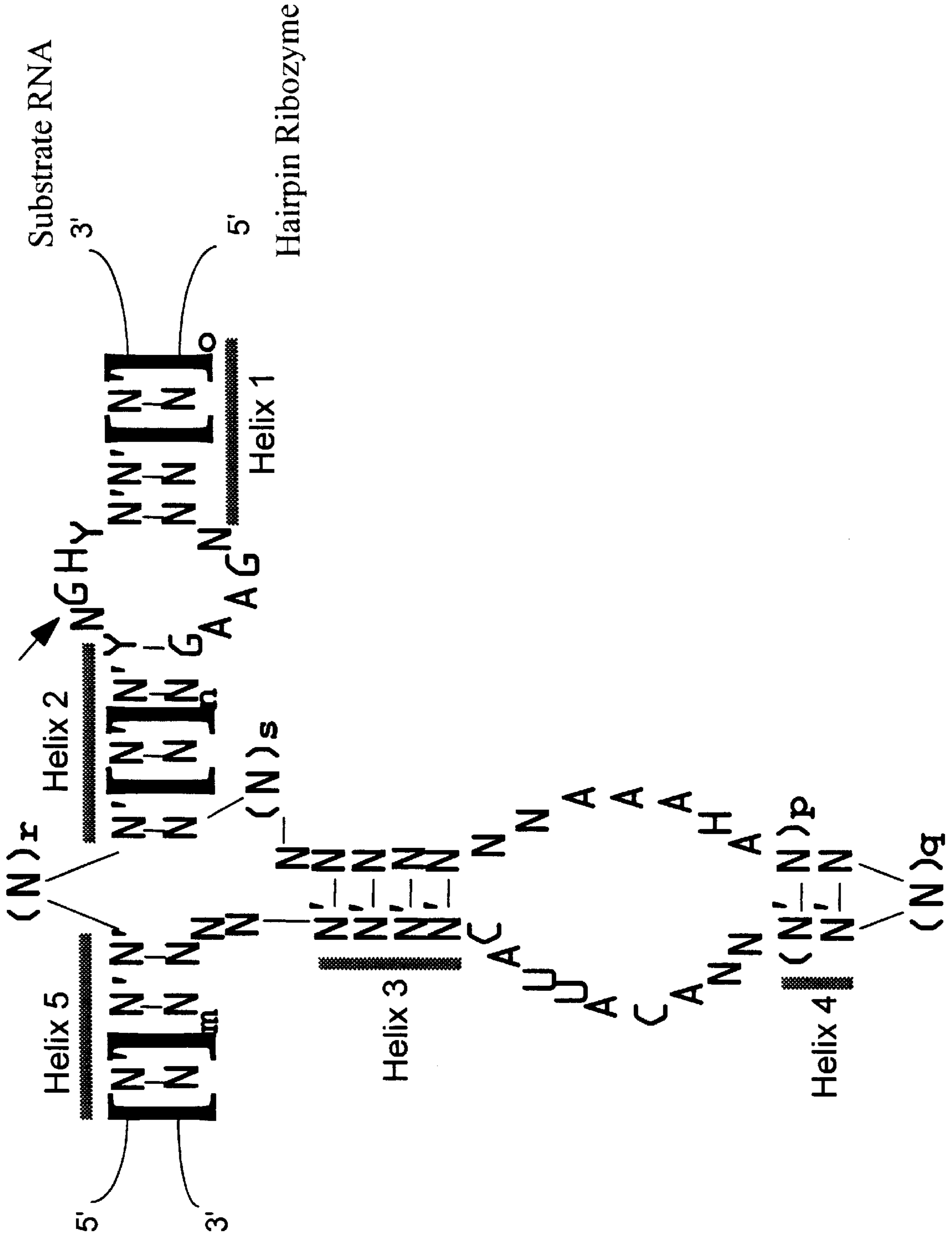
Figure 3: Hairpin Ribozyme
