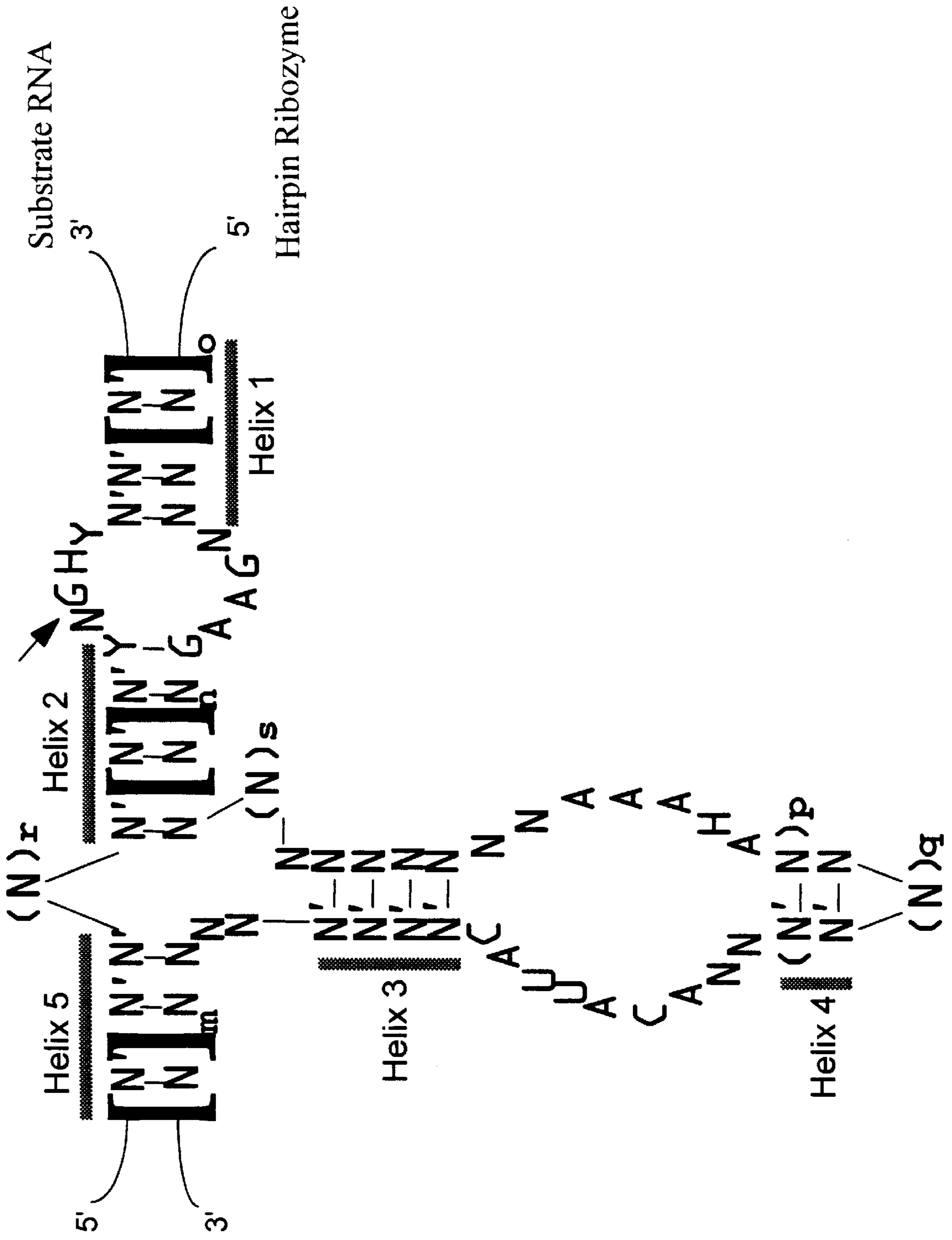
Figure 3: Hairpin Ribozyme
