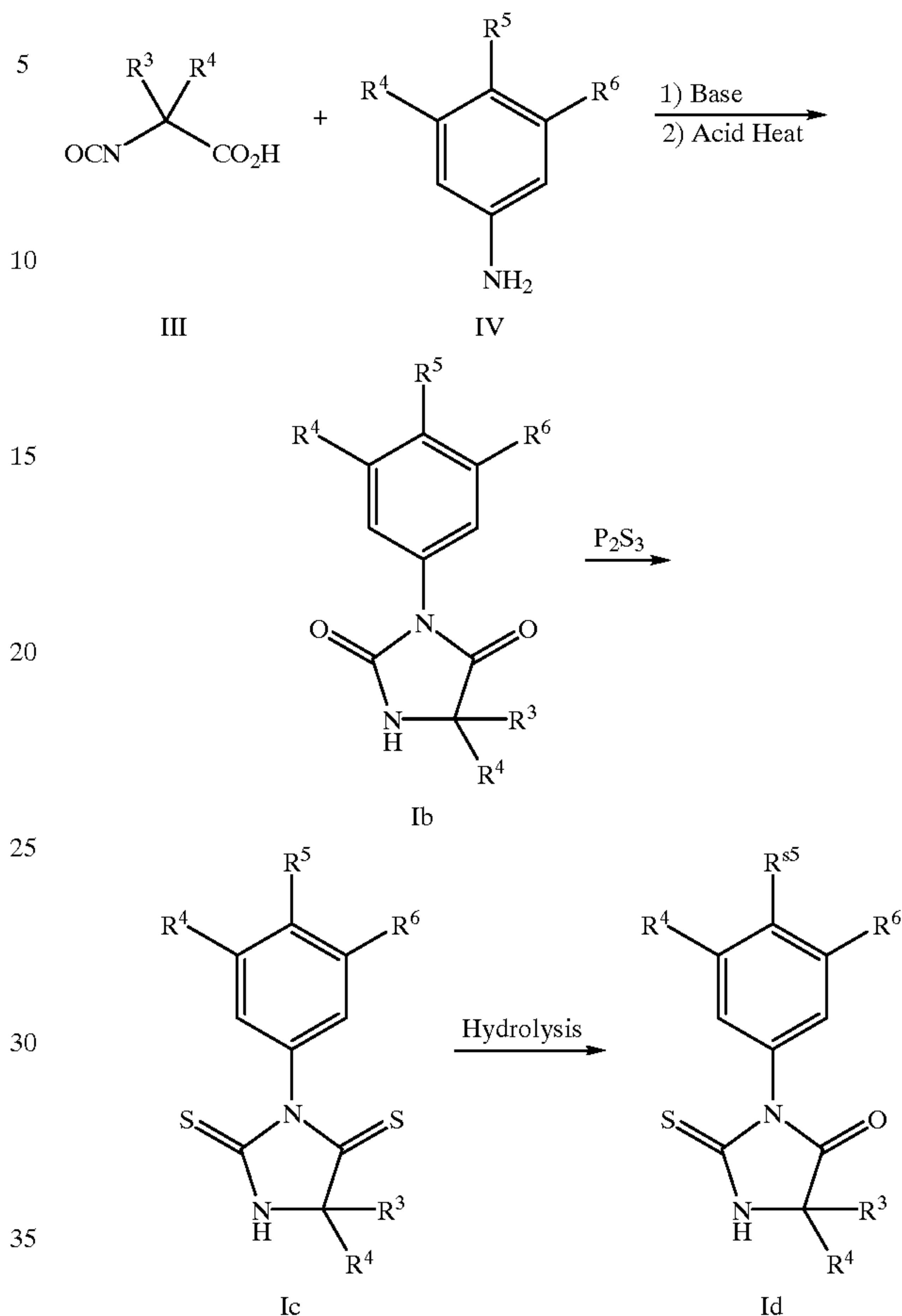
Scheme I
