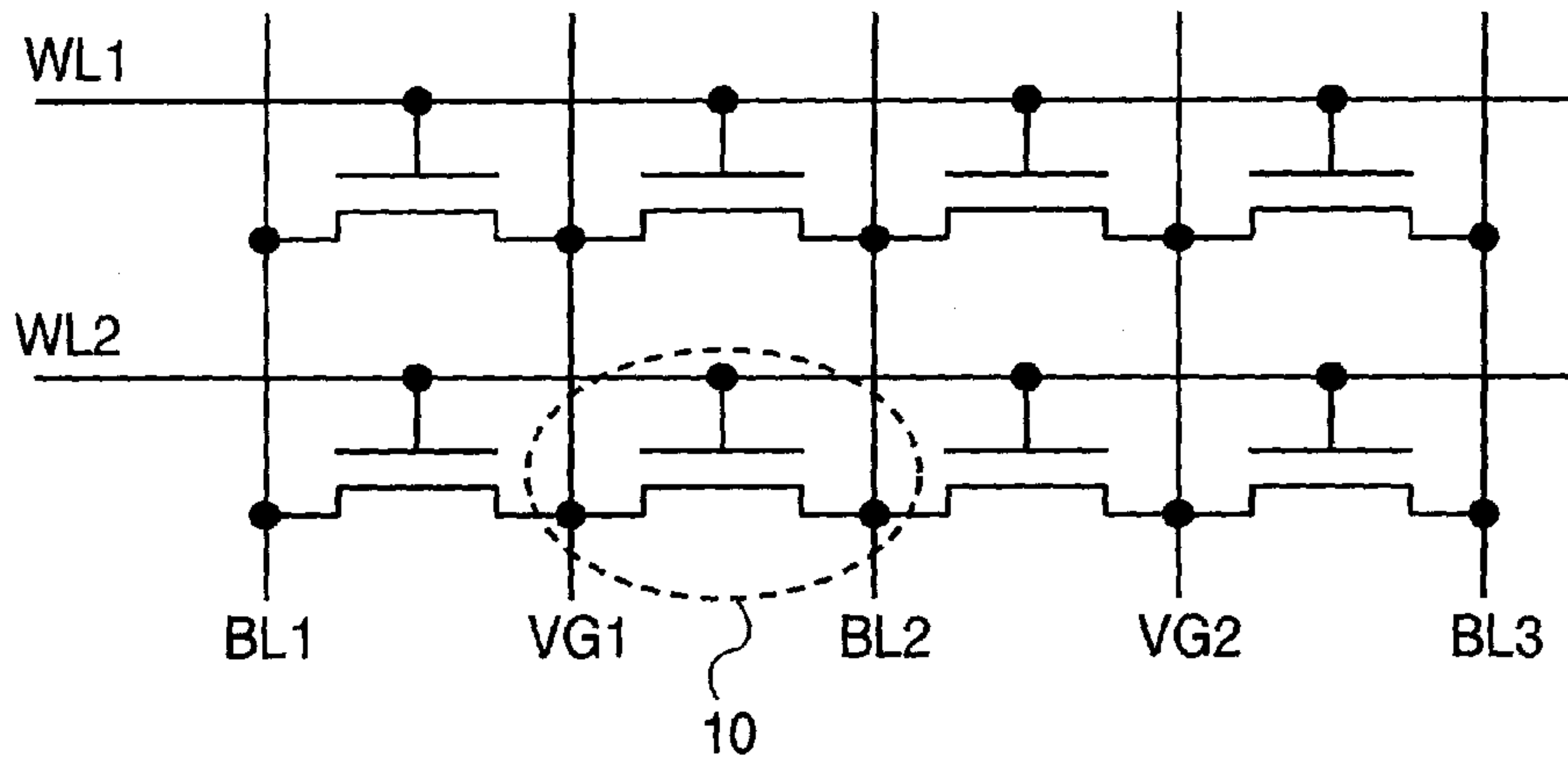
FIG. 1 (PRIOR ART)
