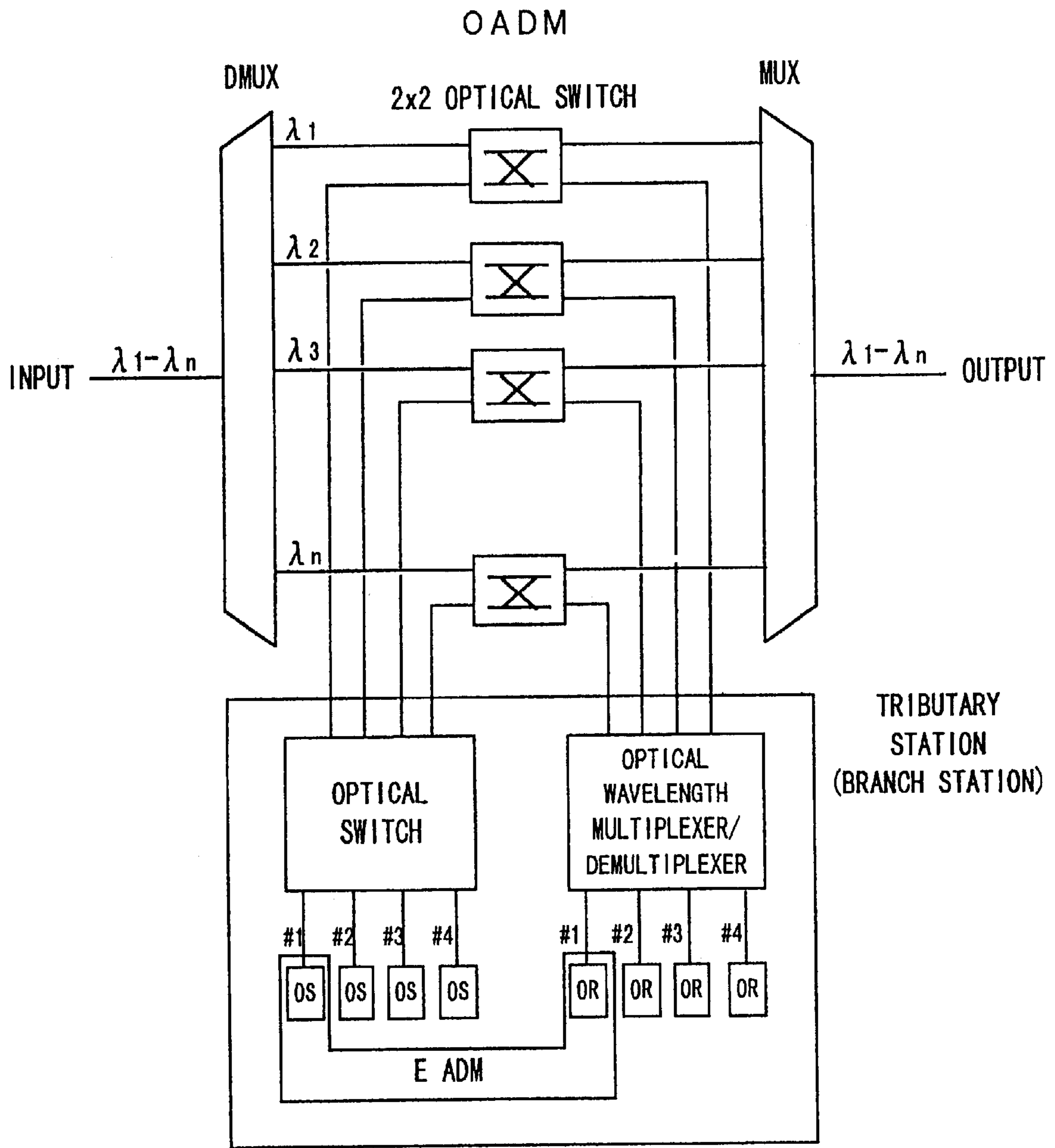
FIG. 1 (PRIOR ART)
