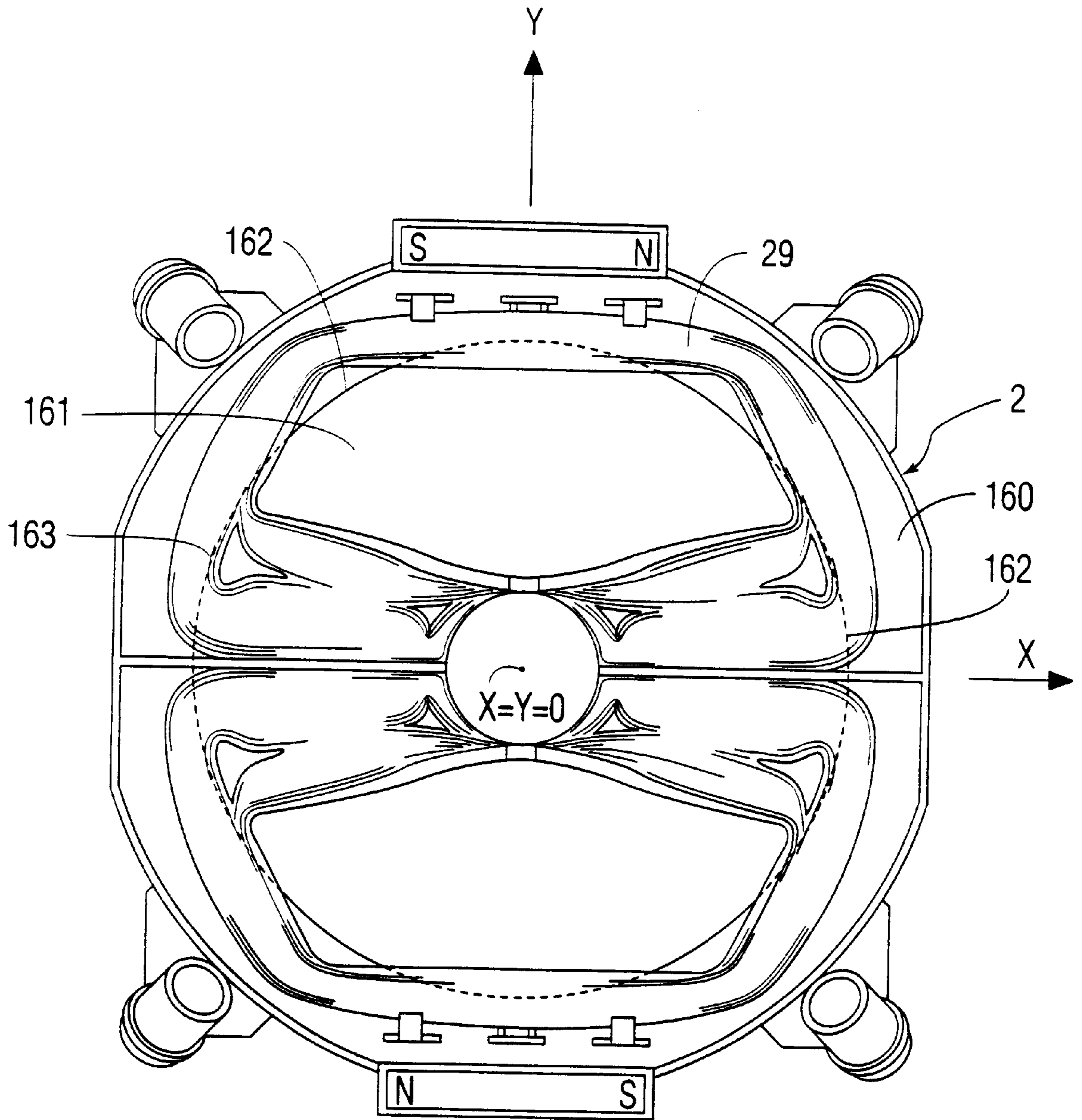
FIG. 2 PRIOR ART
