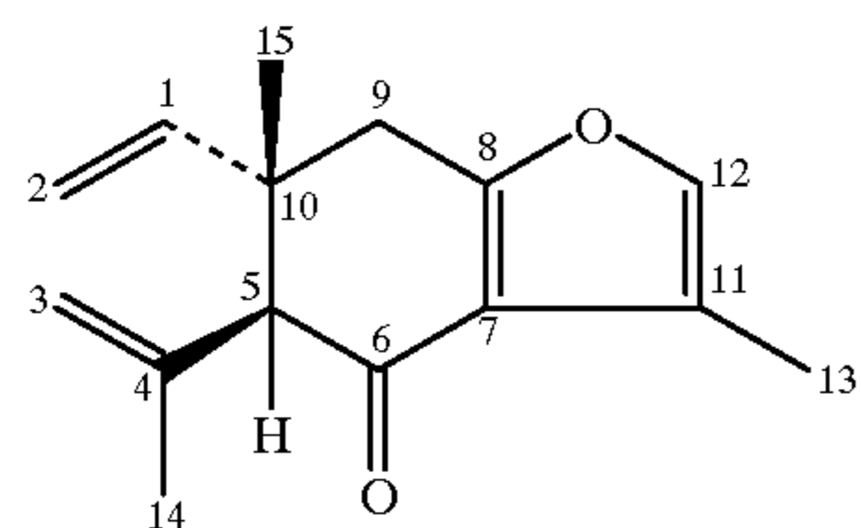
Curzersnona (Furanoeudesmans type)
