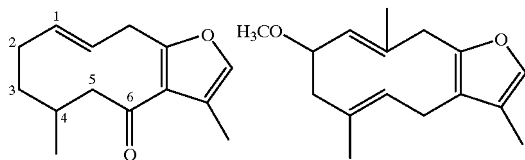
4,5-Dihydrofuranodian-8-one (Furenoelemens type)
