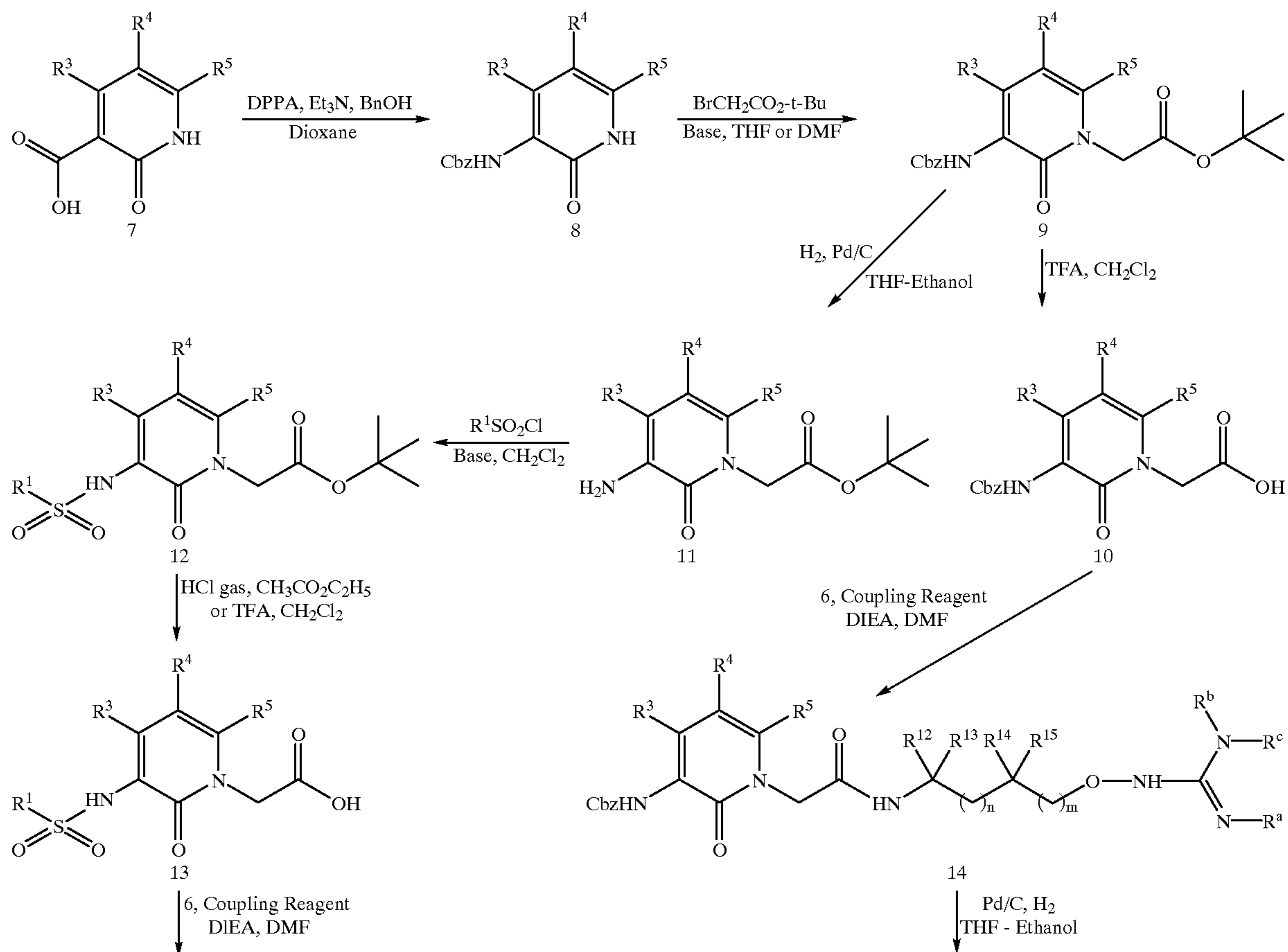
Scheme 2
