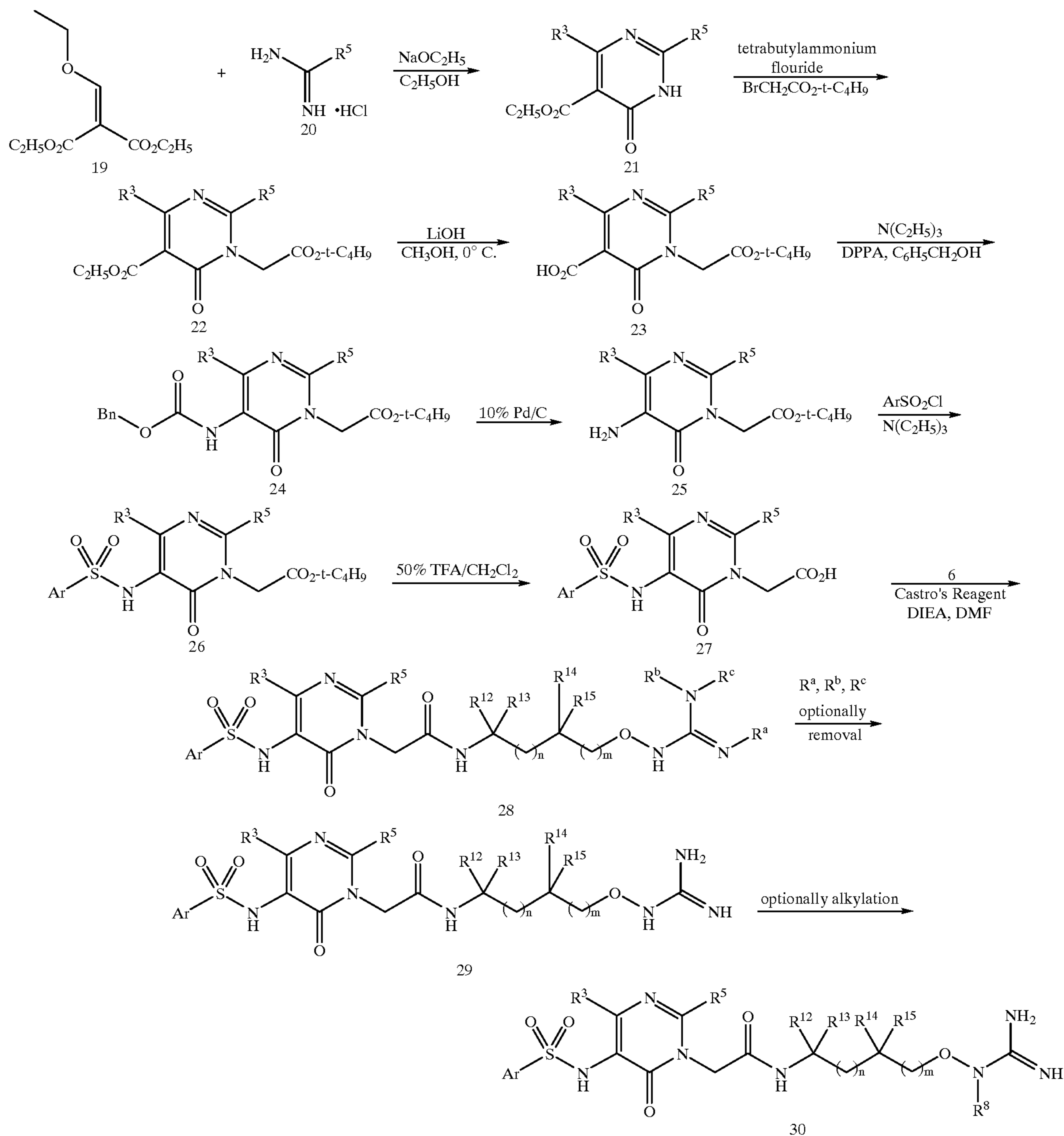
Scheme 3
