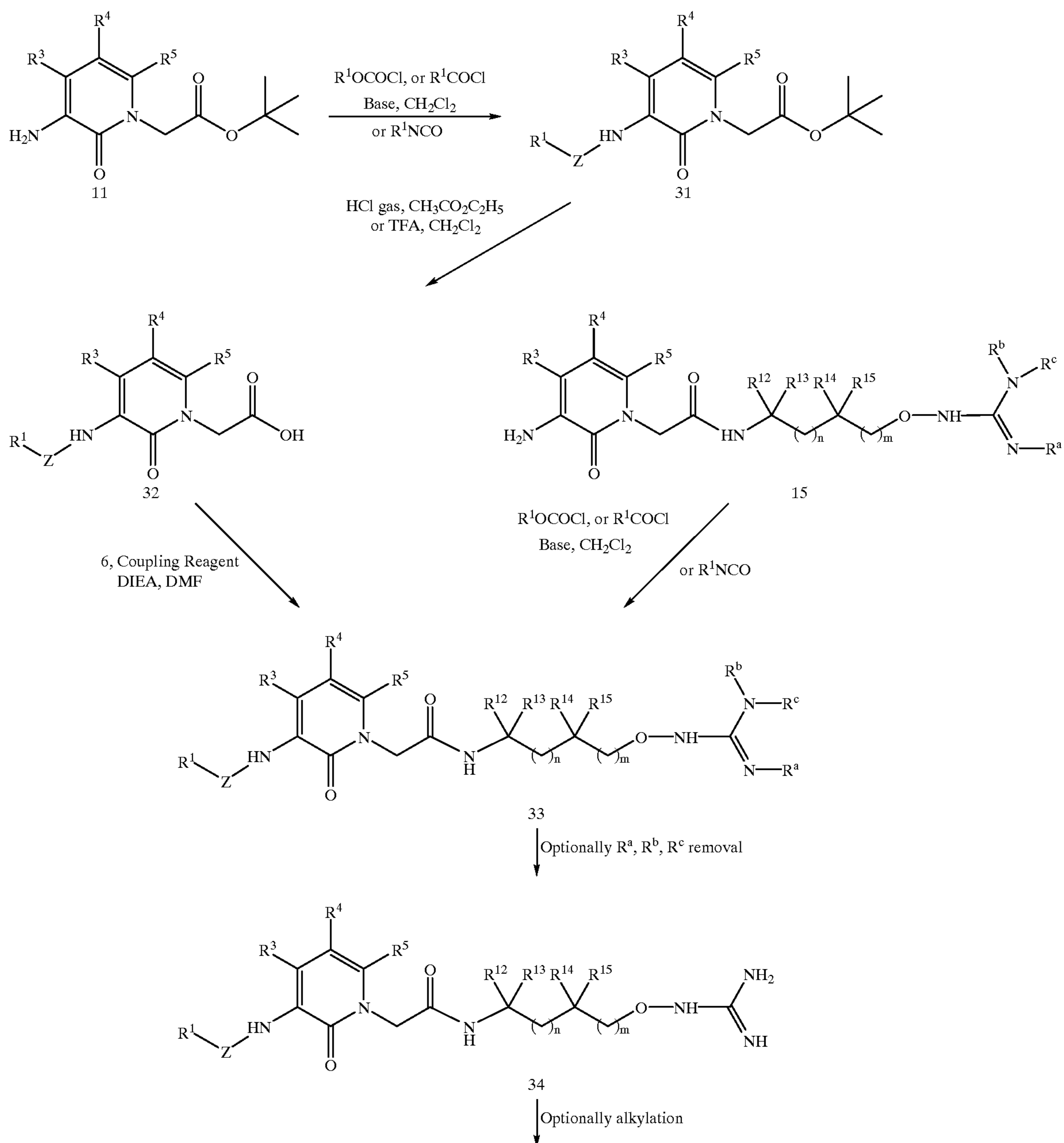
Scheme 4
