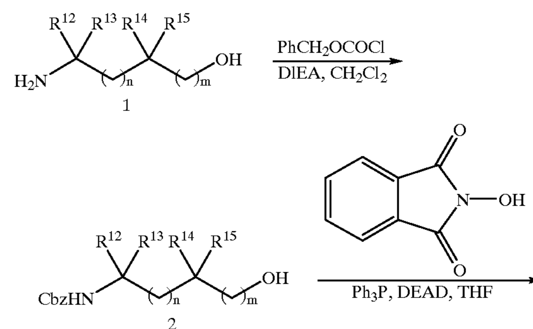
Scheme 1
