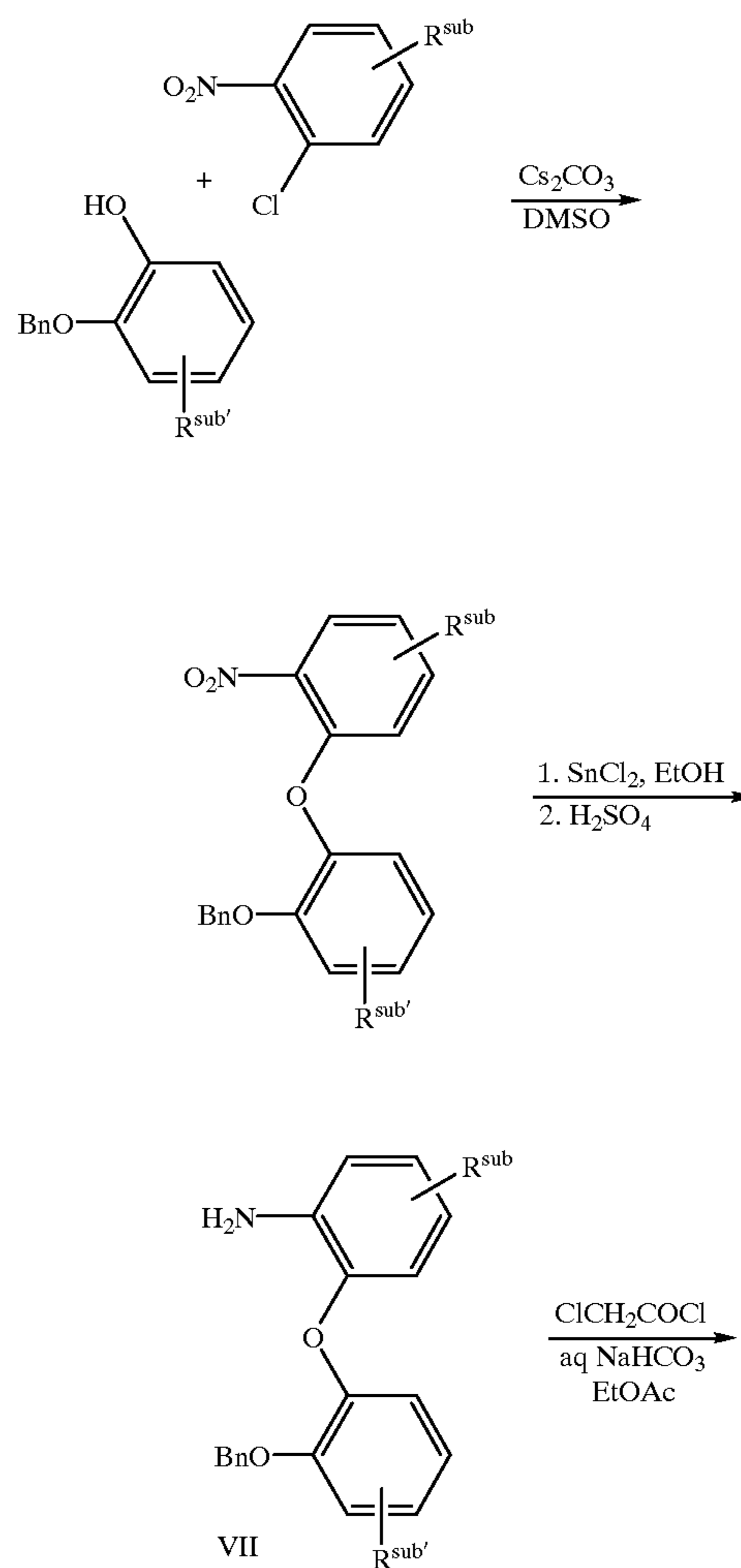
SCHEME 2
