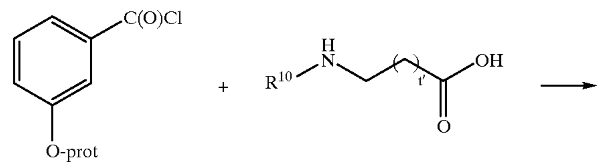
SCHEME 5
