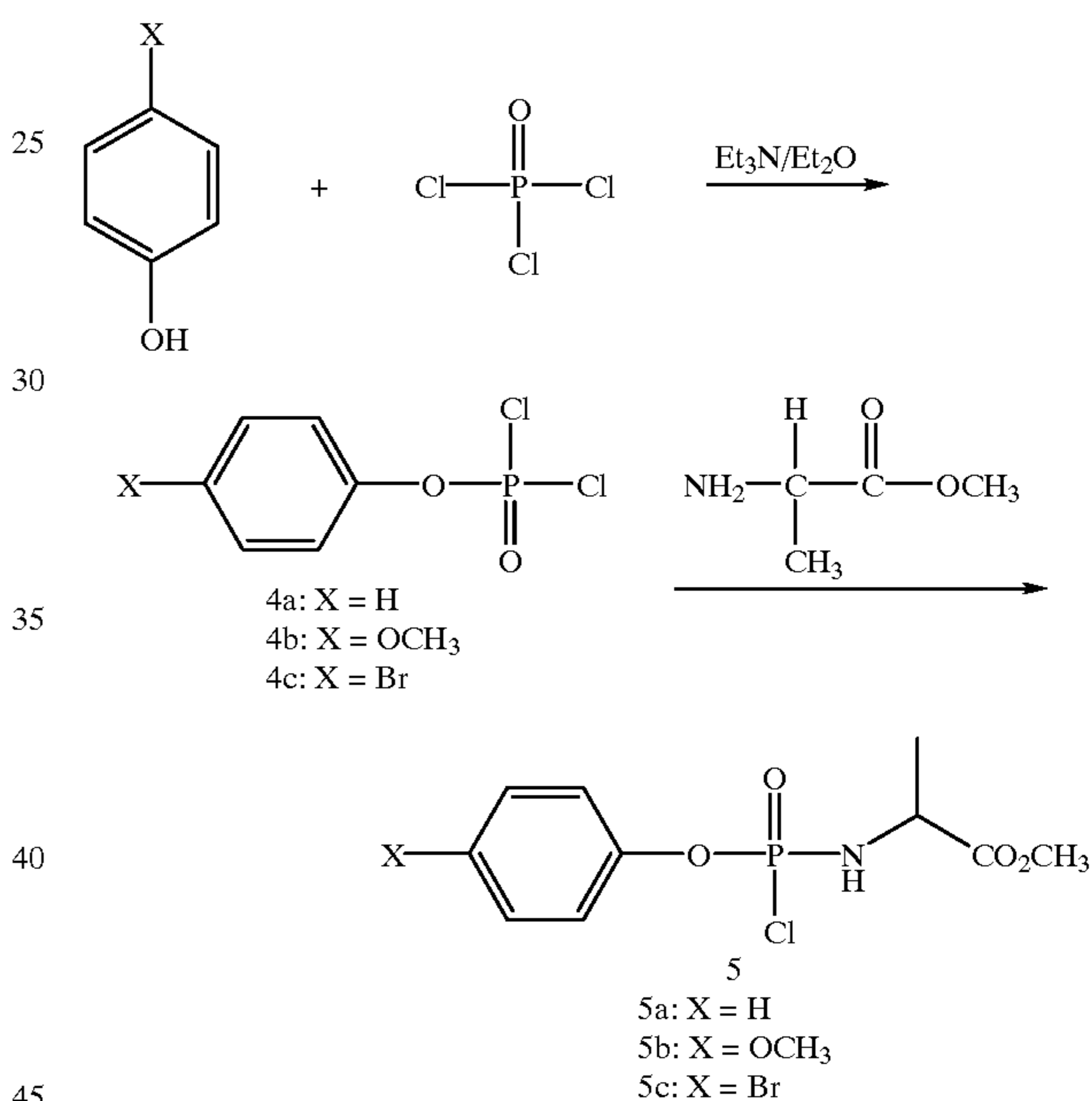
Scheme 2 Synthesis of phenyl methoxyalaninyl phosphorochloridates
