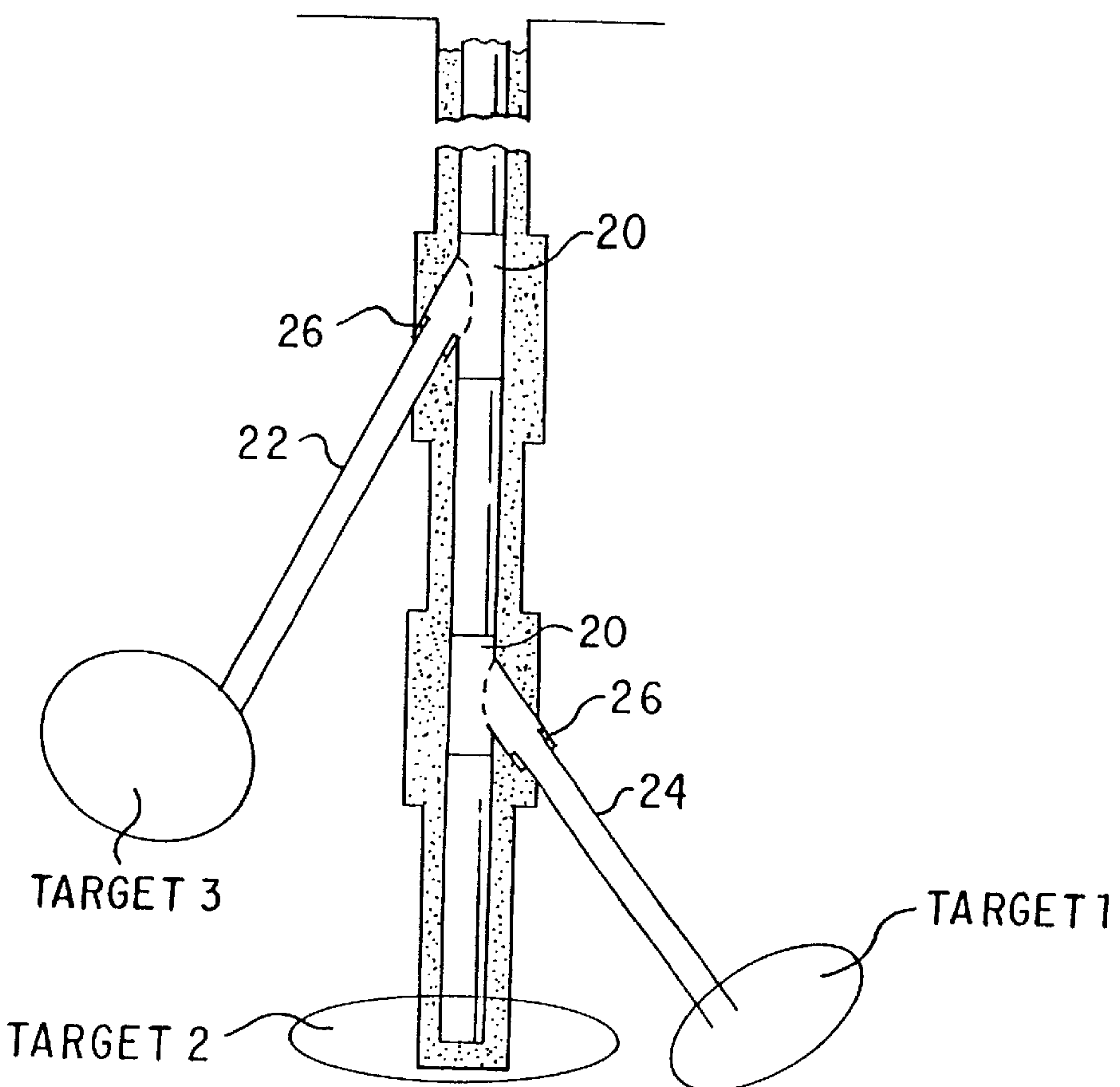
FIG. 2 PRIOR ART
