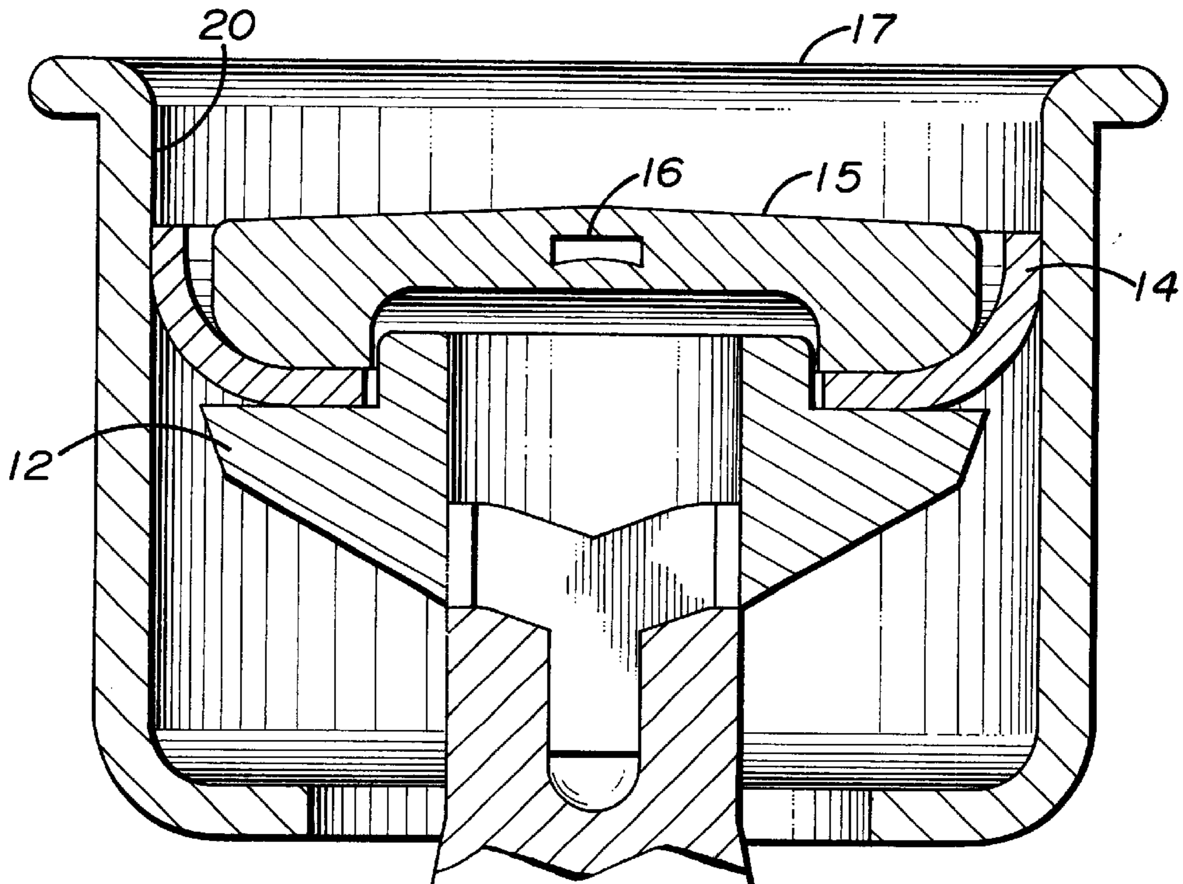
FIG. 1 (PRIOR ART)
