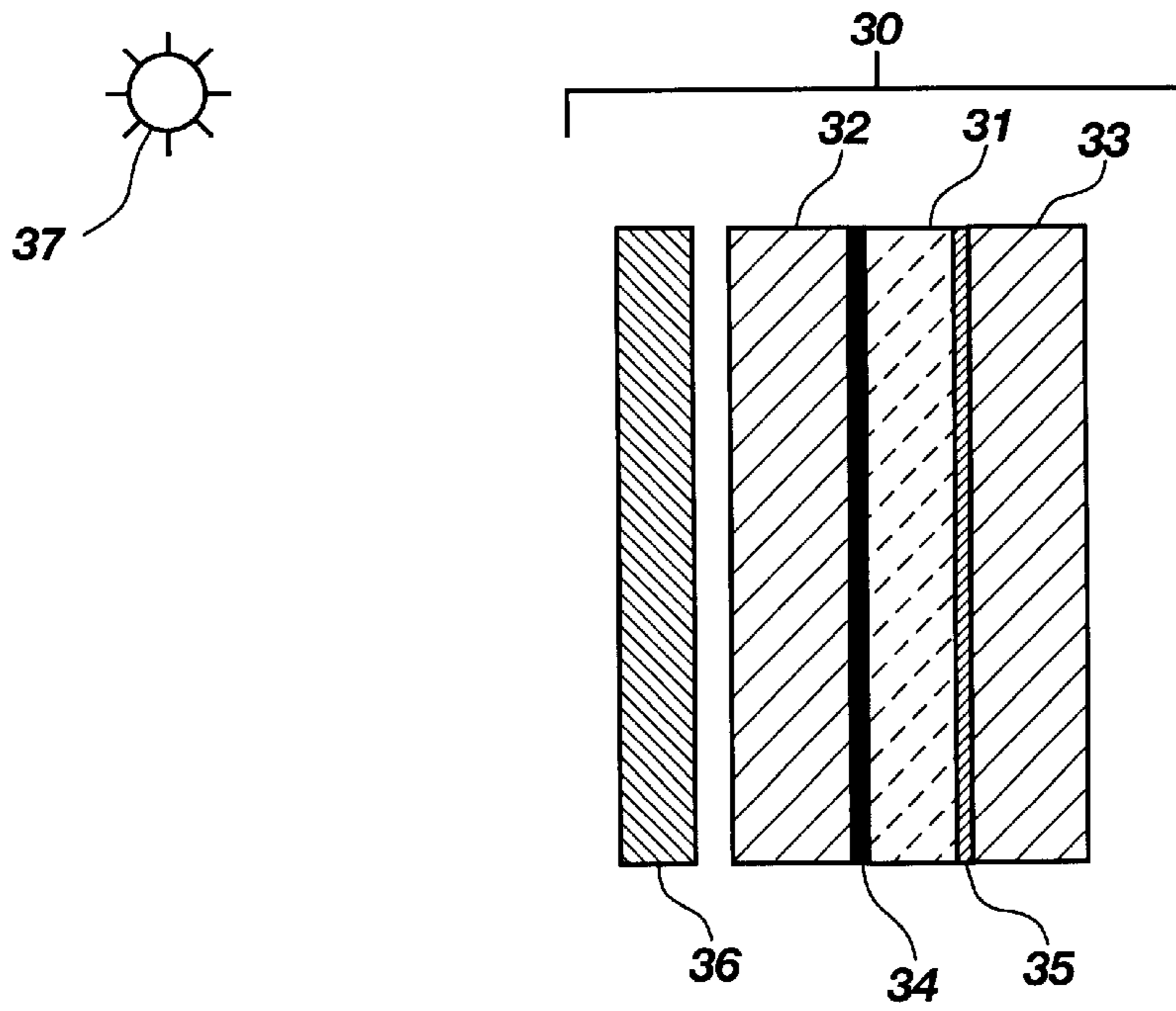
Fig. 3 (PRIOR ART)
