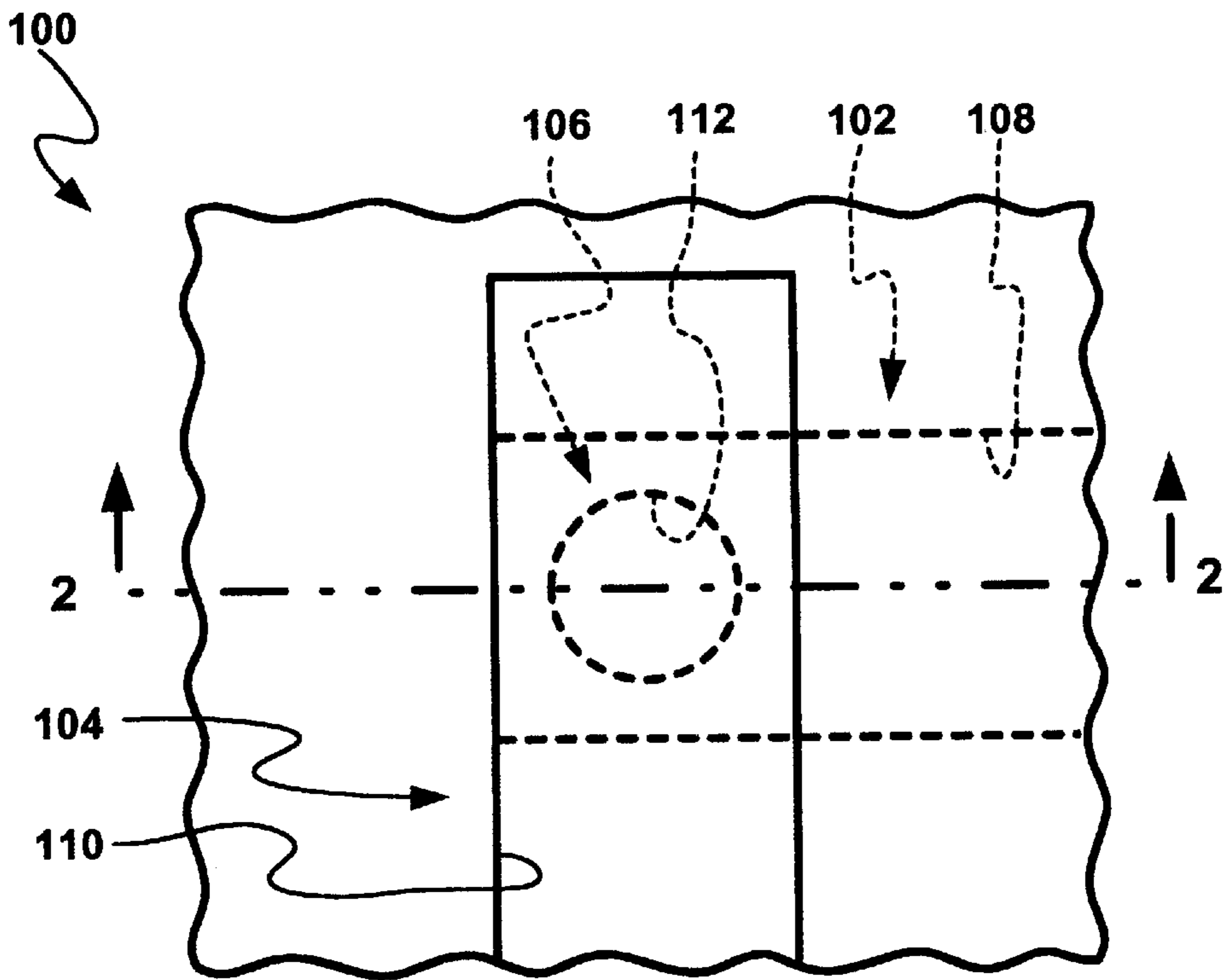
FIG. 1 (PRIOR ART)
