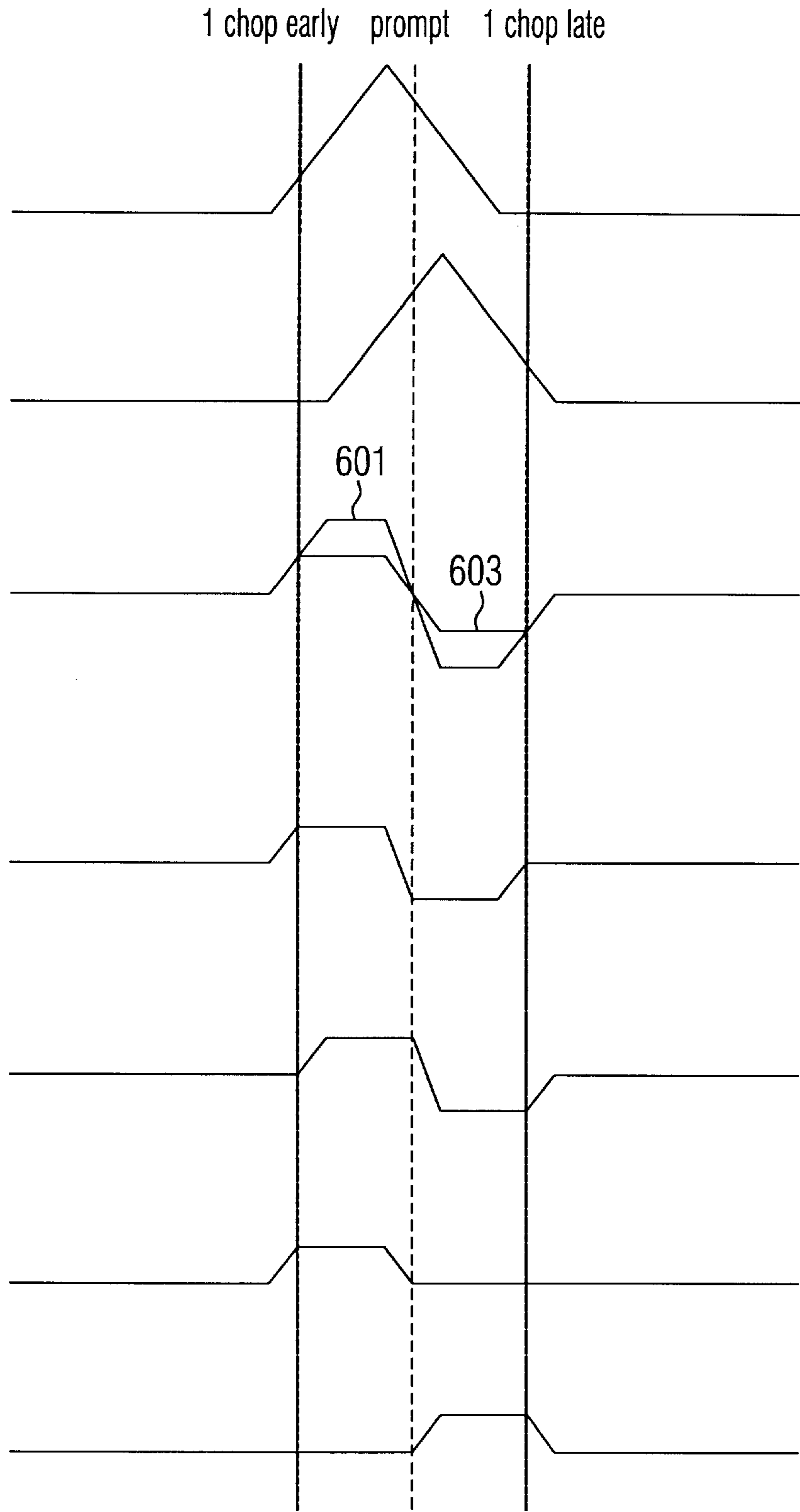
FIG. 6C 1/4 early - 1/2 late correlator
