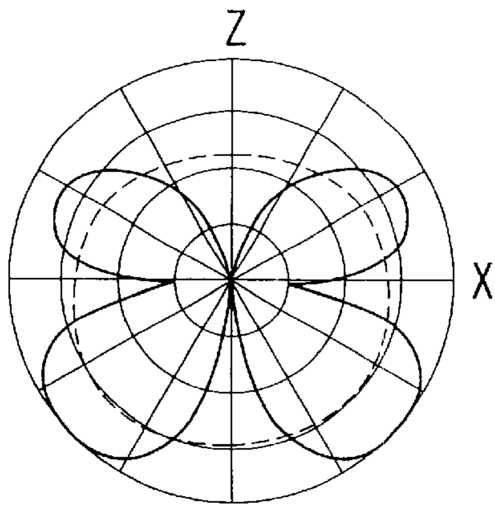
FIG. 7A 5 [dB/div] PRIOR ART — V POLARIZED WAVE --- H POLARIZED WAVE
