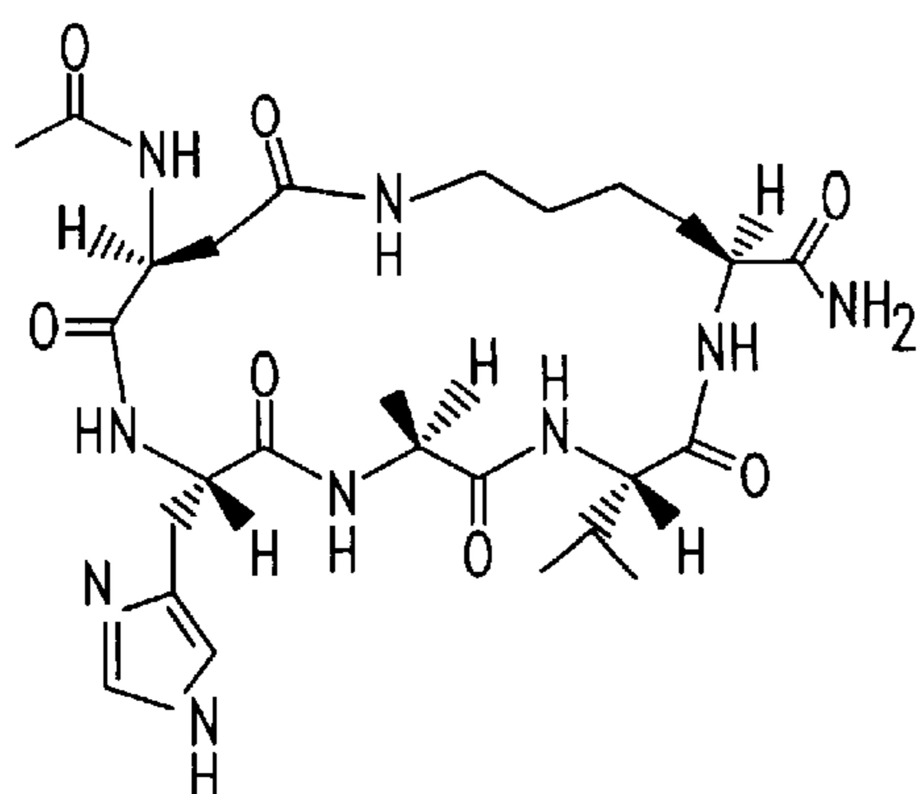
N-Ac-DHAVK-NH 2
