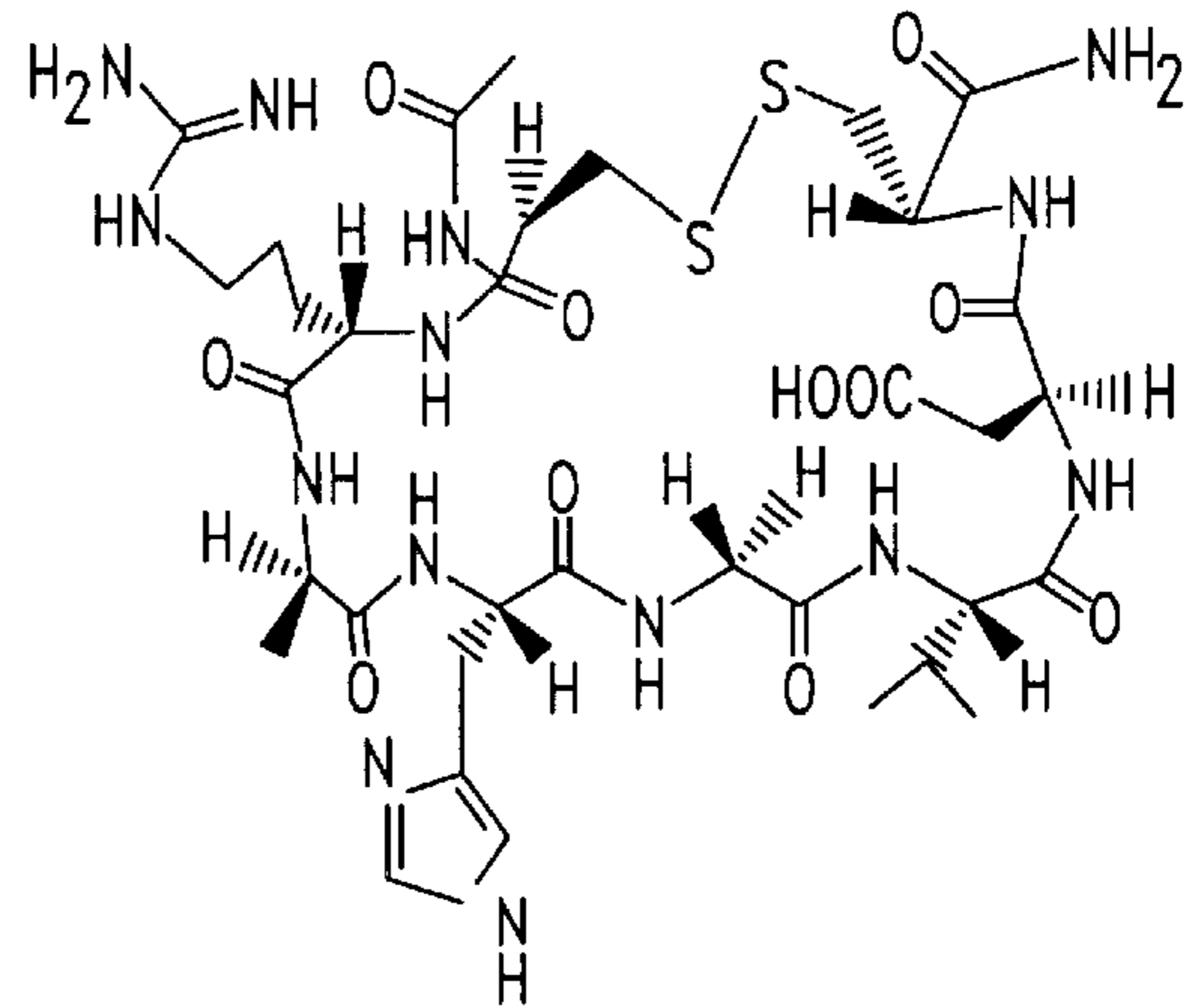
N-Ac-CRAHGVDC-NH 2
