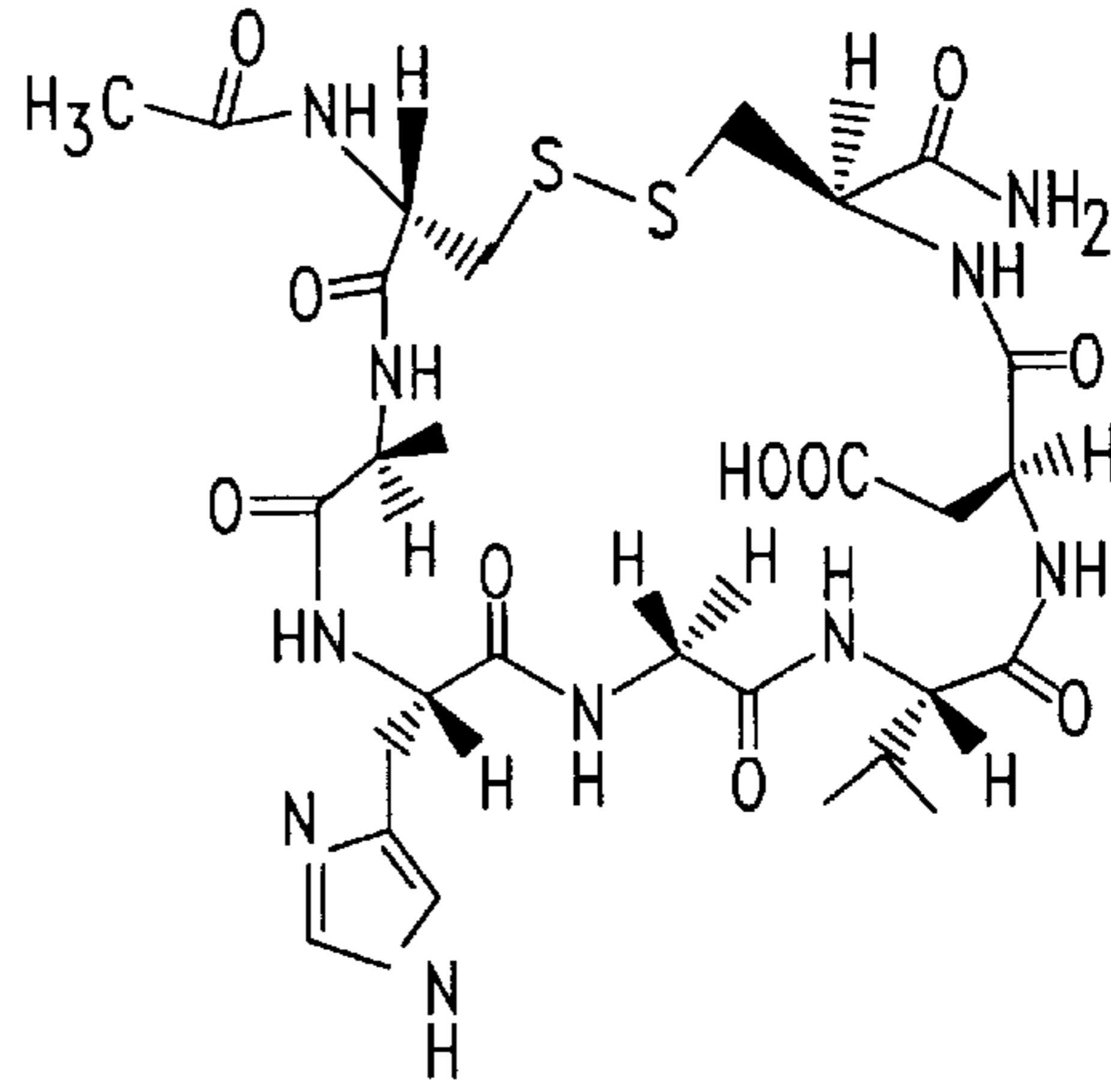
N-Ac-CAHGVDC-NH 2
