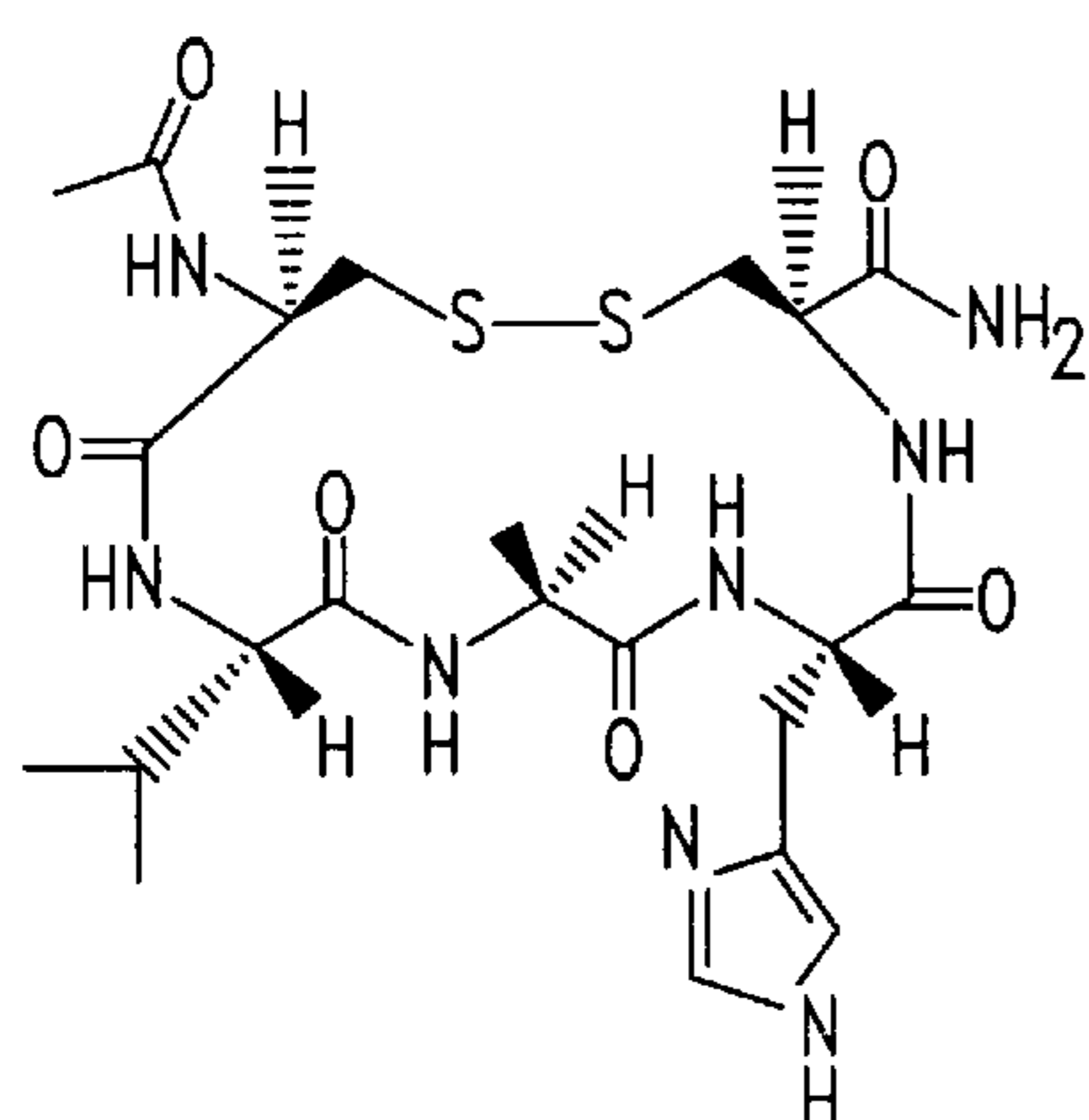
N-Ac-CVAHC-NH 2
