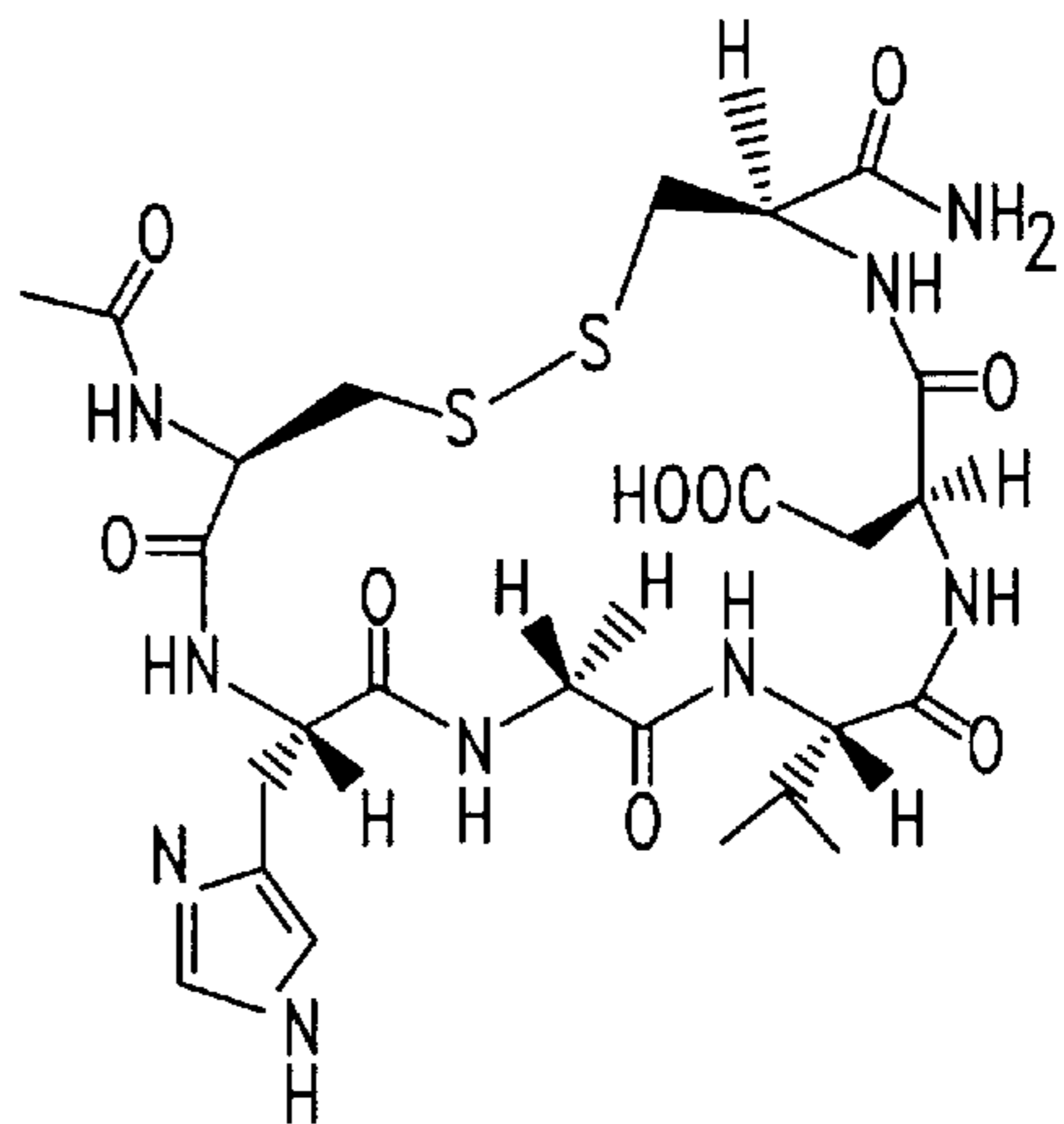
N-Ac-CHGVDC-NH 2
