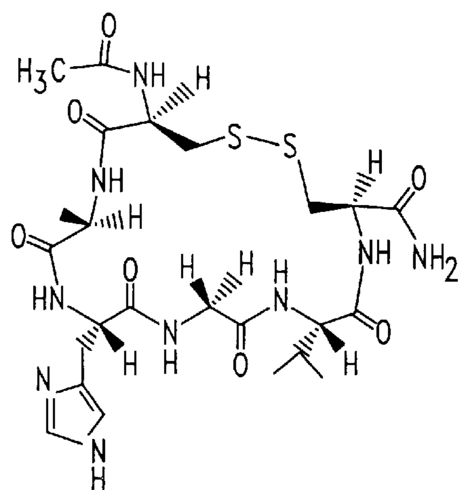
N-Ac-CAHGVNC-NH 2
