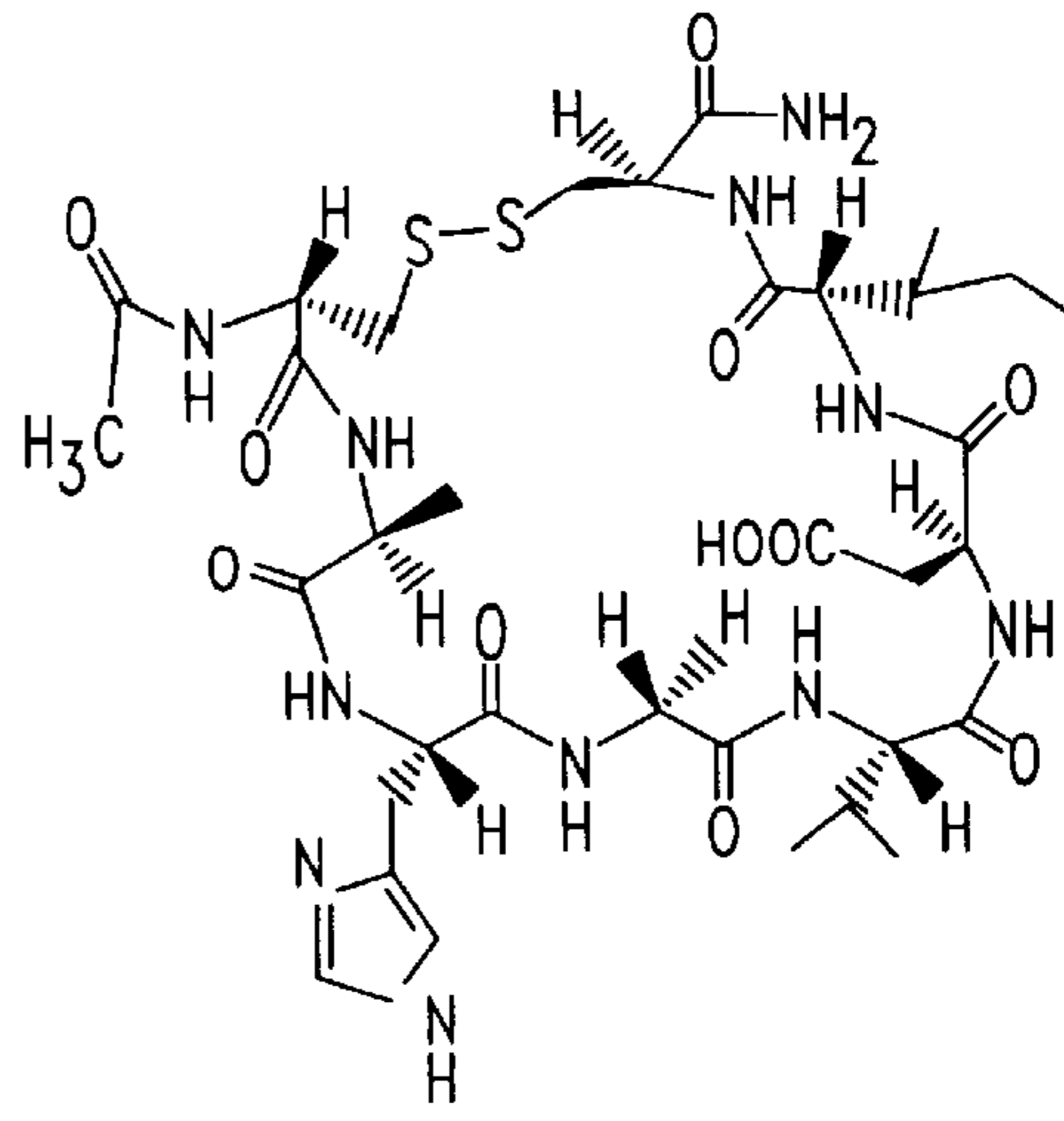
N-Ac-CAHGVDC-NH 2
