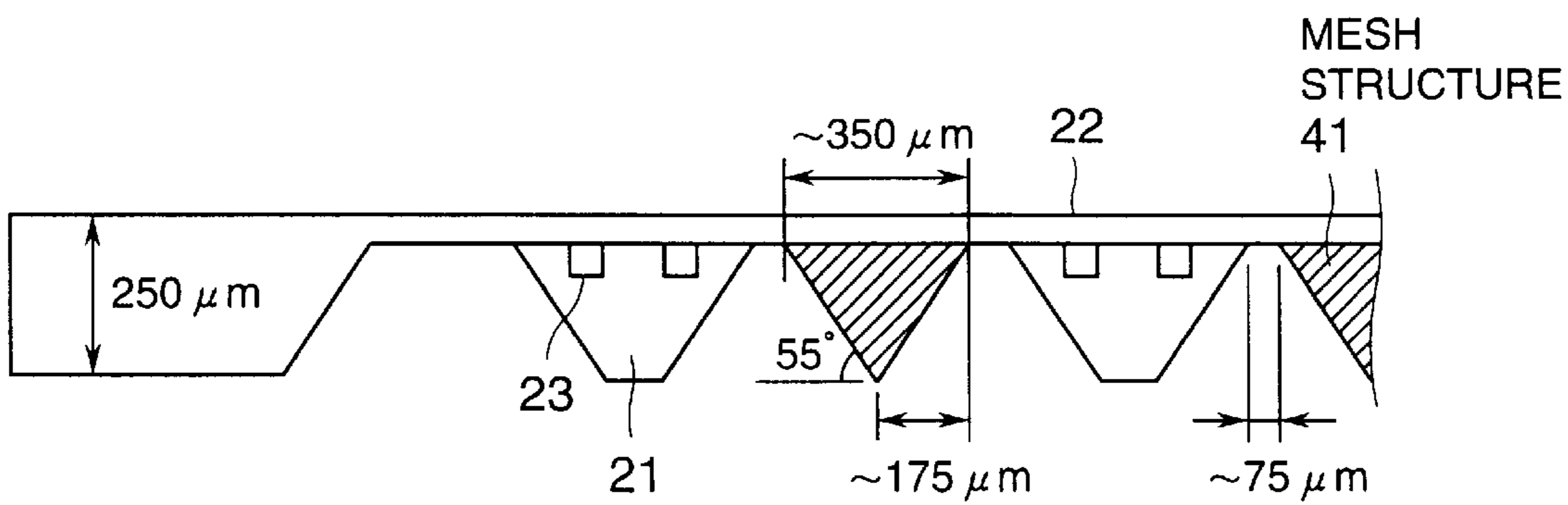
A CROSS SECTION VIEW AT B-B'
