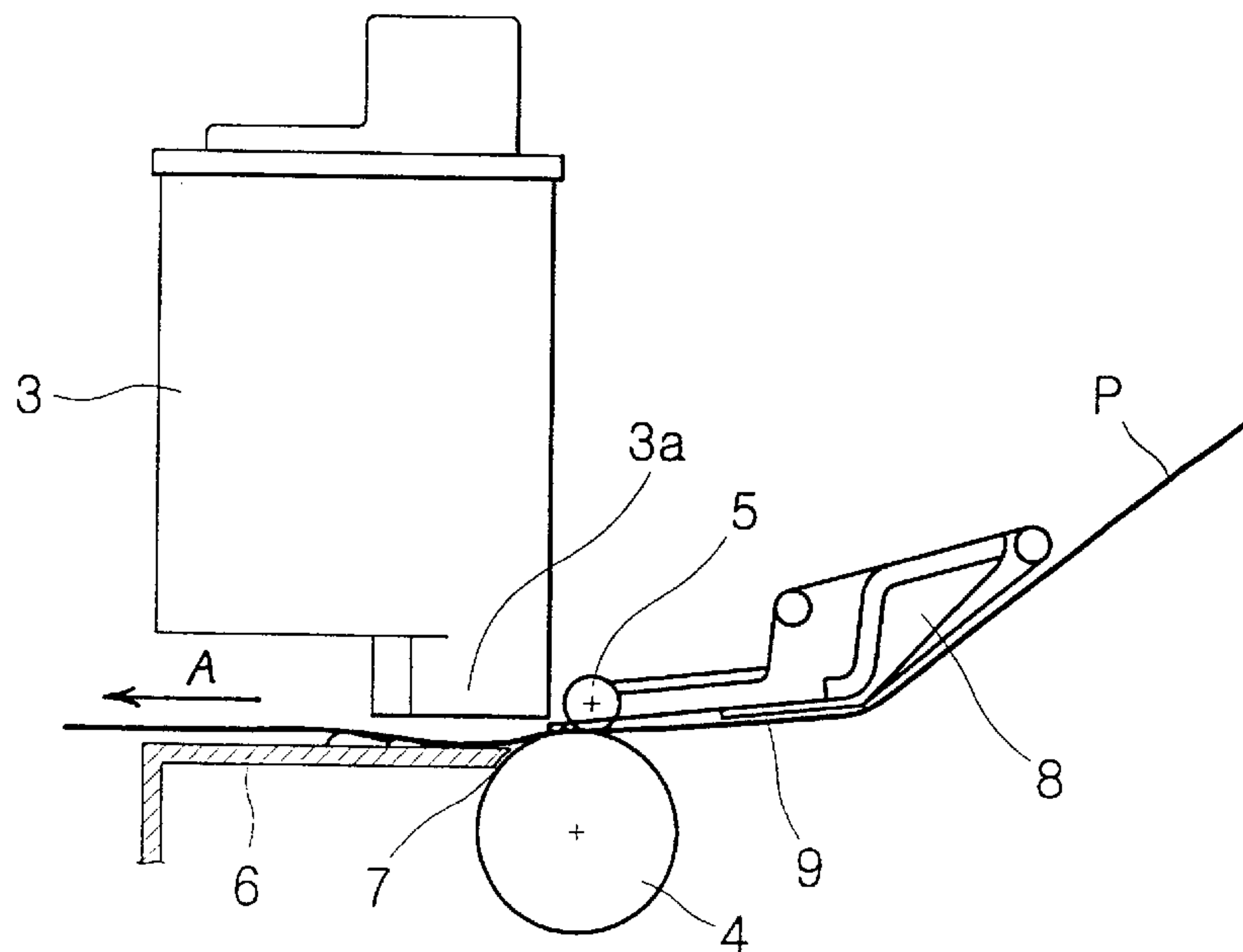
Fig. 2 (Prior Art)
