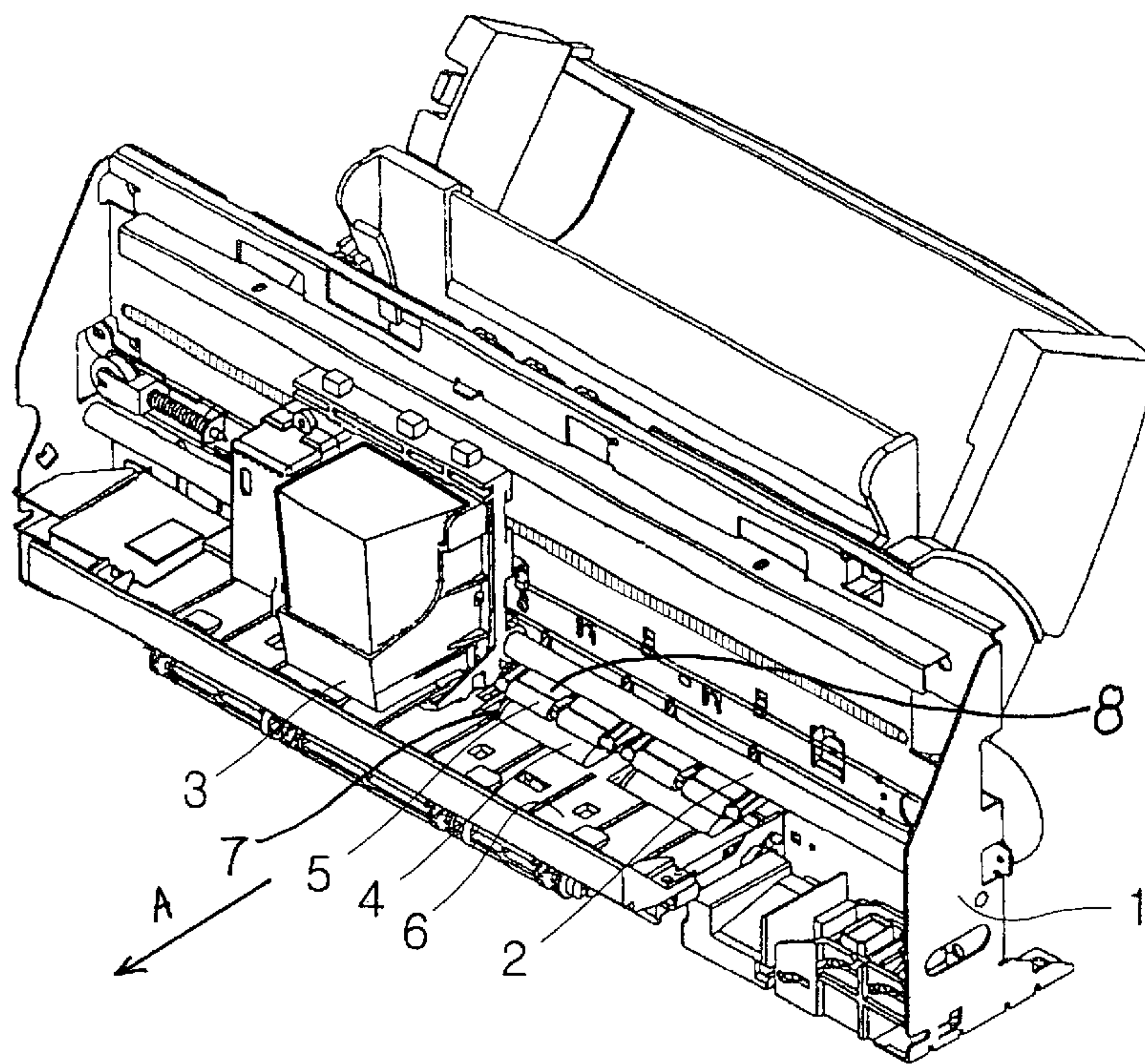
Fig. 1 (Prior Art)
