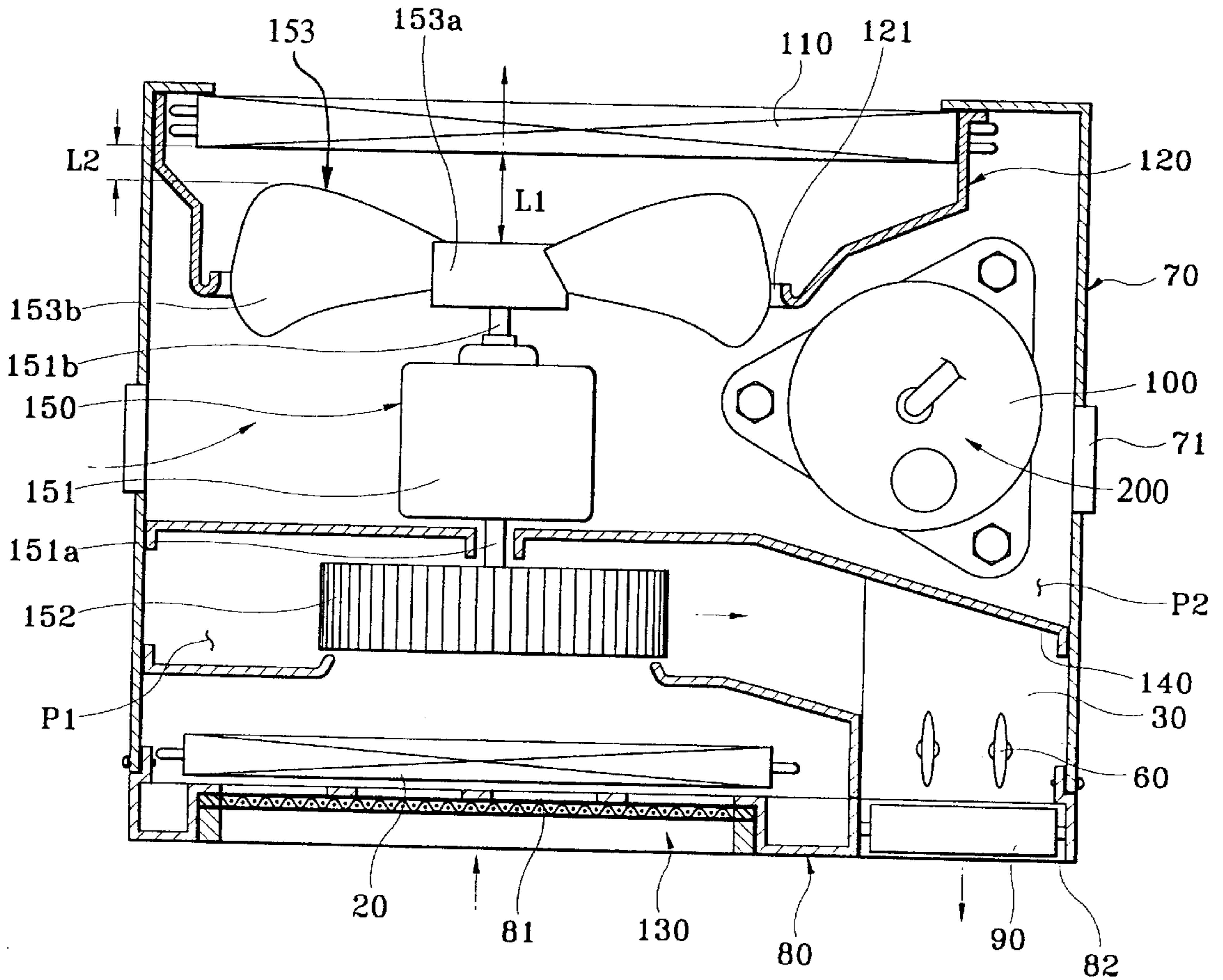
FIG. 2 (PRIOR ART)
