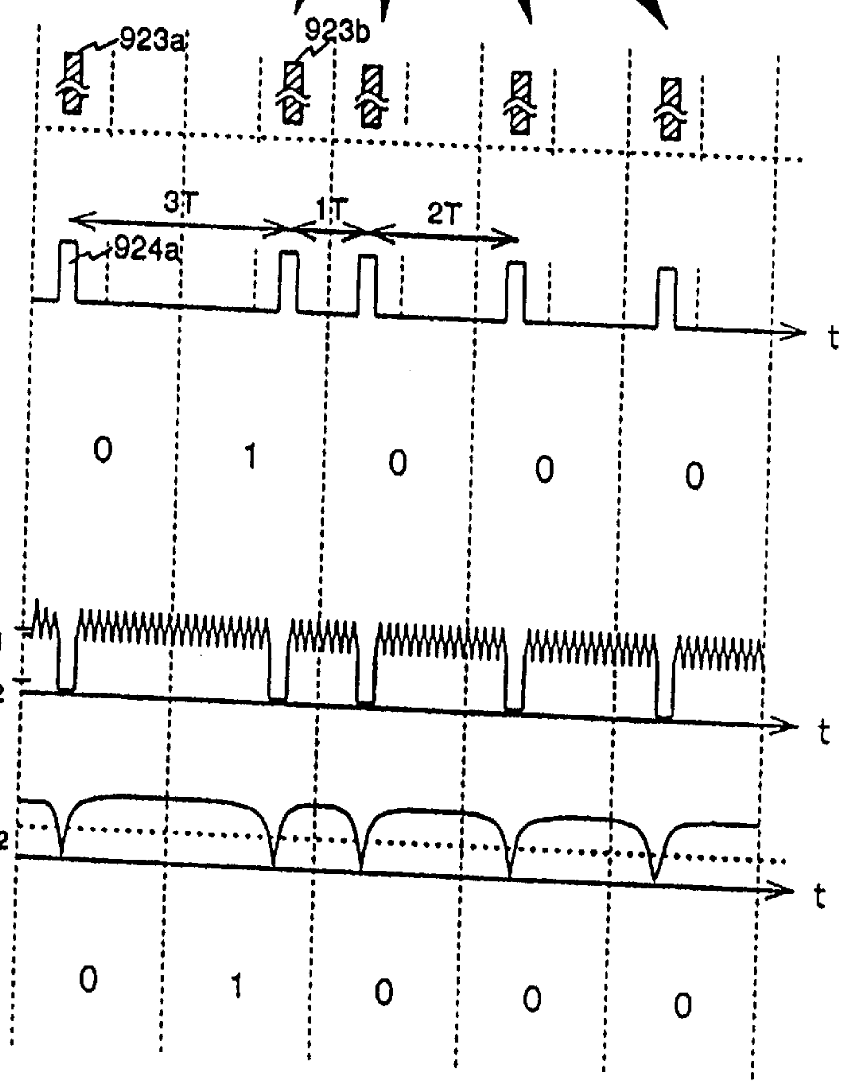
Fig. 3c Recorded Signal
