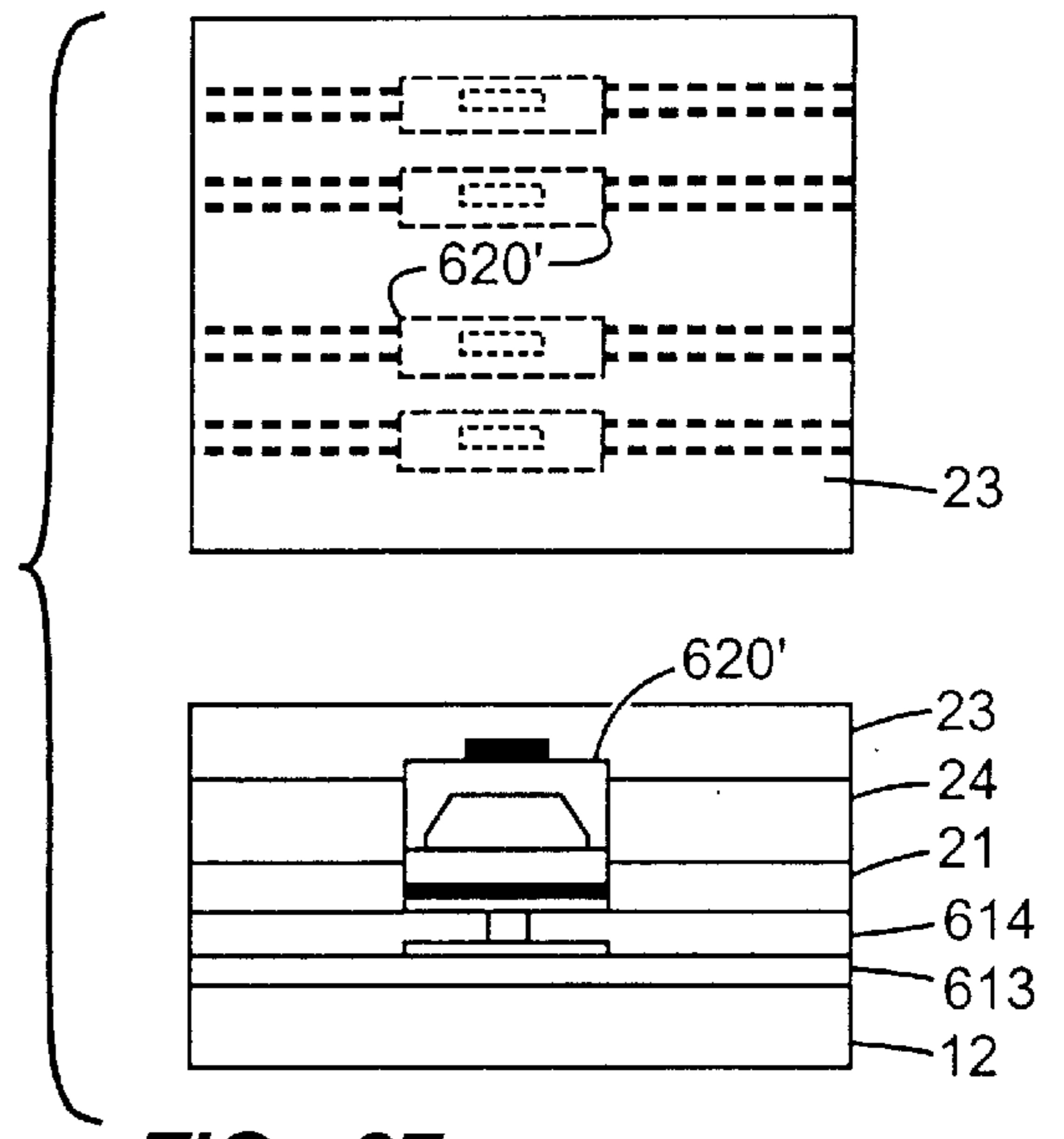
FIG. 87 (CLAD COATING)
