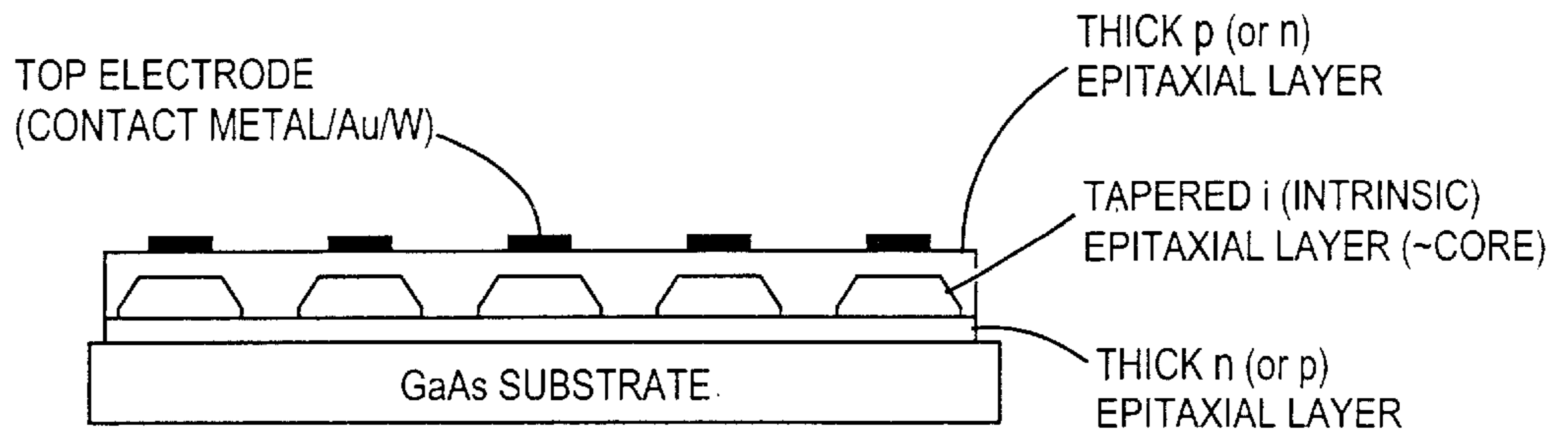
FIG. 82 (EPITAXIAL GROWTH)
