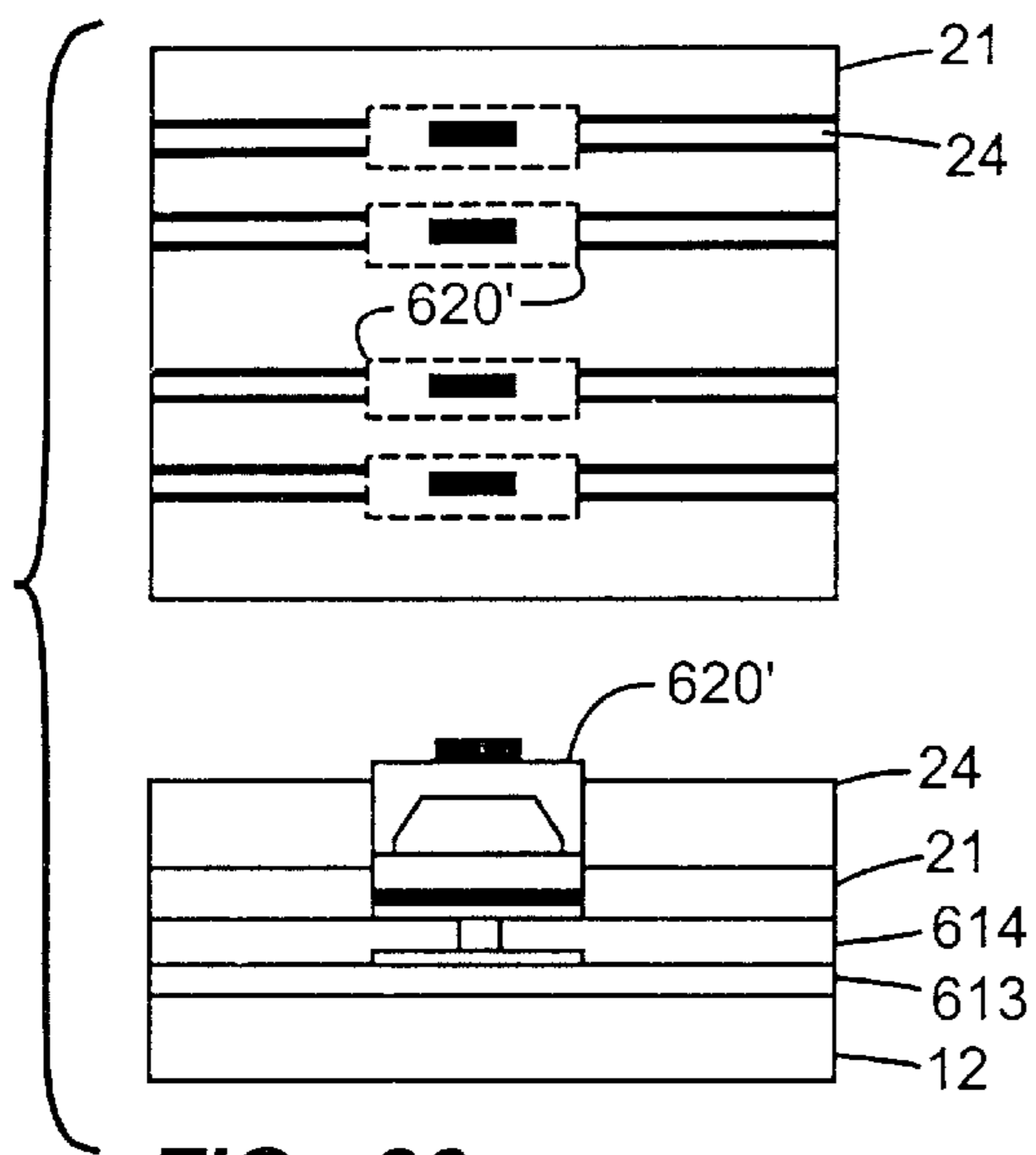
FIG. 86 (CORE PATTERNING)
