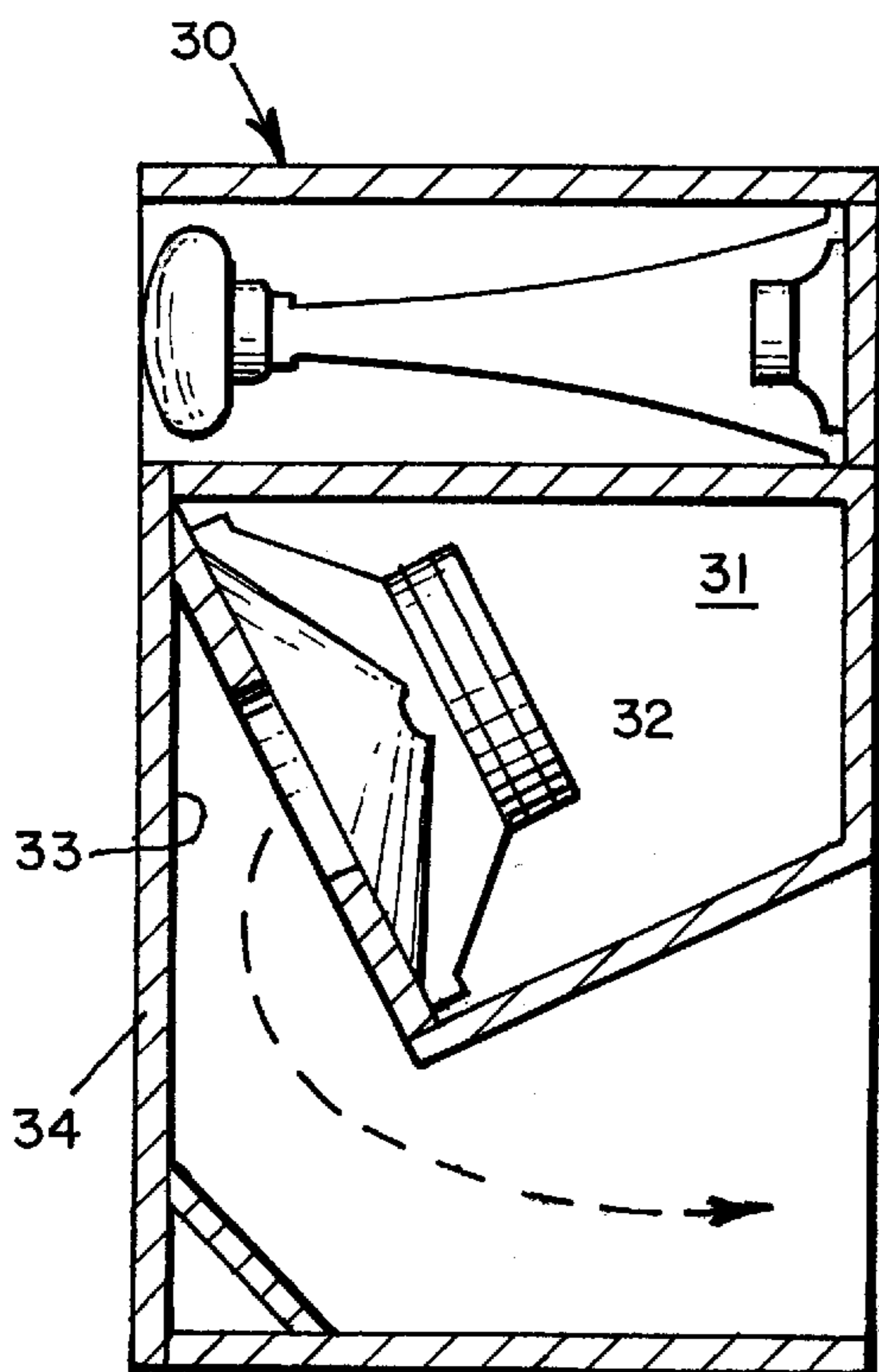
Fig. 3. (PRIOR ART)
