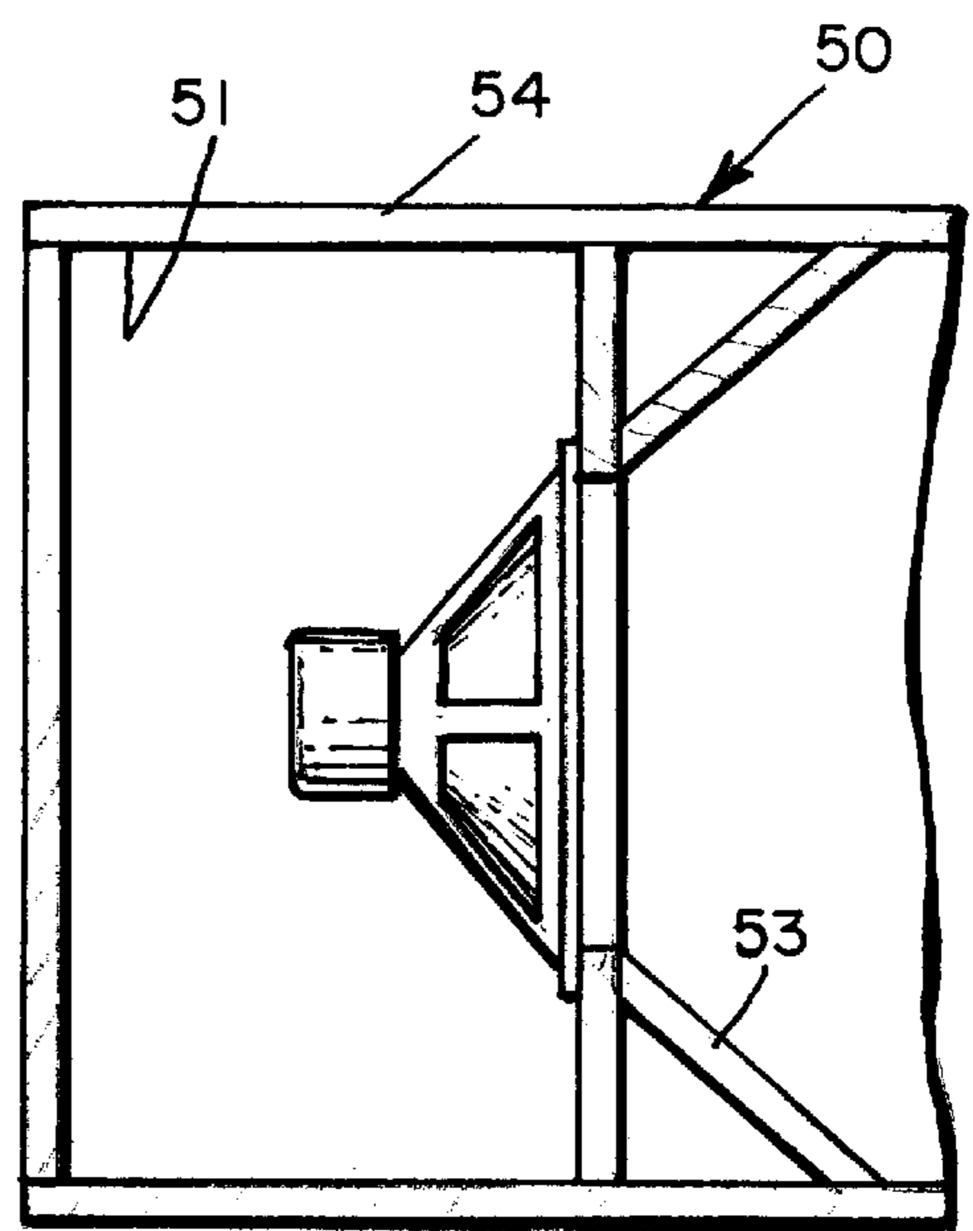
Fig. 6. (PRIOR ART)
