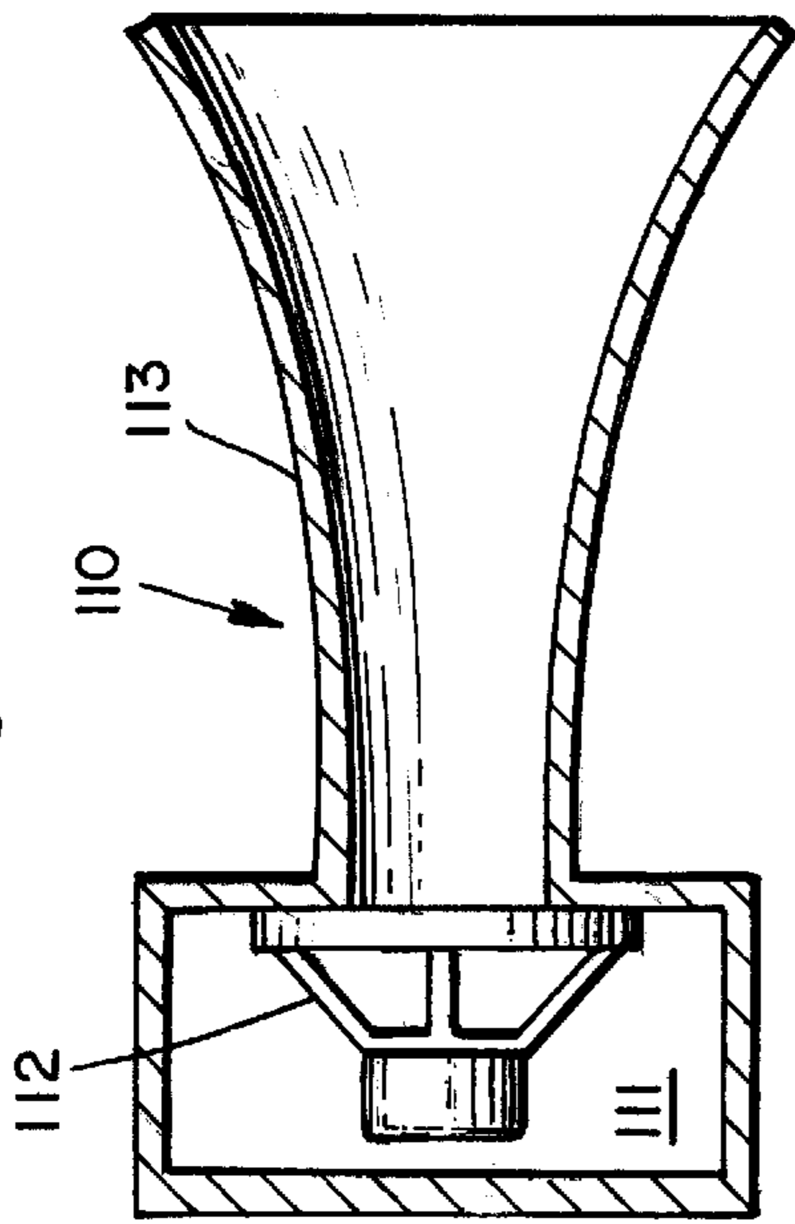
Fig. 8. (PRIOR ART)
