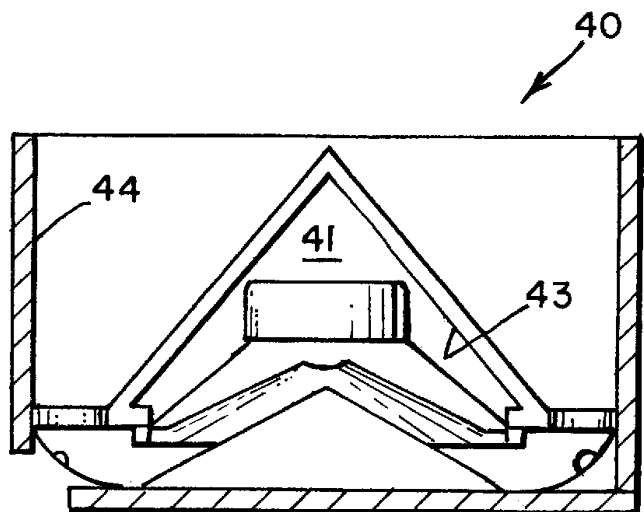
Fig. 4. (PRIOR ART)
