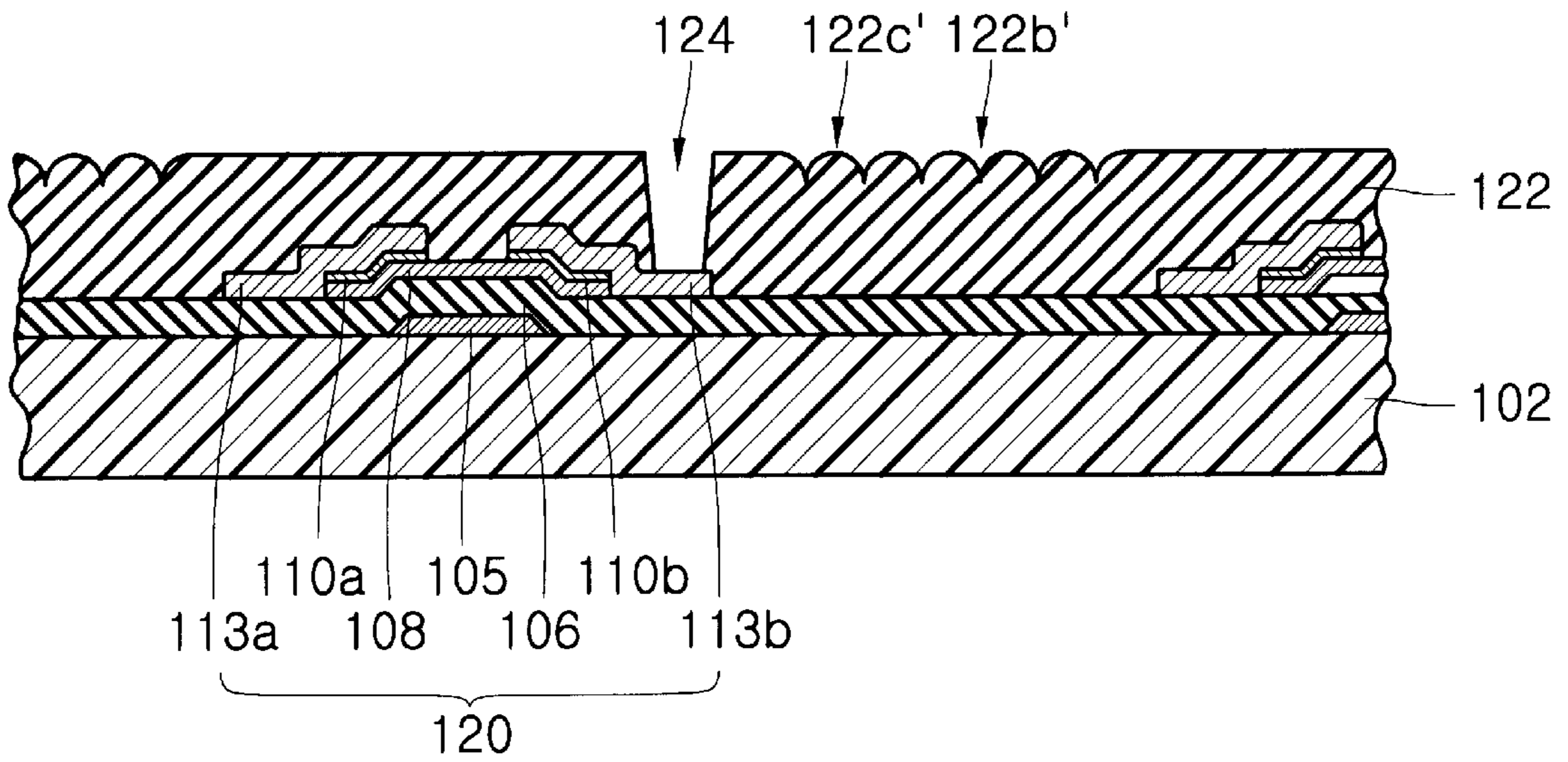
FIG. 3D
