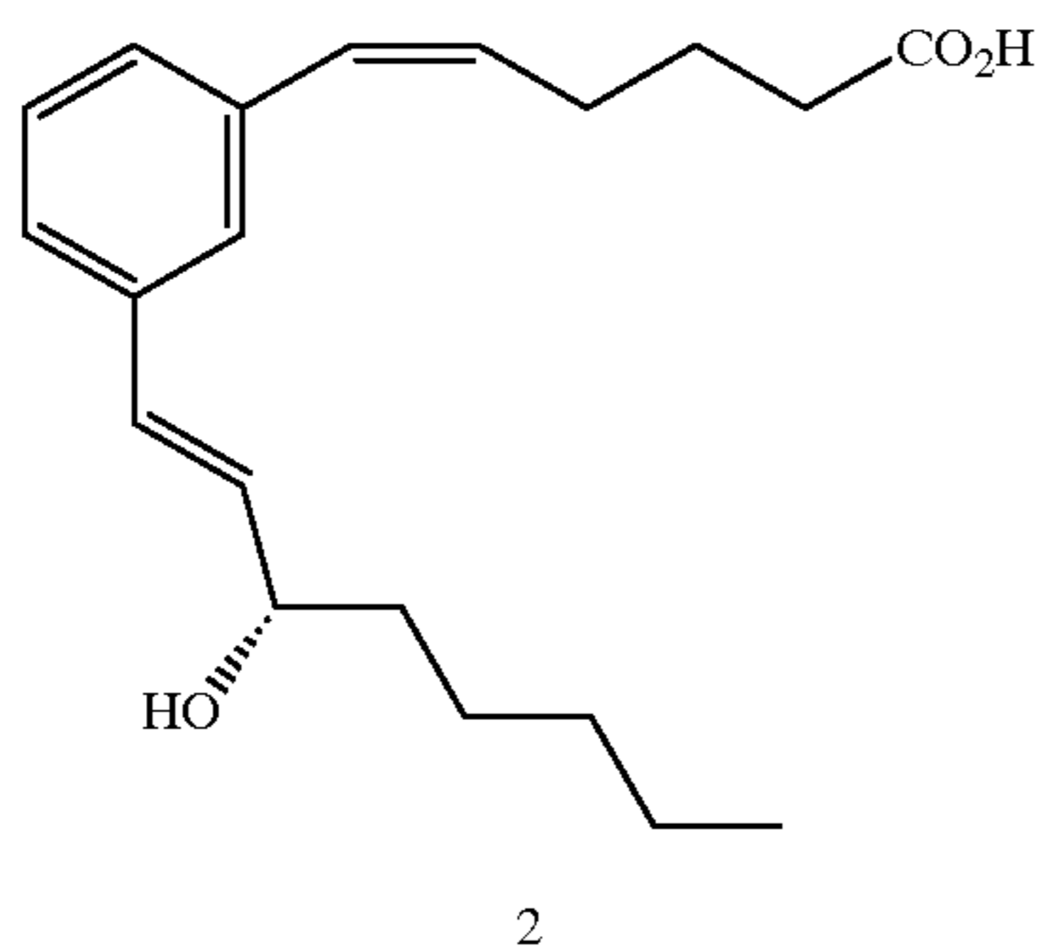
(5Z)-6-[3-(3R-hydroxy-1E-octenyl)-1-phenyl]hex-5-enoic acid (2)
