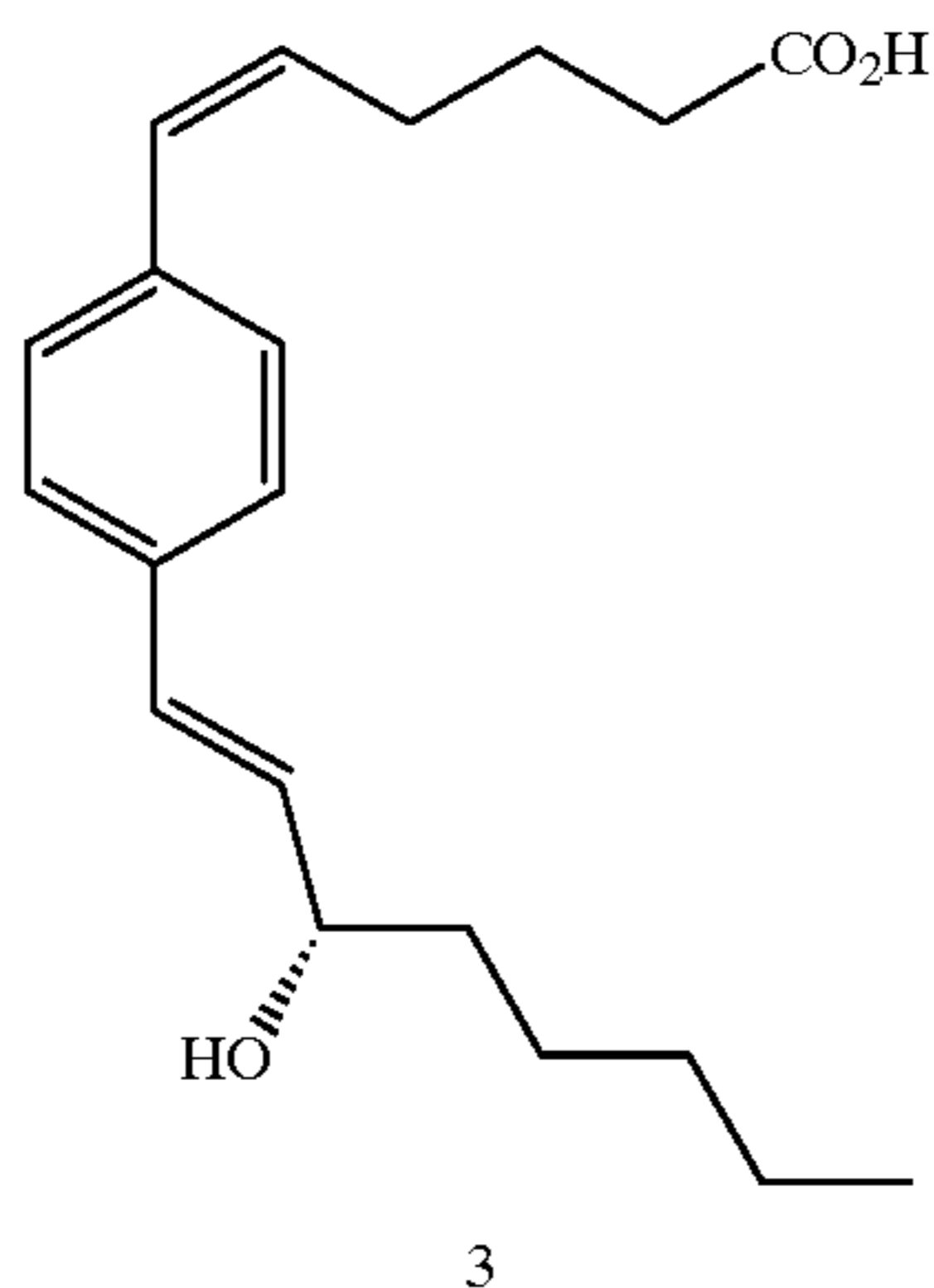
(5Z)-6-[4-(3R-hydroxy-1E-octenyl)-1-phenyl]hex-5-enoic acid (3)
