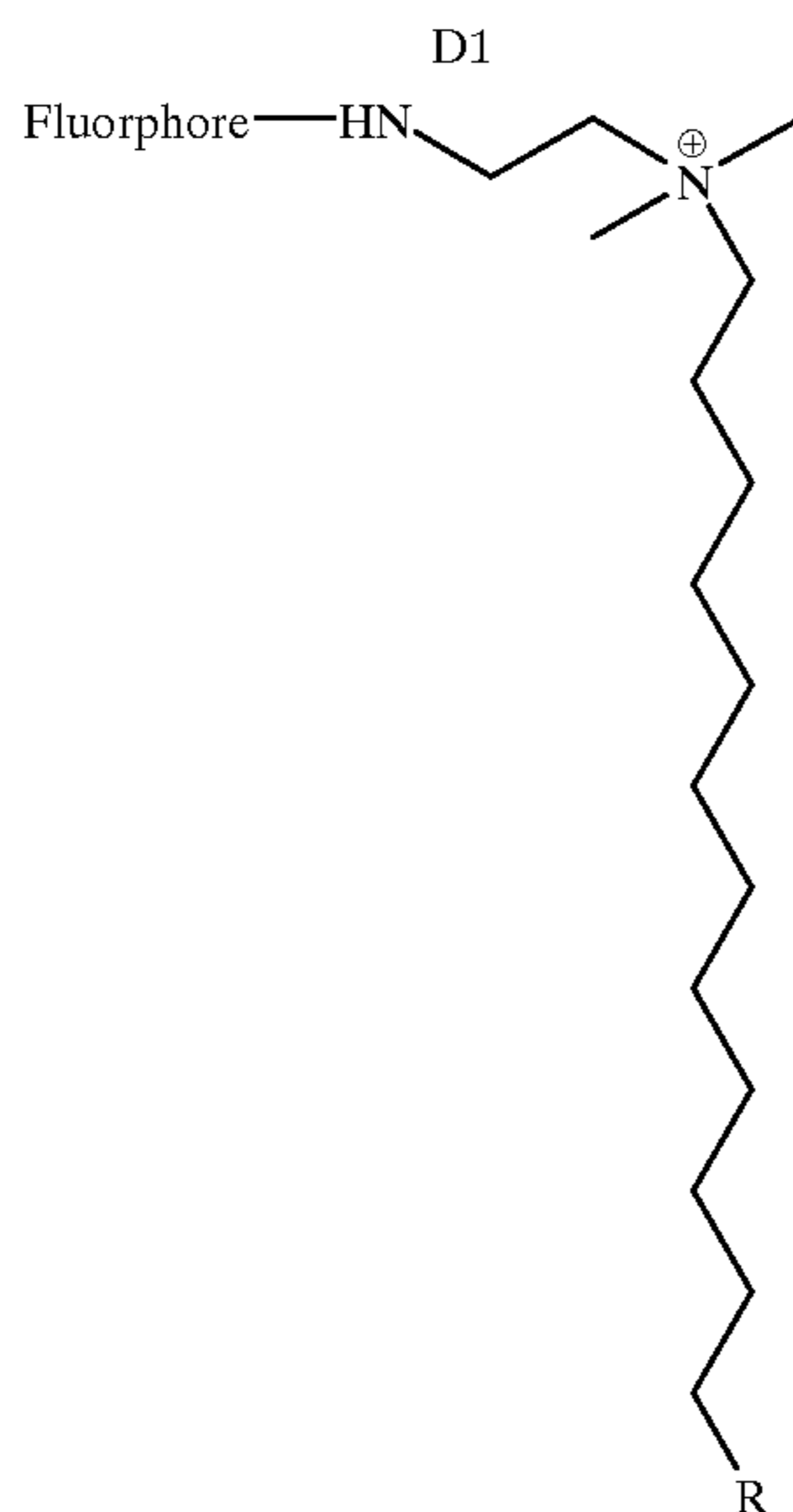
D2: Generic fluorescent quaternary ammonium lipid R = 0 to 20 methylene equivalents
