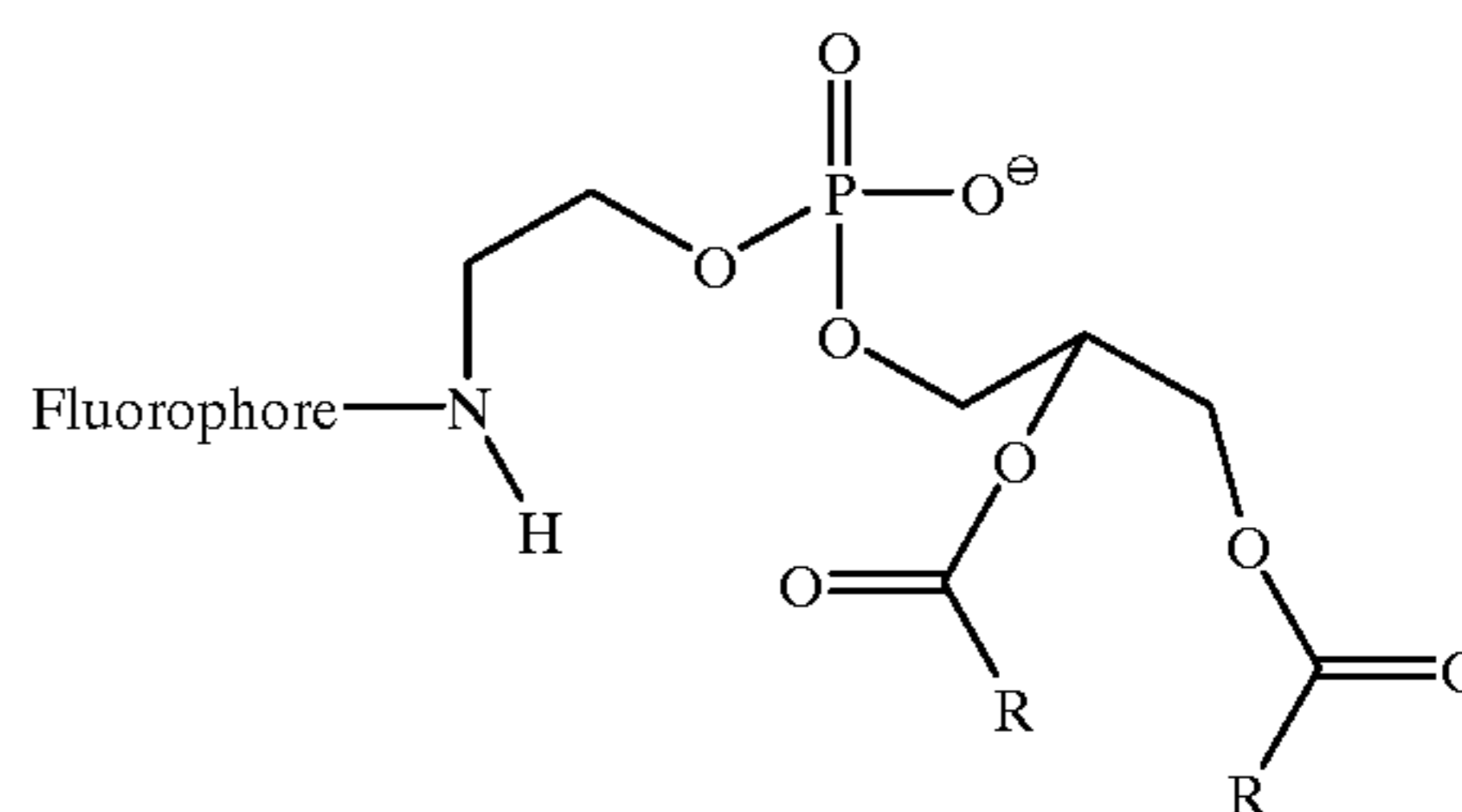
C: Generic FI-PE
