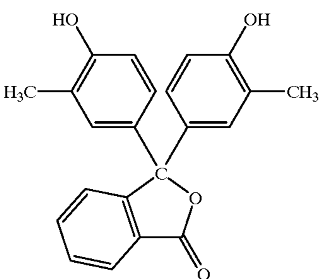
o-cresolphthalein and
