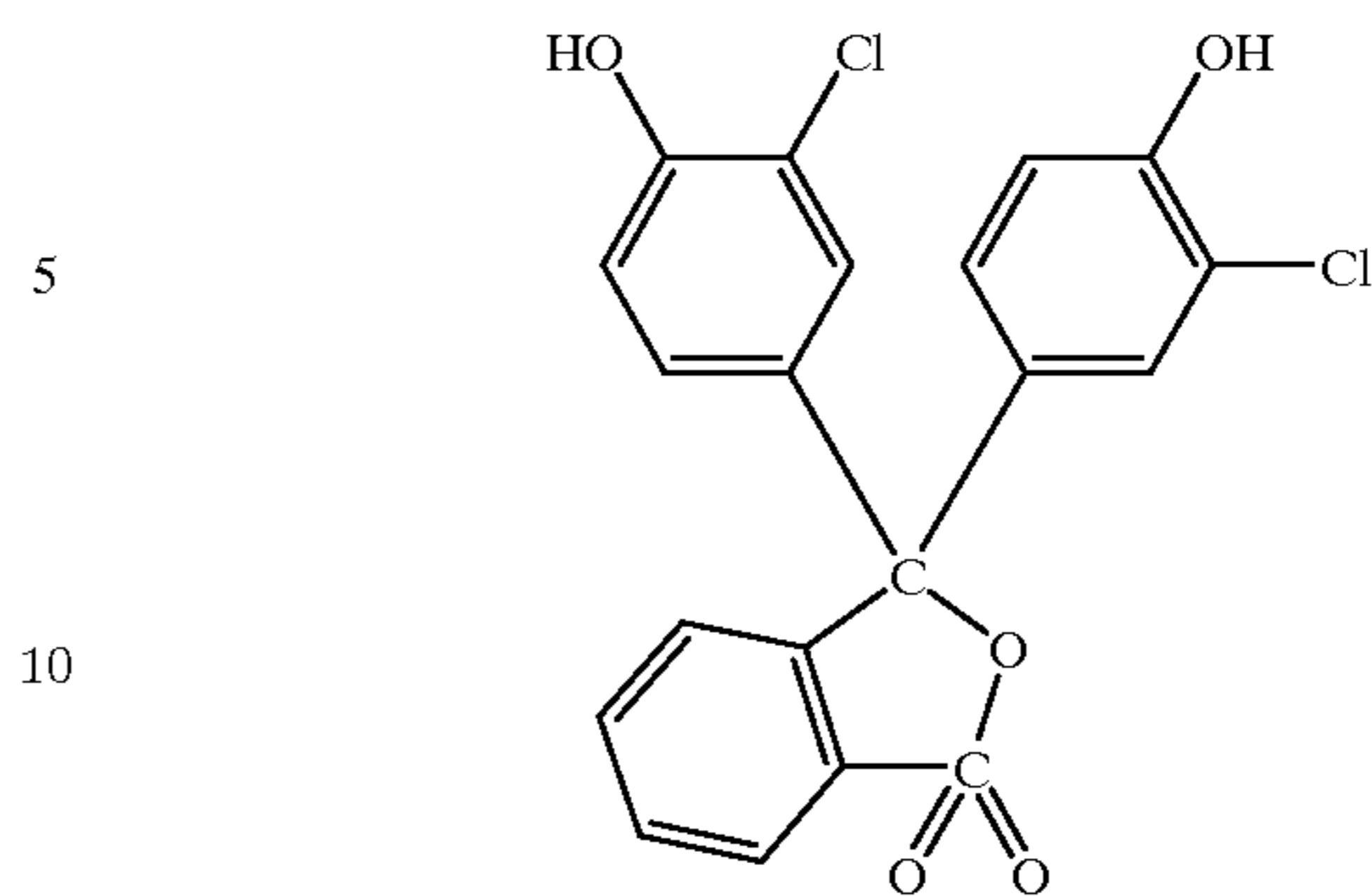
chlorophenol red
