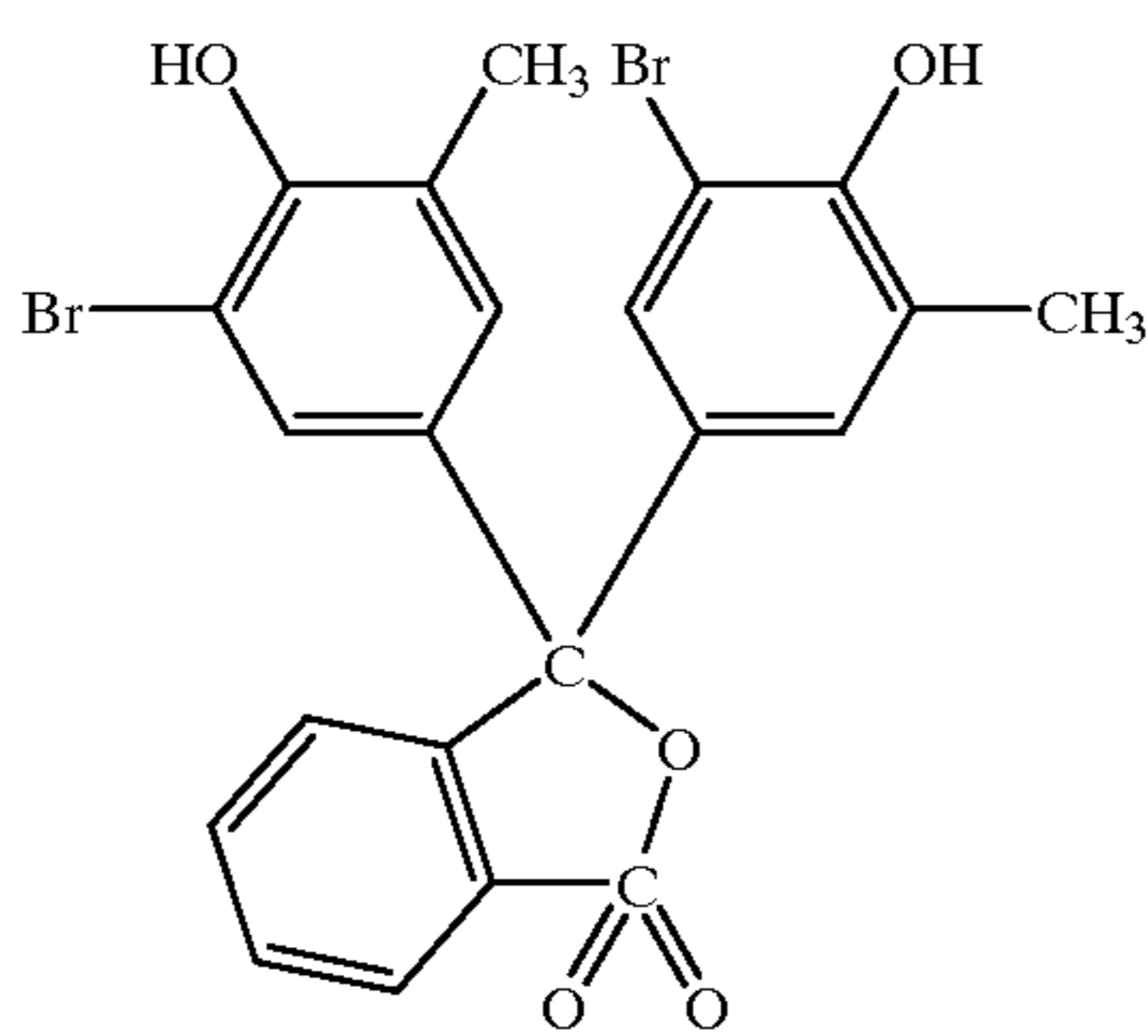
bromocresol purple
