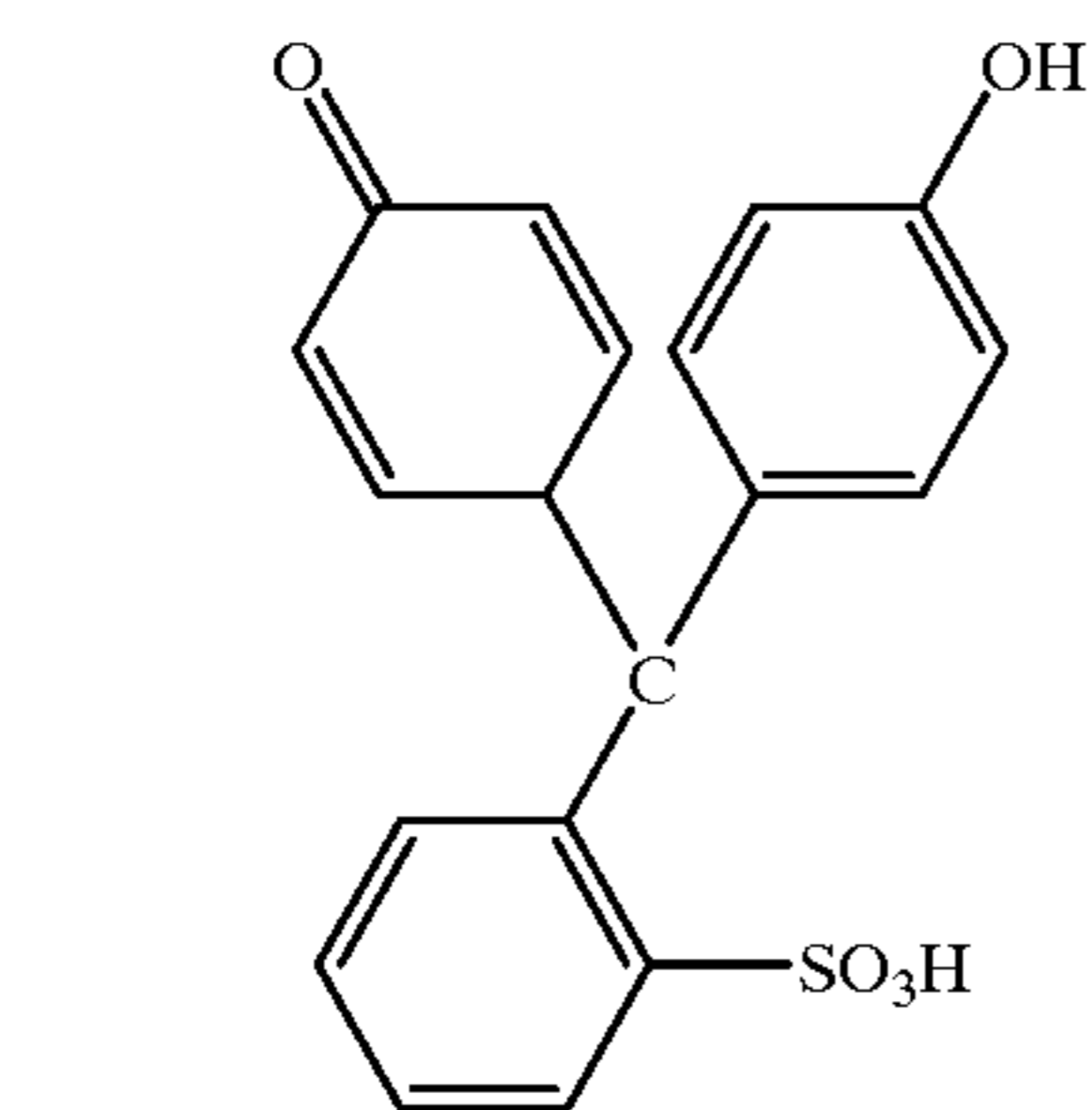
phenol red
