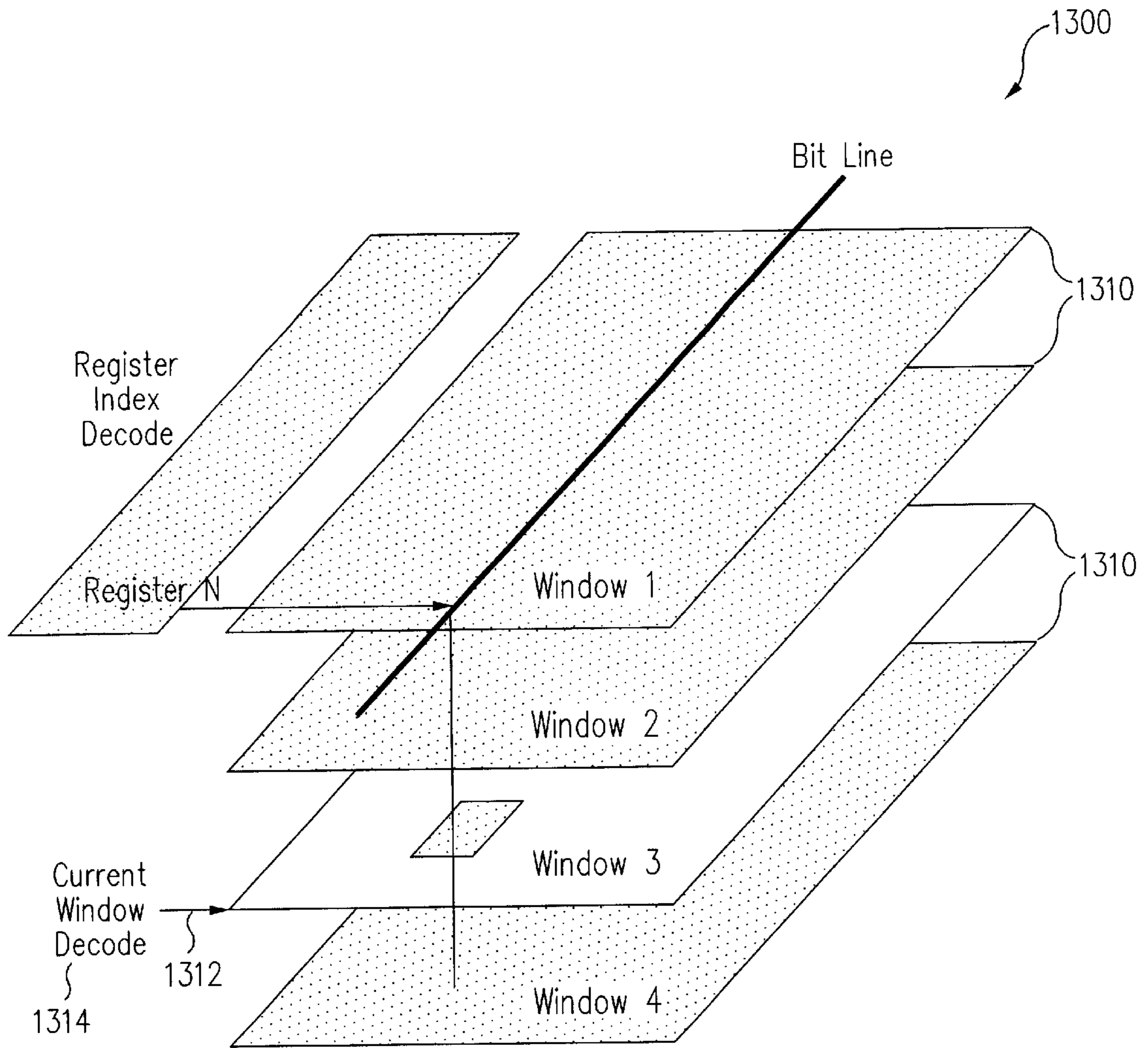
A Three Dimensional Register File
