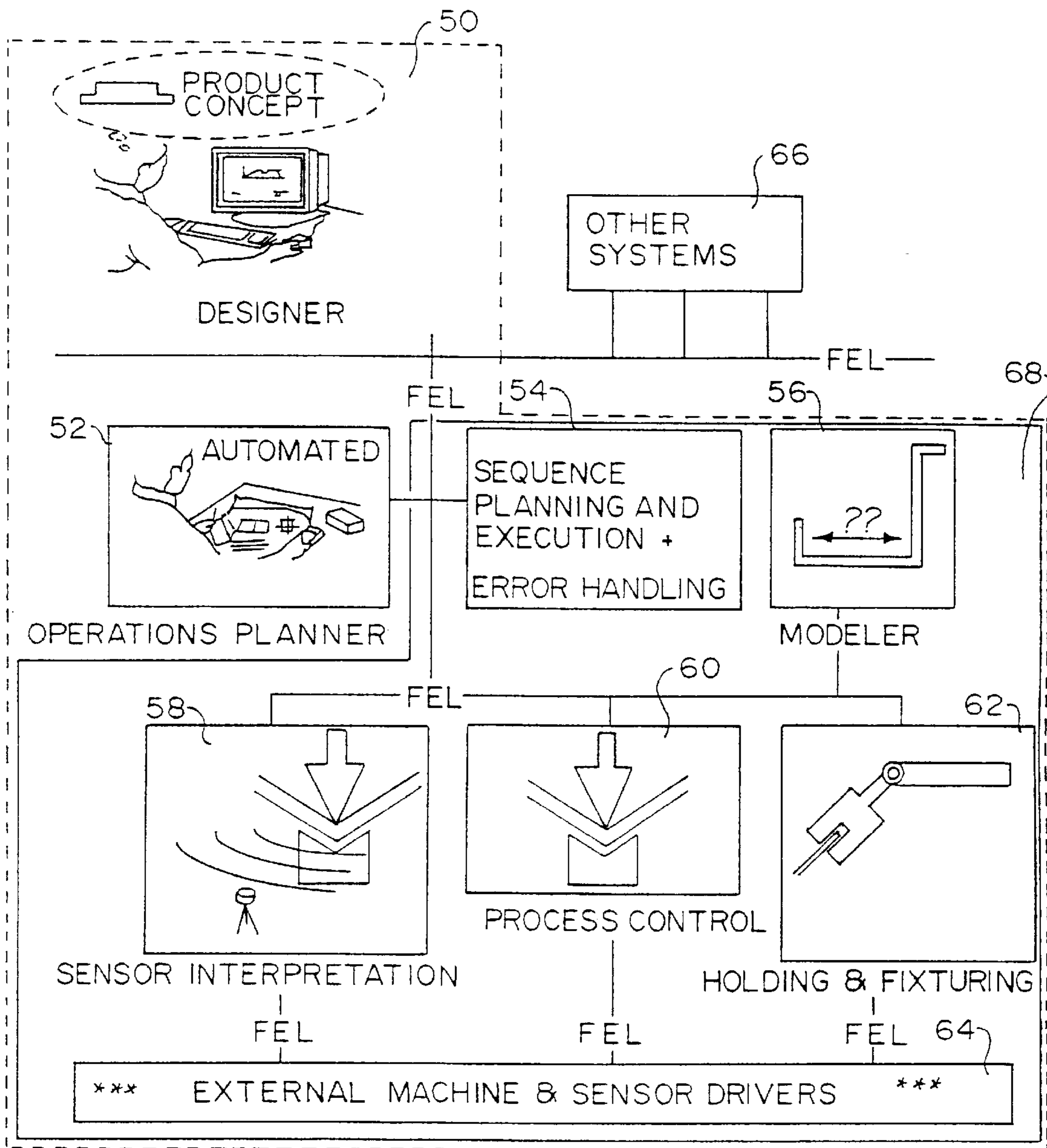
FIG. 4 PRIOR ART
