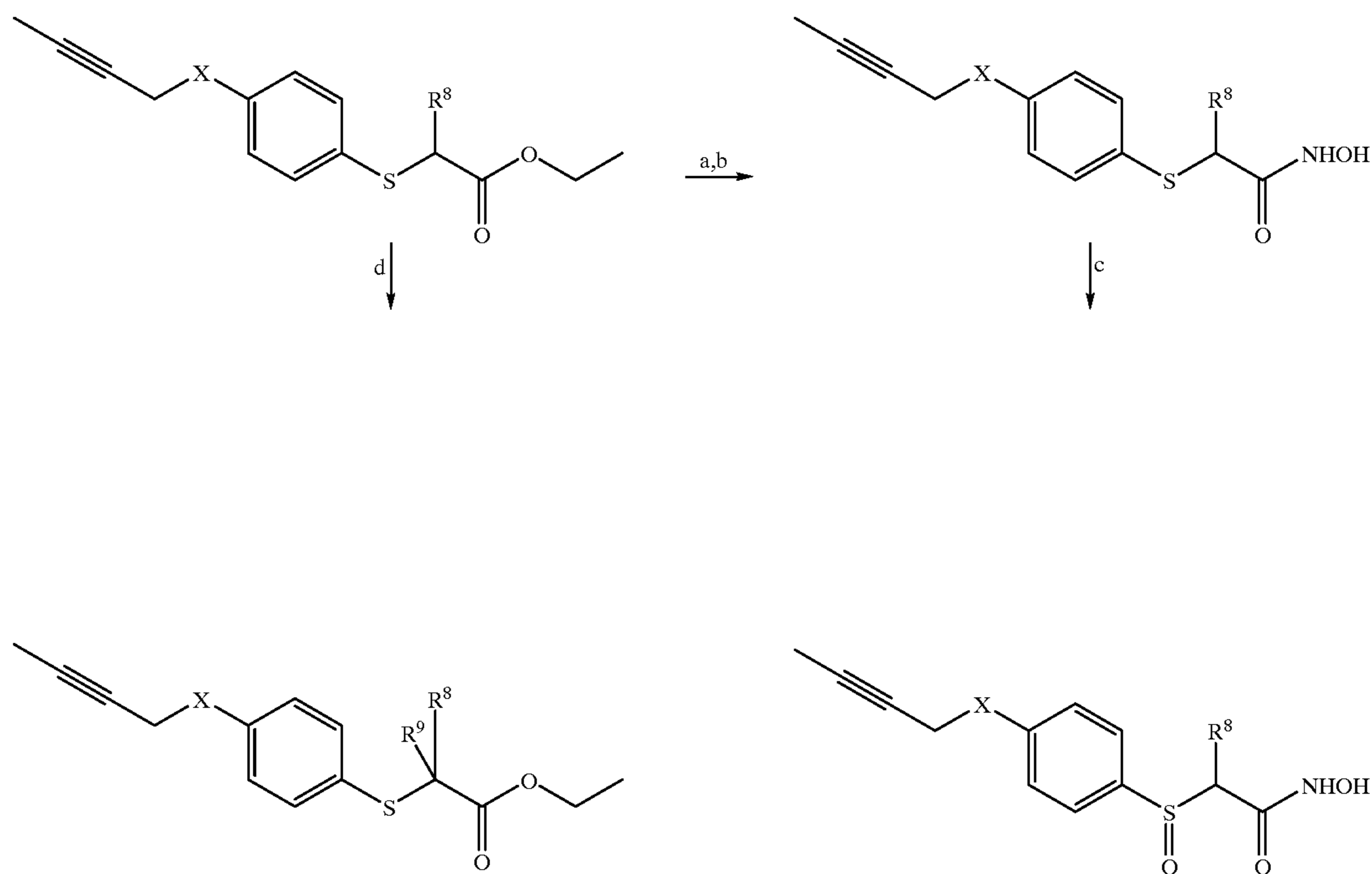
Scheme 2:
