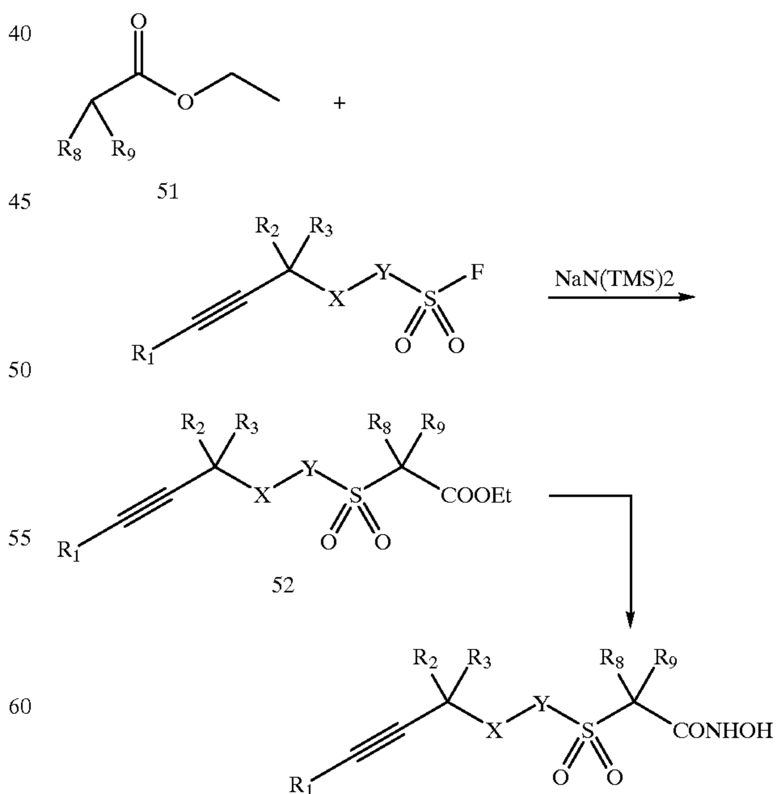
Scheme 12
