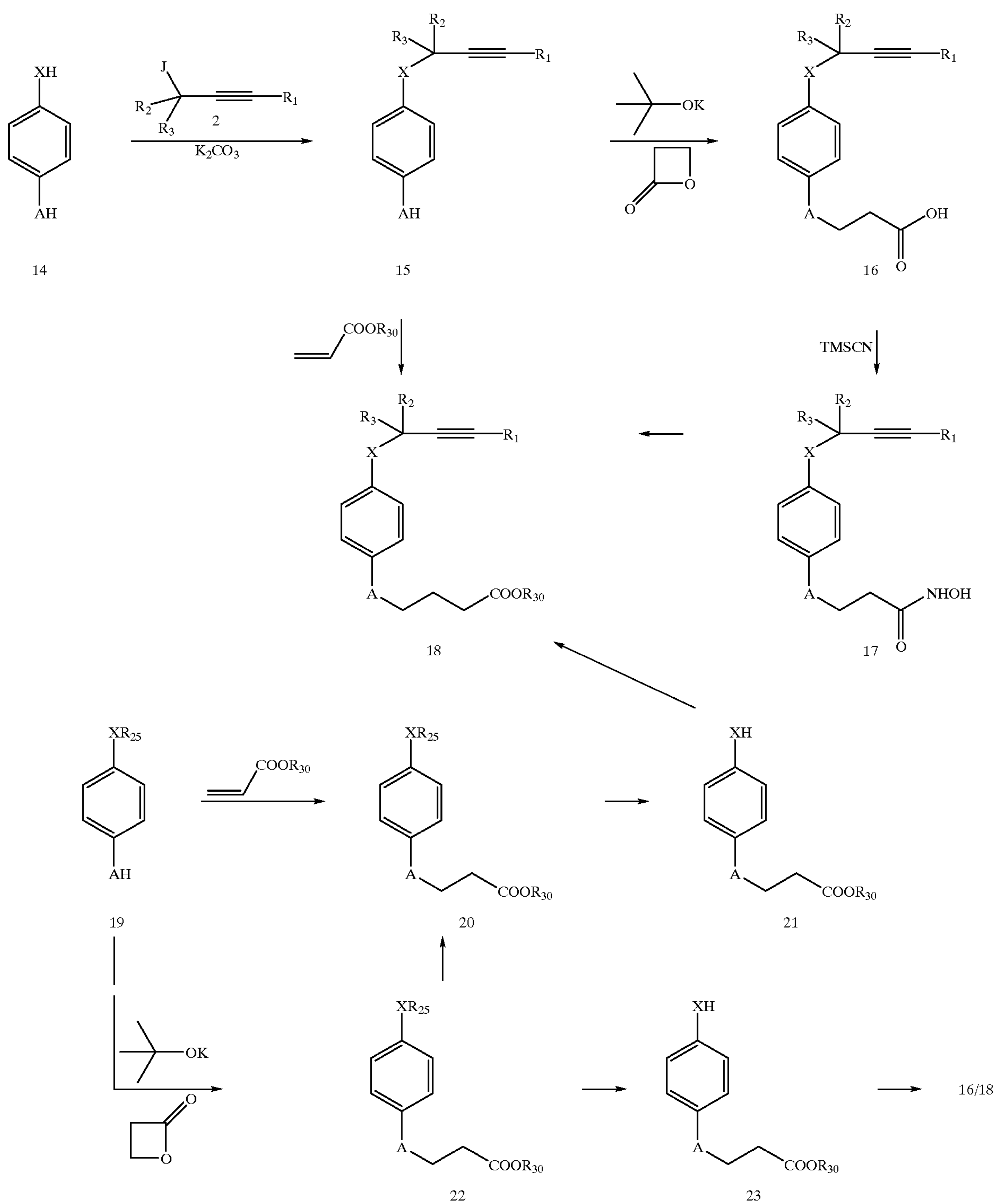
Scheme 4
