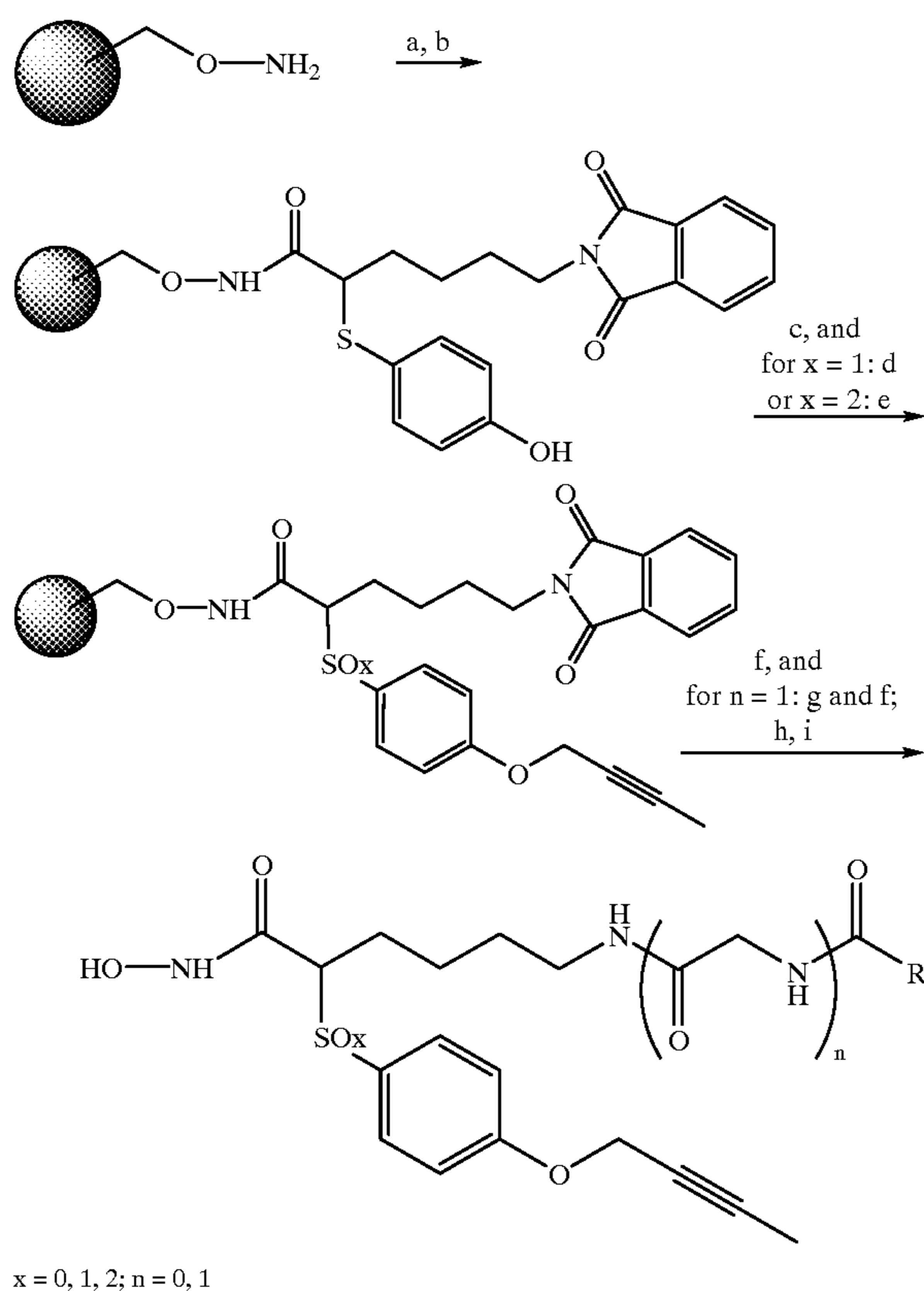
Scheme 11
