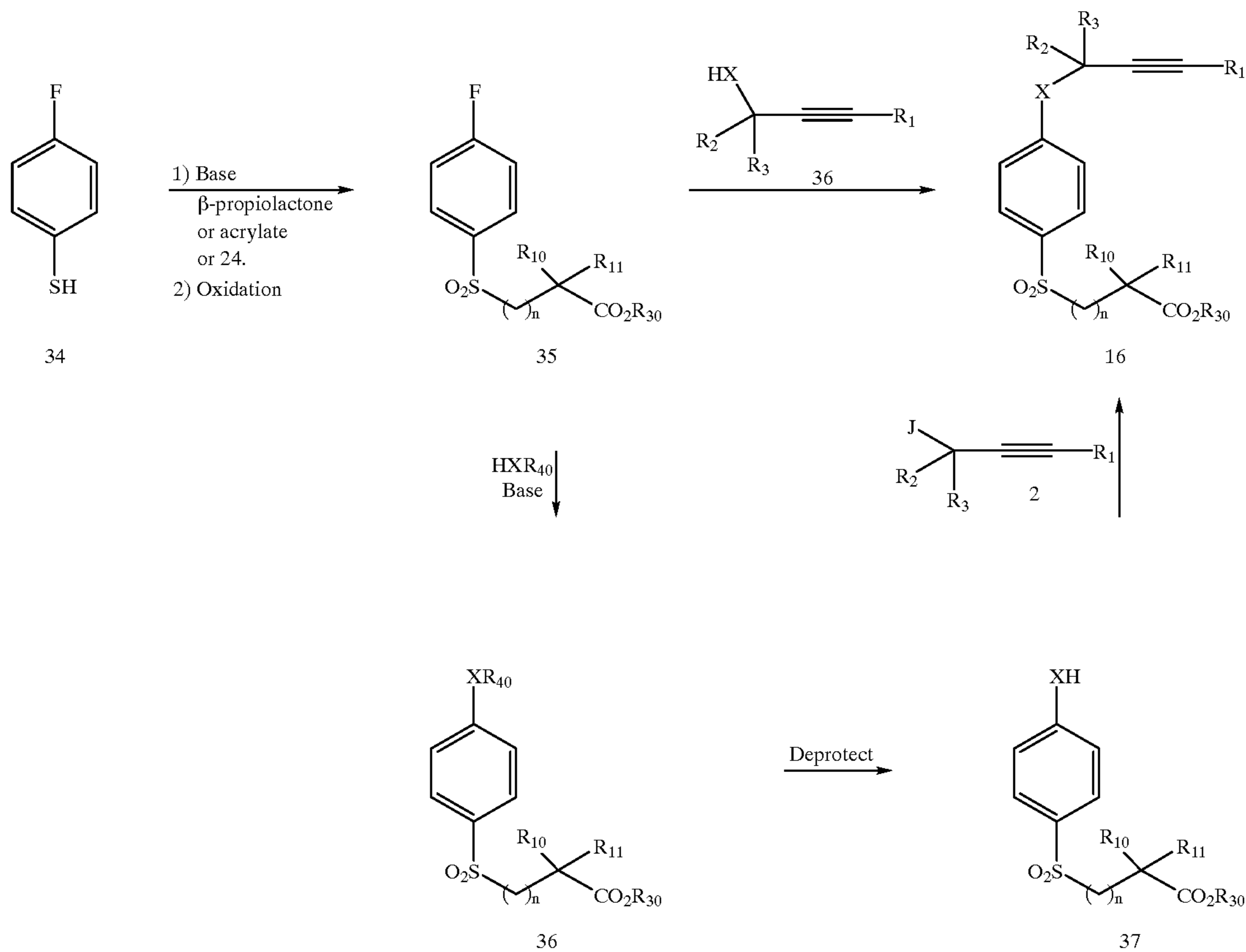
Scheme 7
