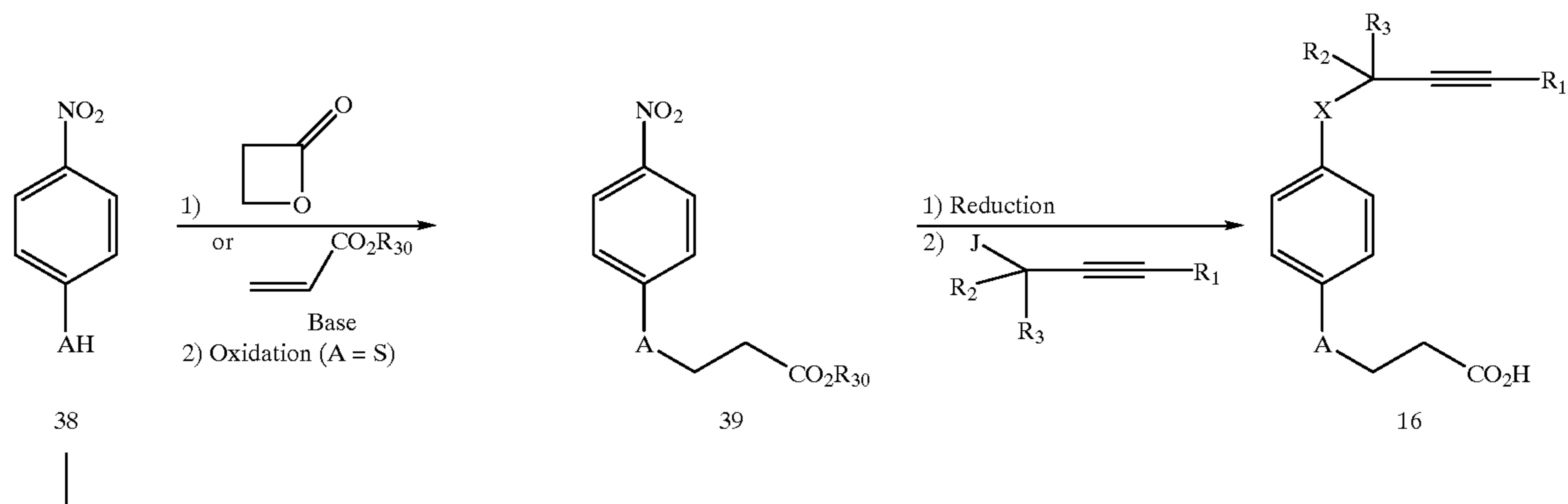
Scheme 8
