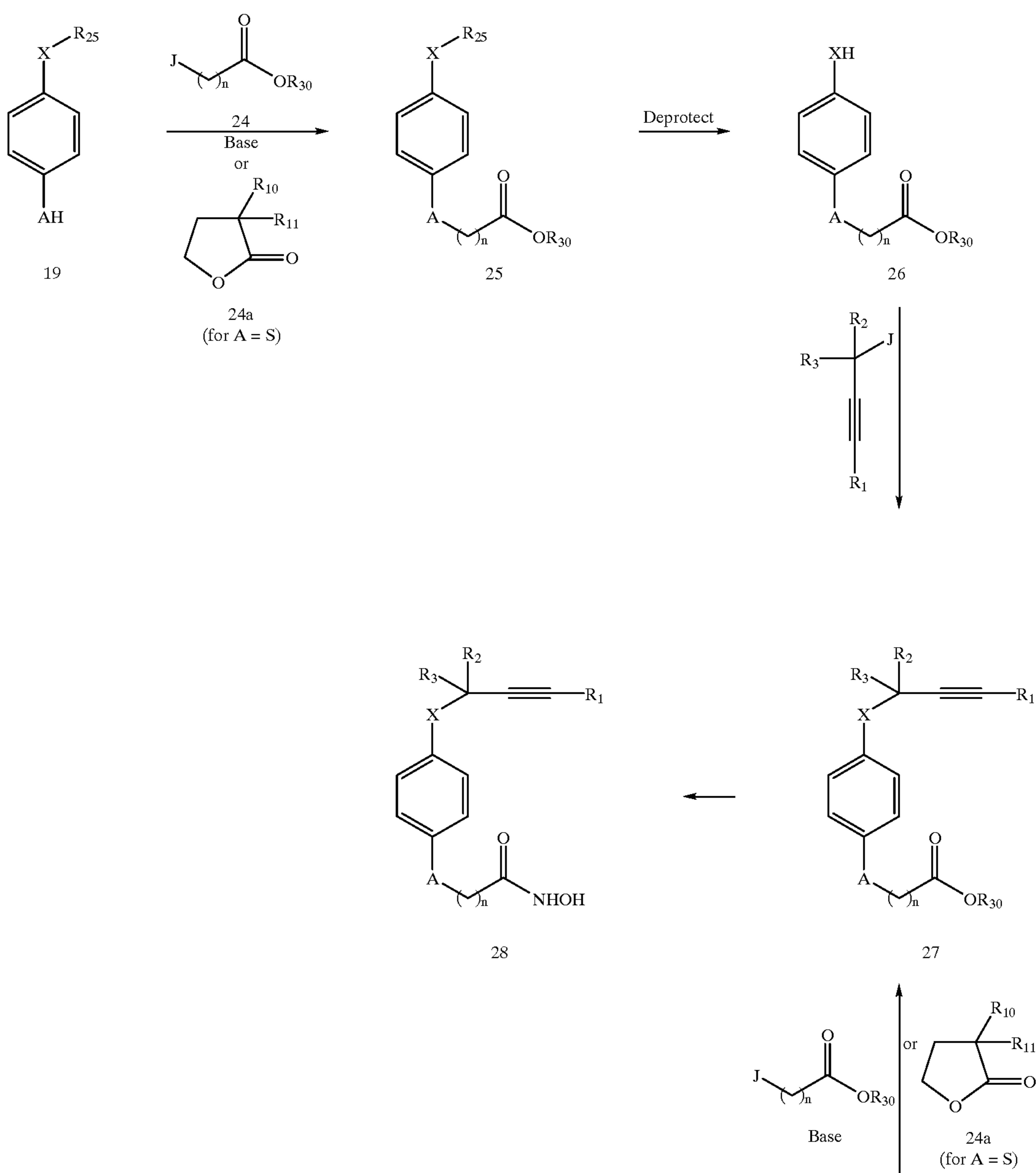
Scheme 5
