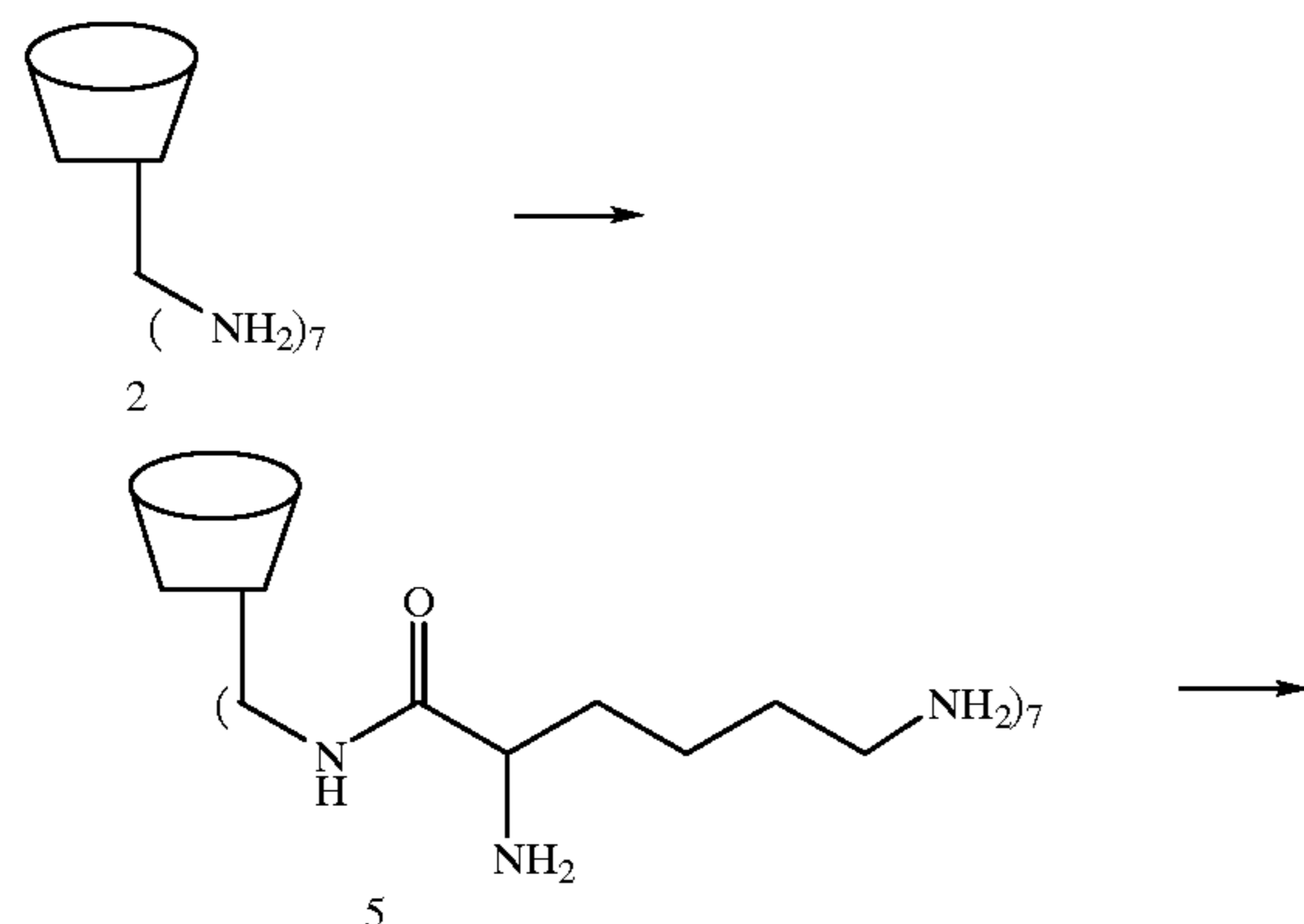
Scheme 6
