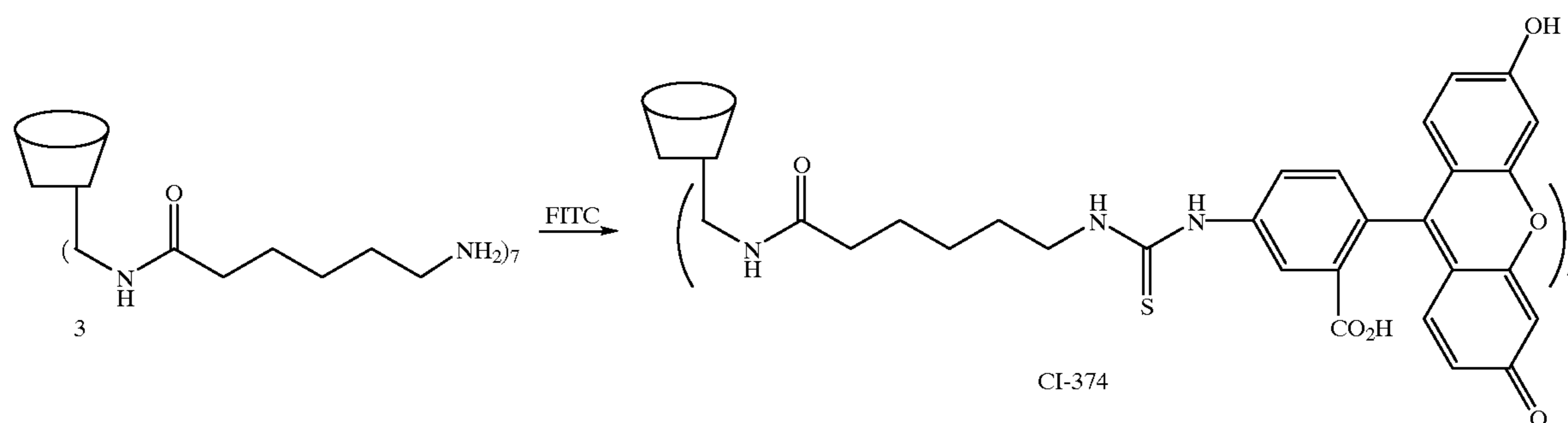
Scheme 5
