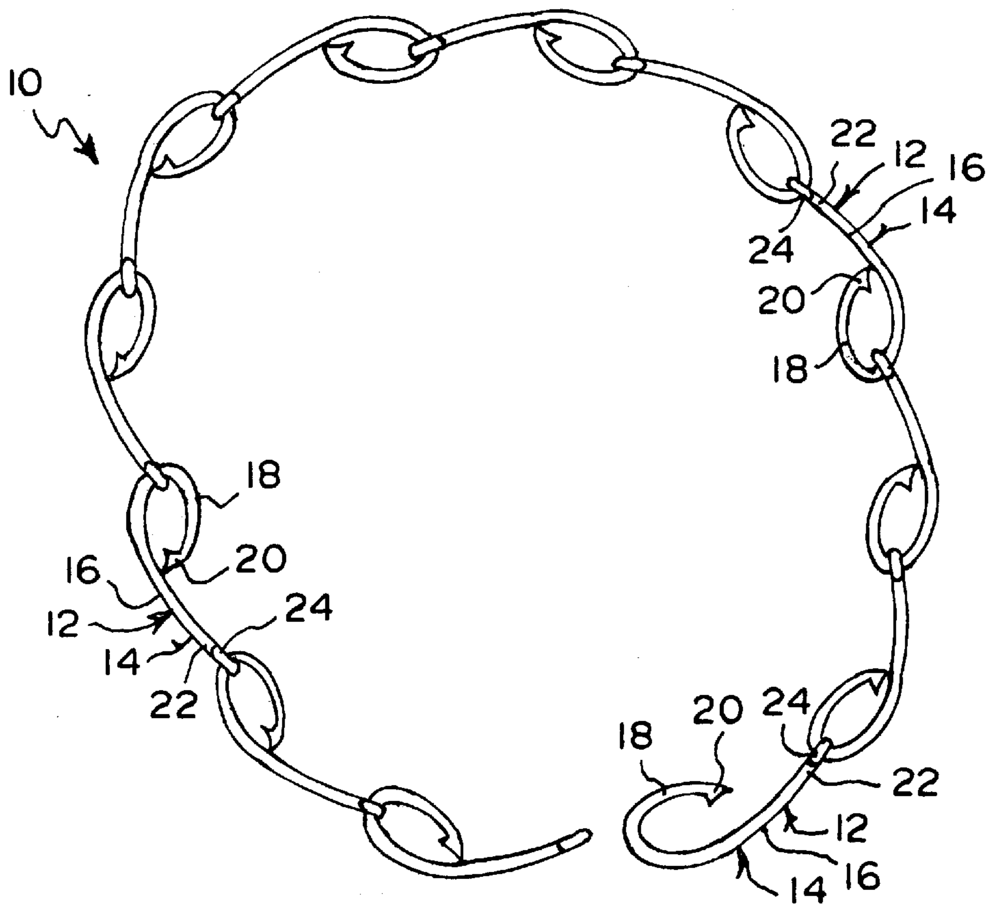
Fig. 1 (PRIOR ART)
