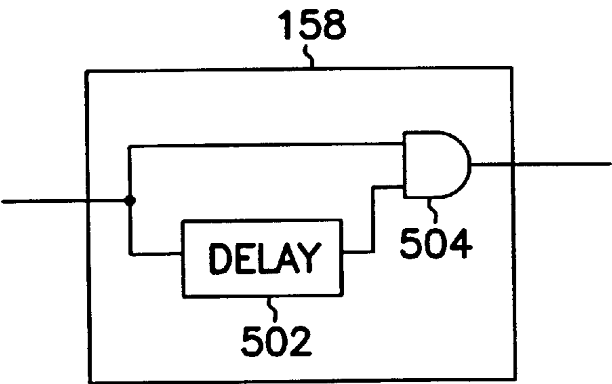
FIG. 6 (PRIOR ART)
