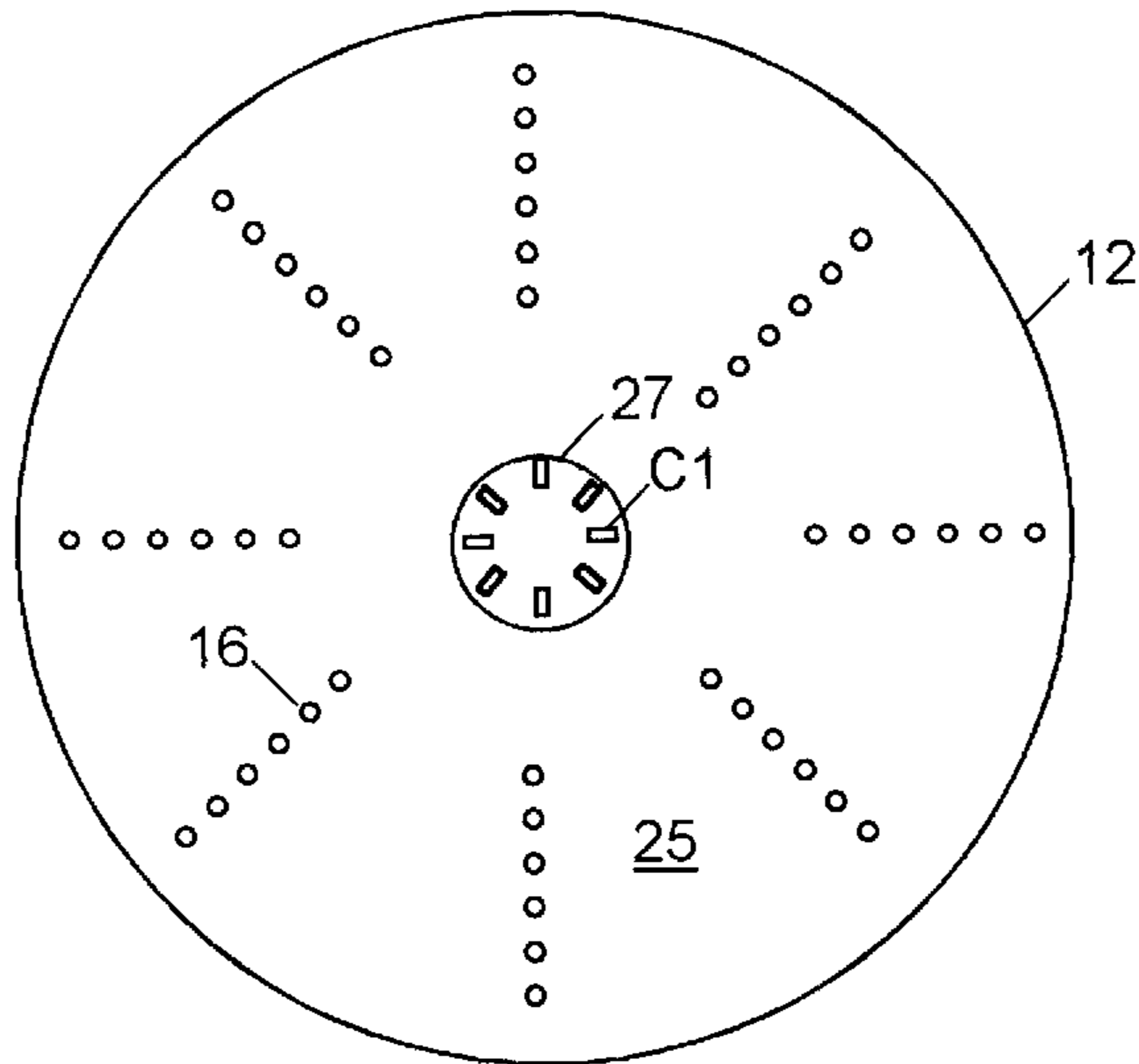
FIG. 4 (PRIOR ART)
