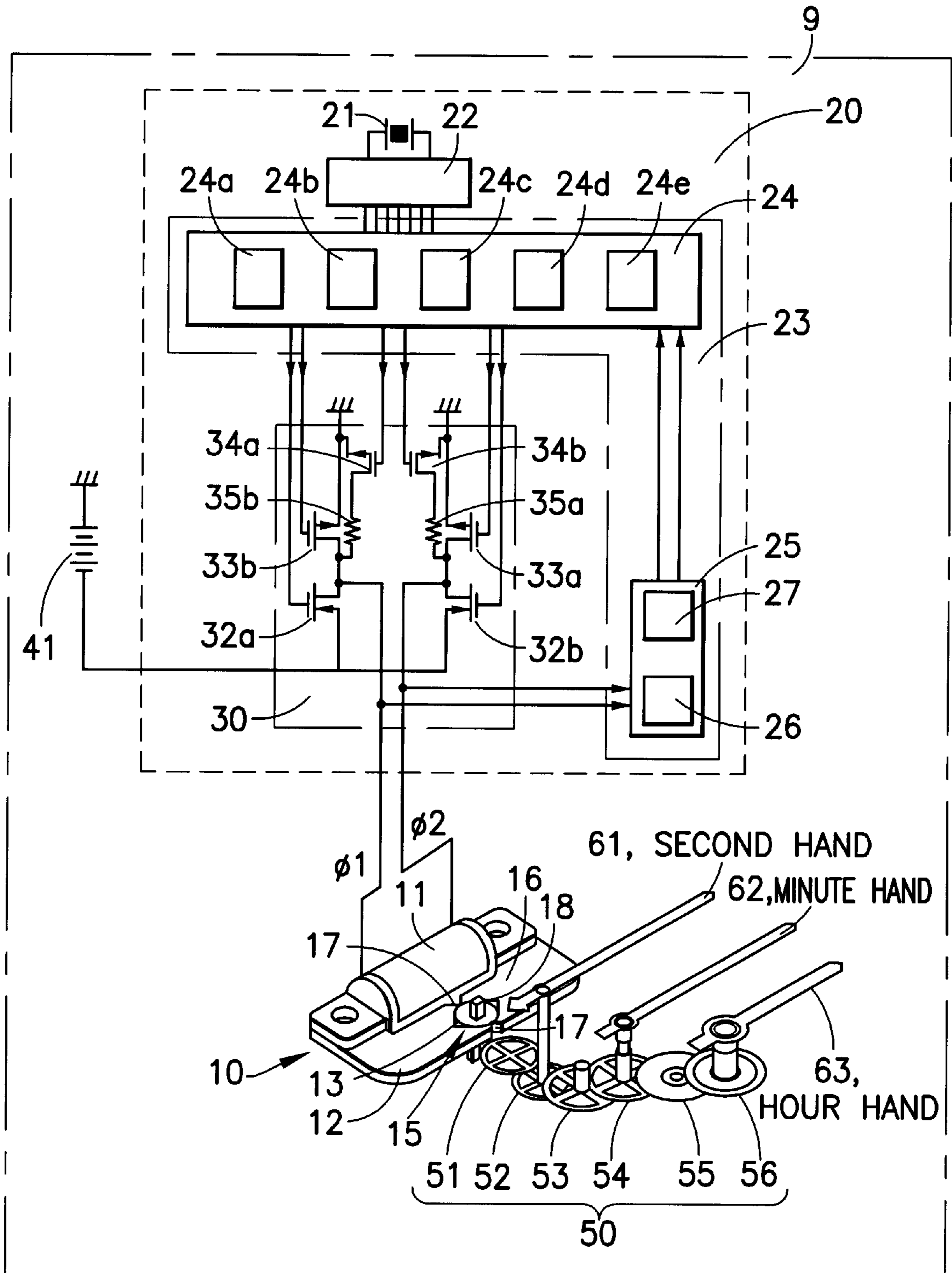
FIG. 12 PRIOR ART
