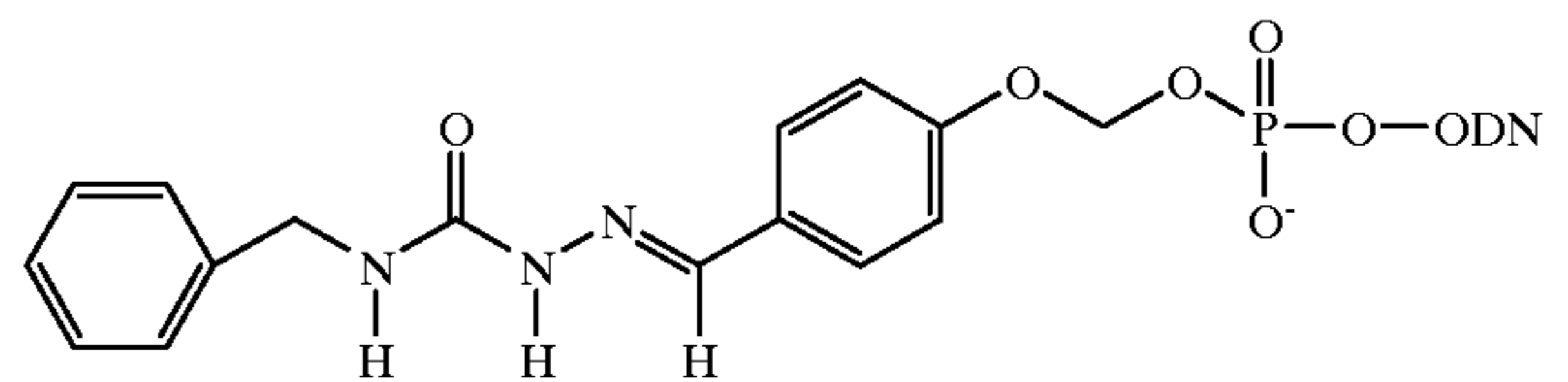
Formula 10
