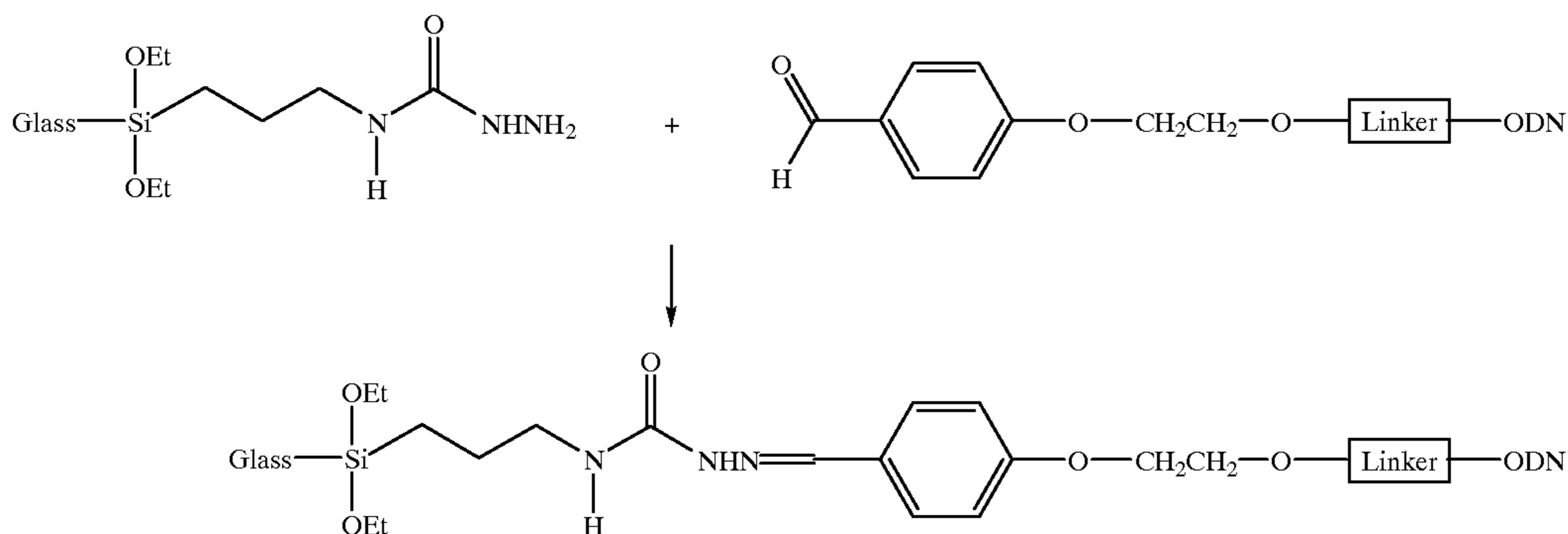
Reaction Scheme 4
