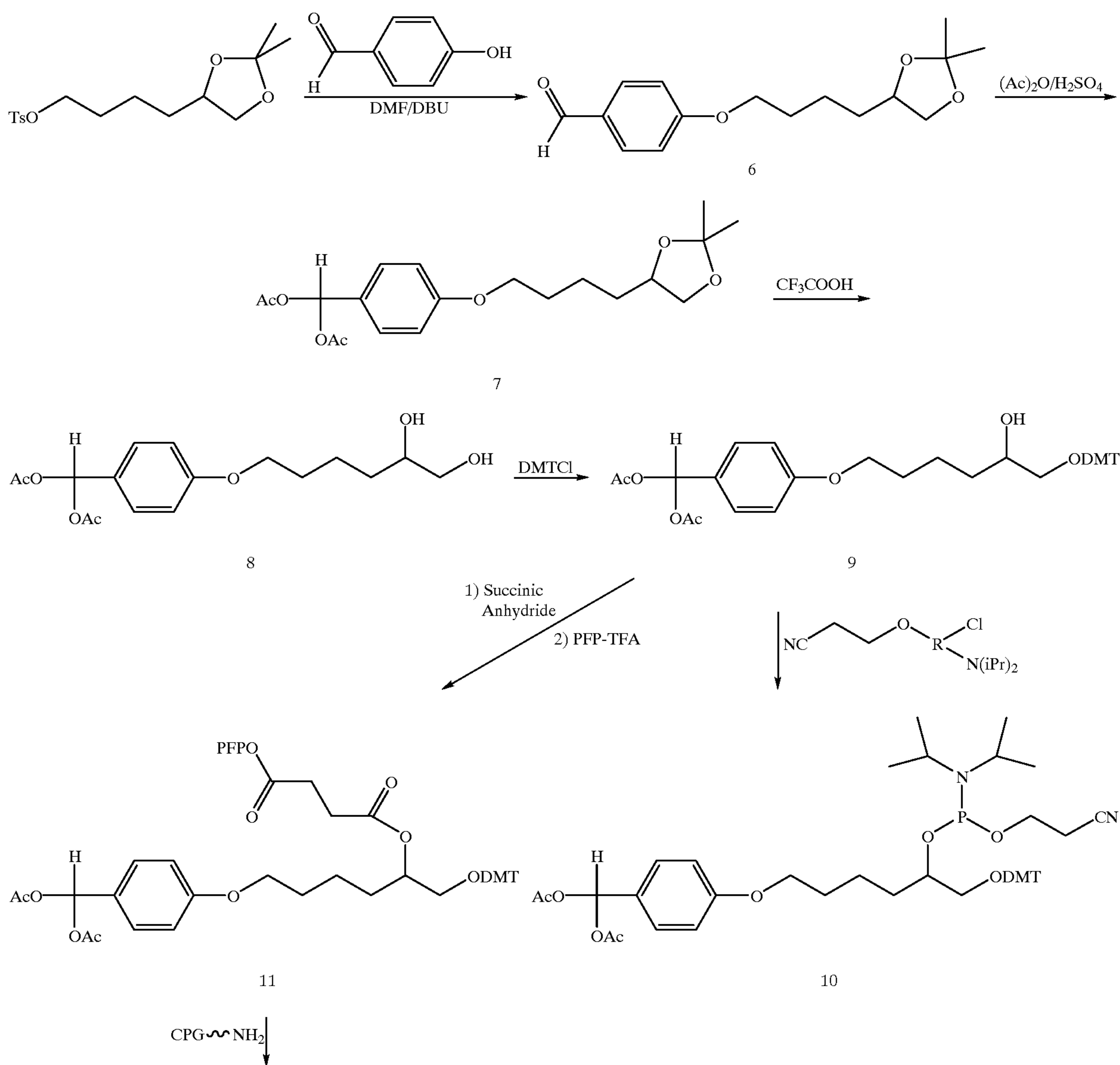
Reaction Scheme 3
