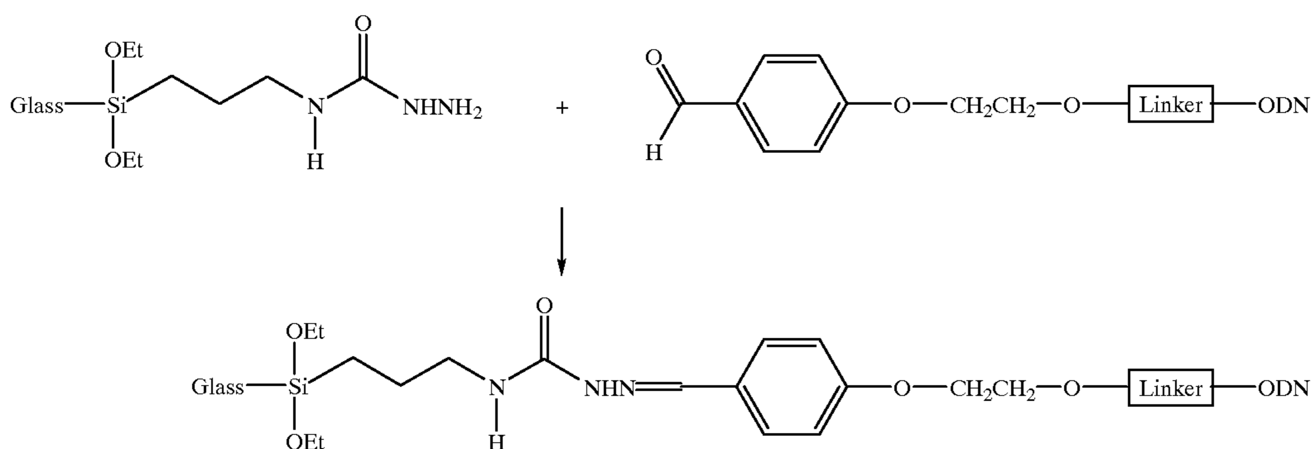
Reaction Scheme 4
