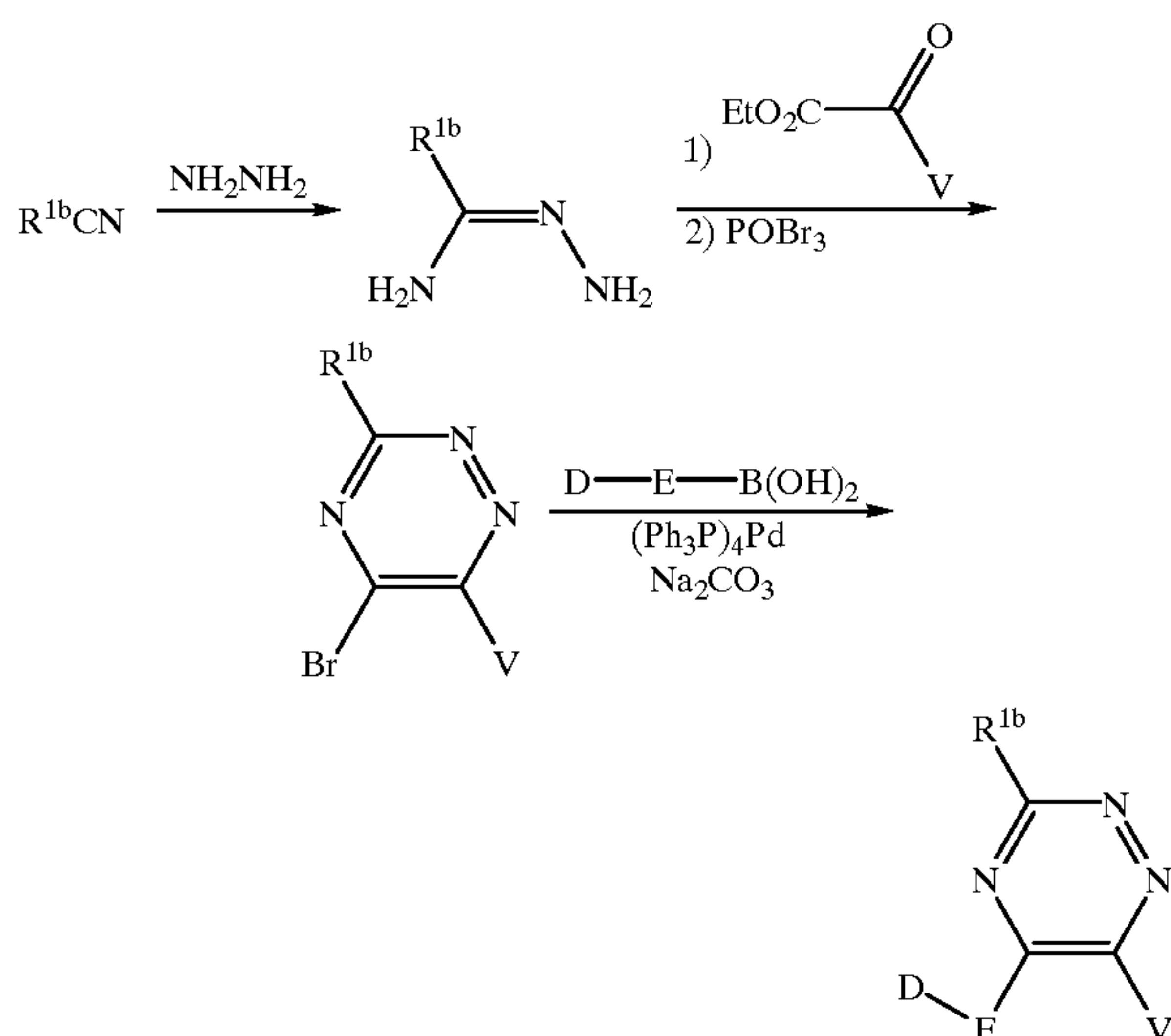
Scheme 54
