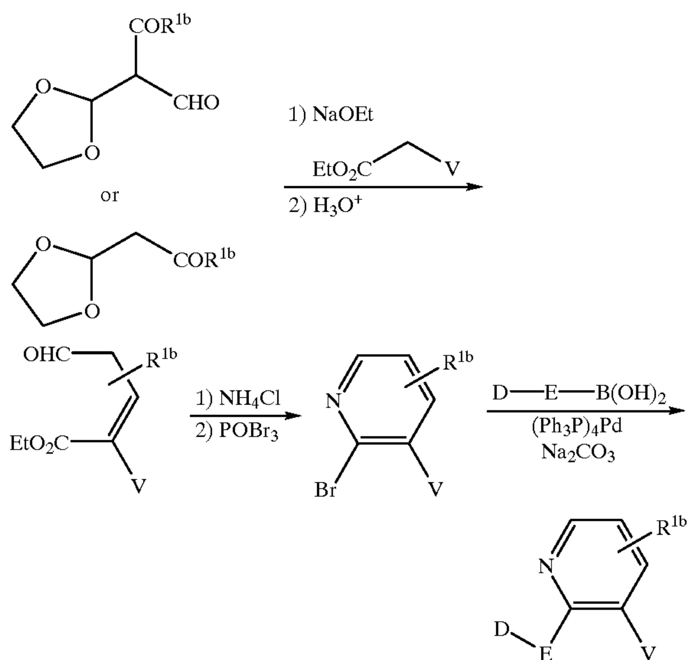
Scheme 42
