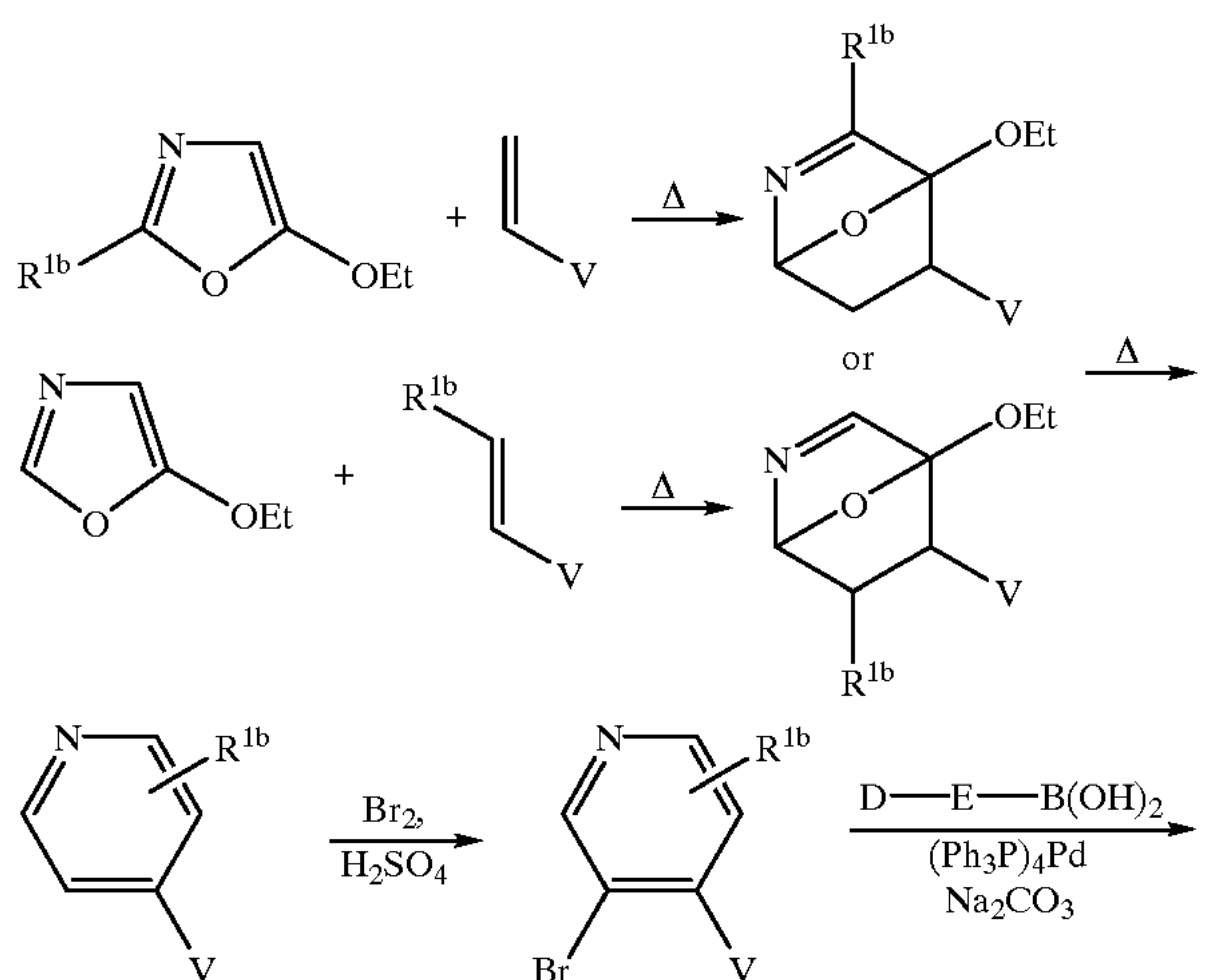
Scheme 43
