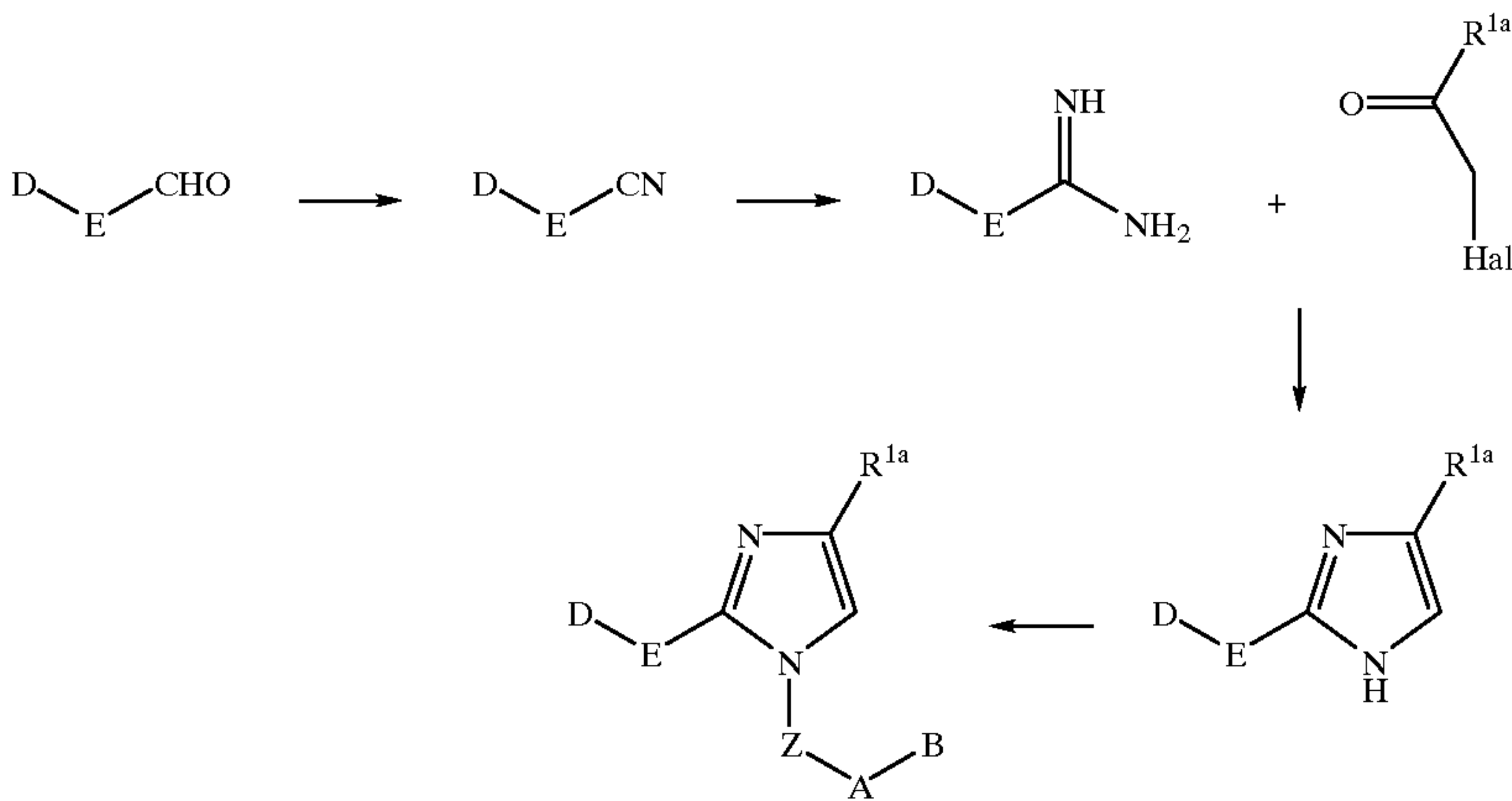
SCHEME 19
