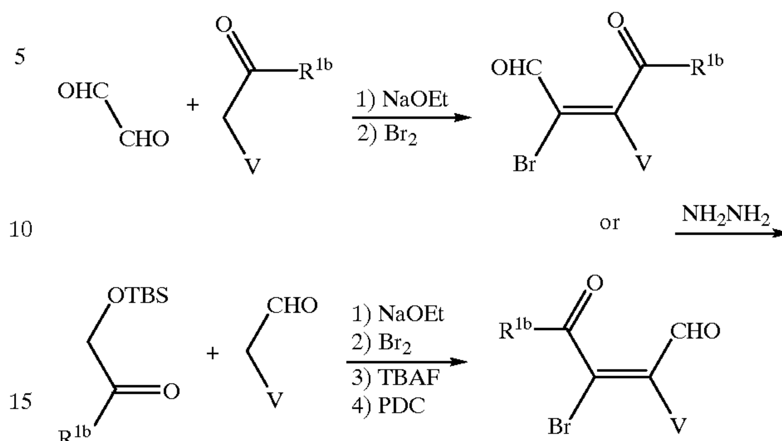
Scheme 47
