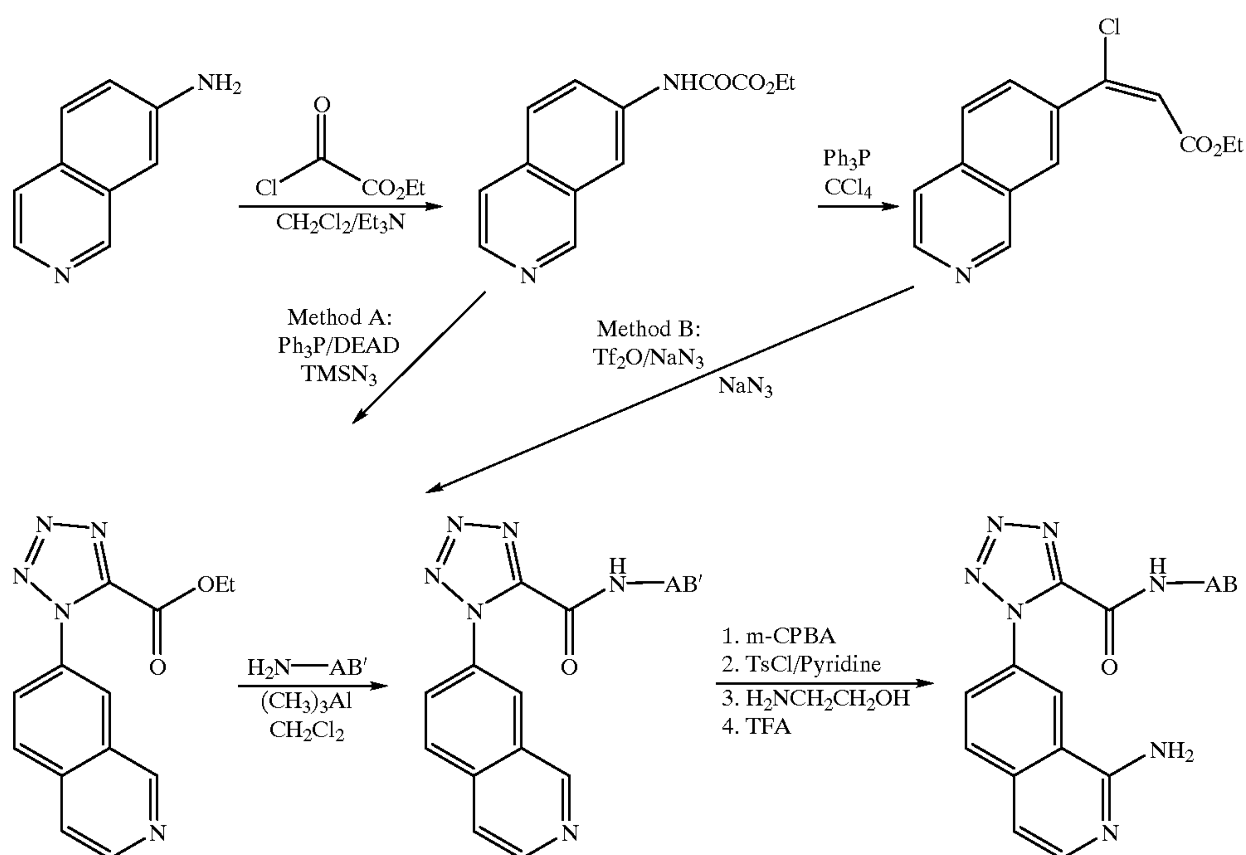
SCHEME 15
