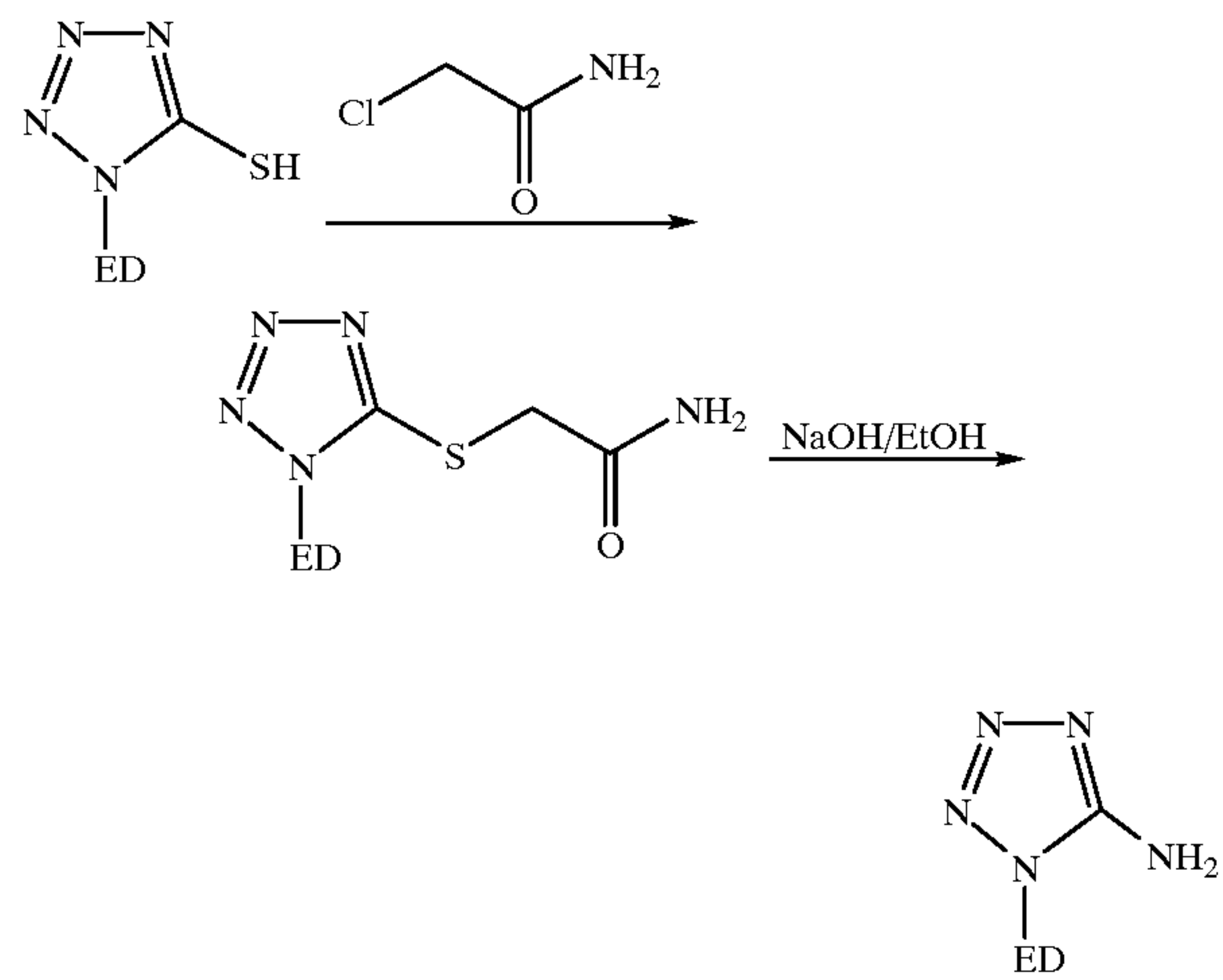
SCHEME 17
