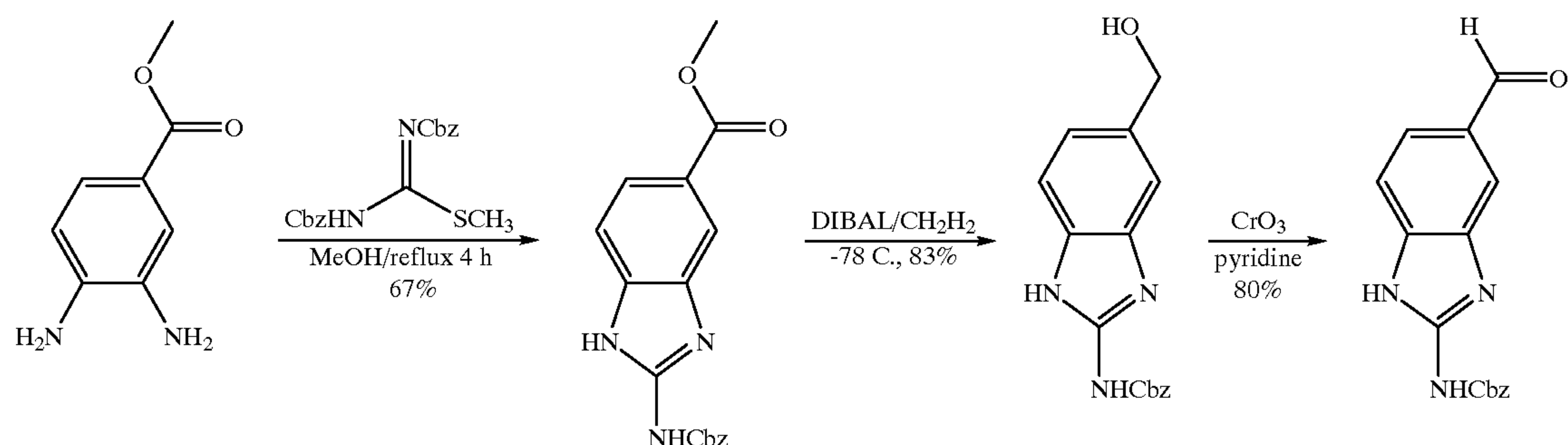
SCHEME 6
