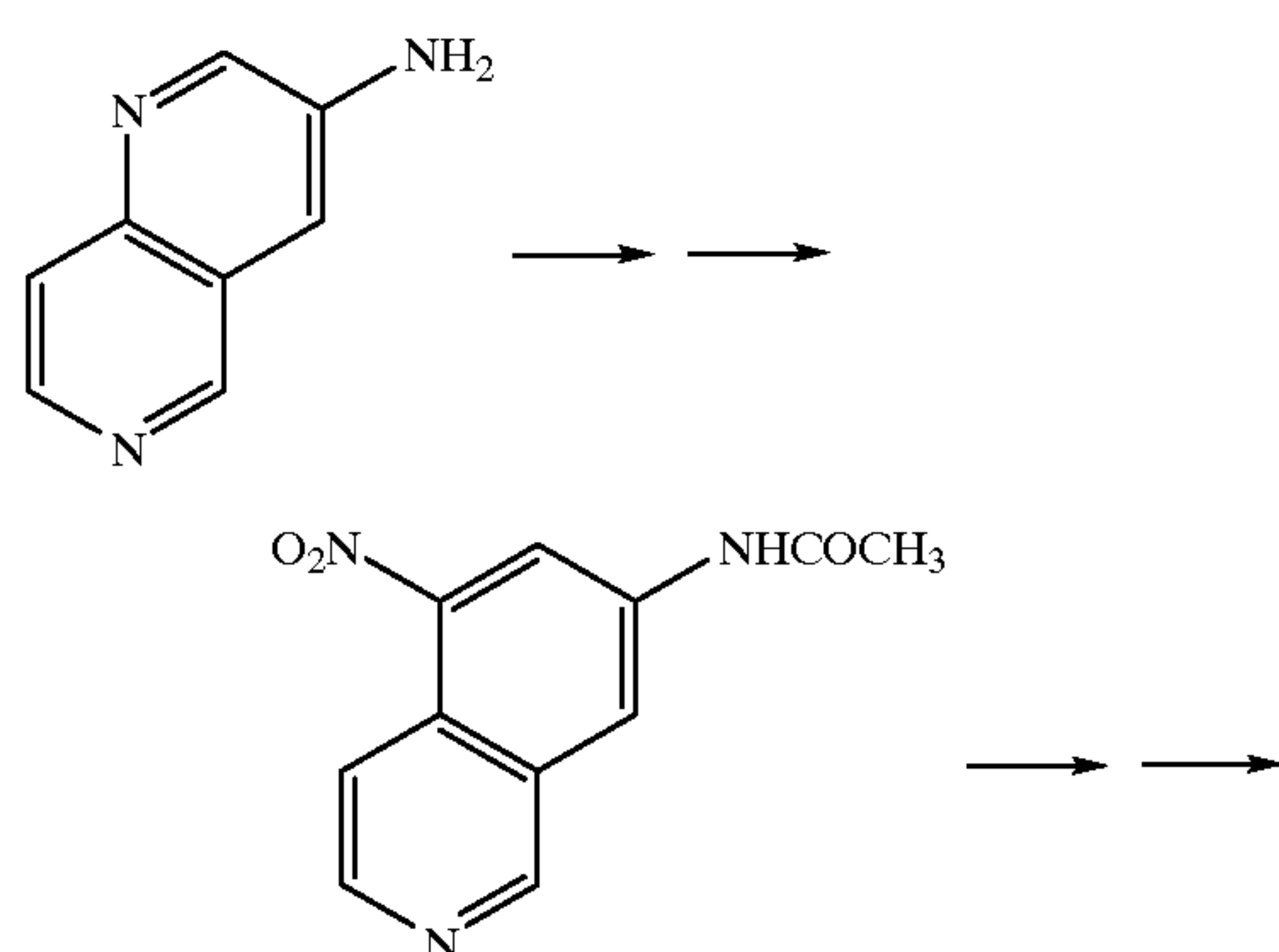
SCHEME 2c
