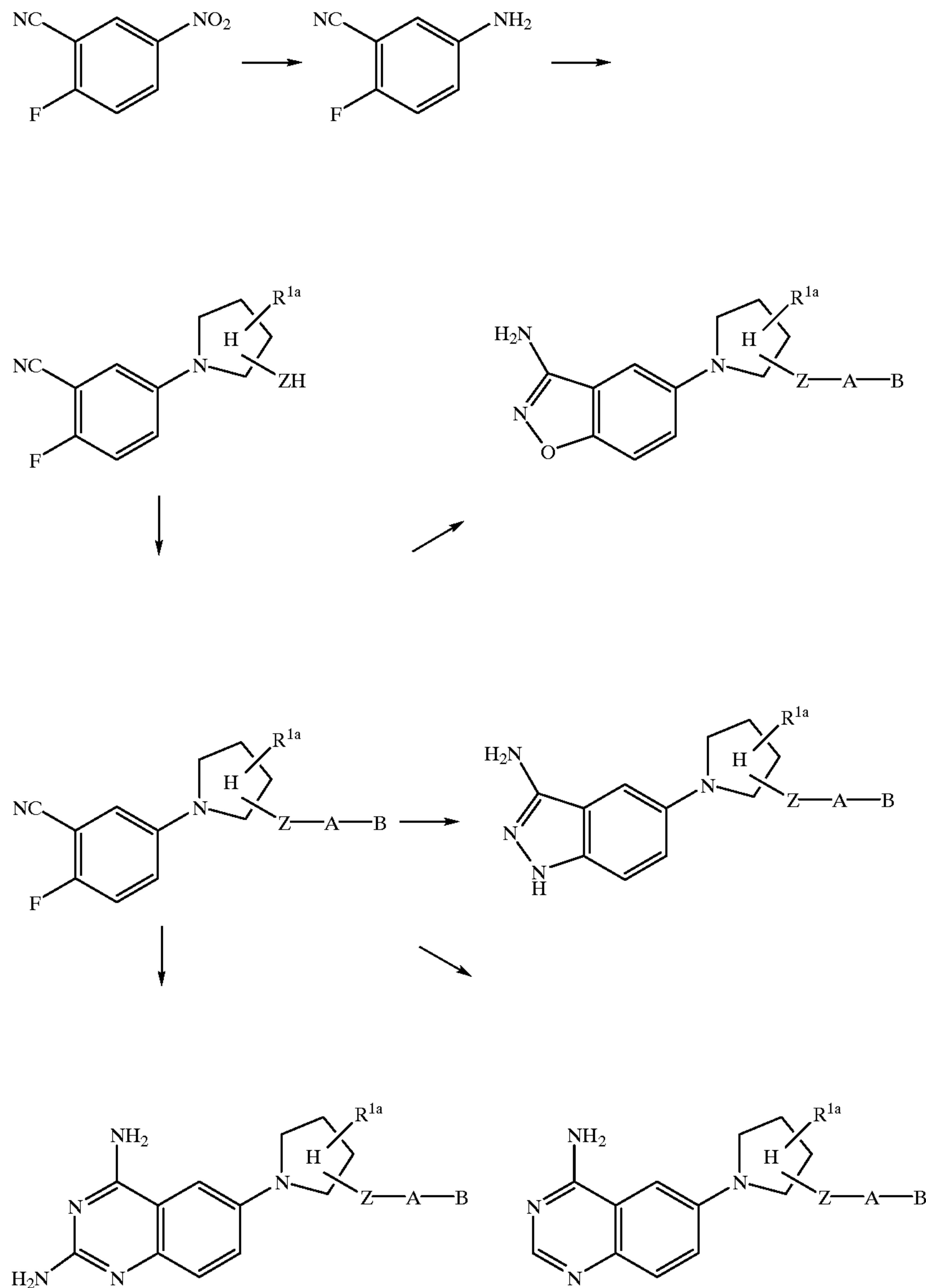
SCHEME 7
