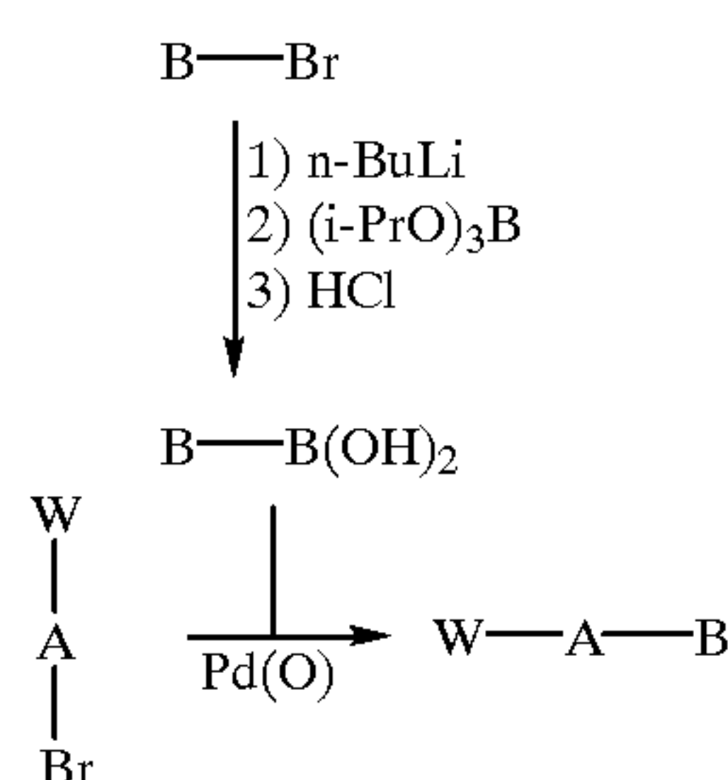
Scheme 57
