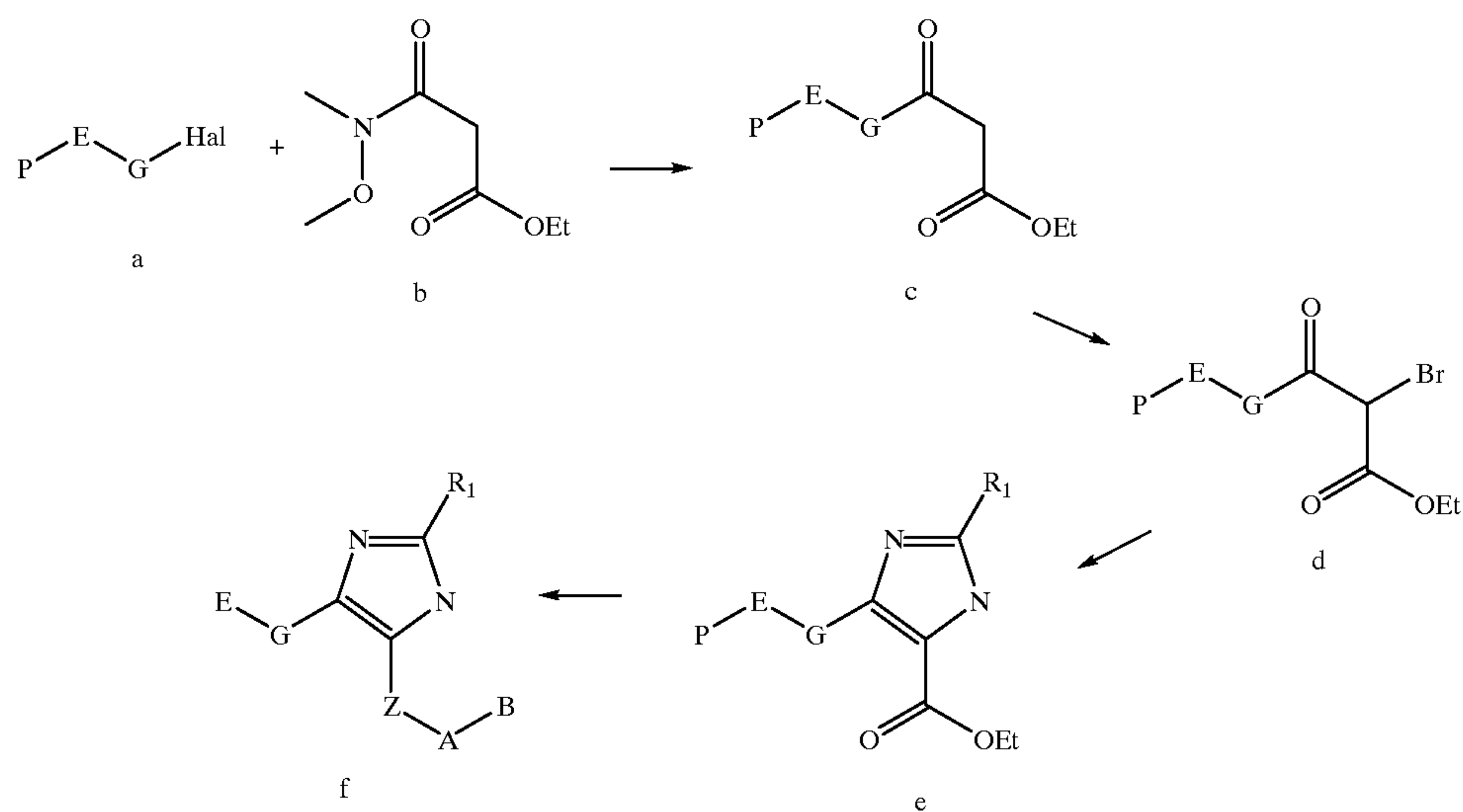
Scheme 18b
