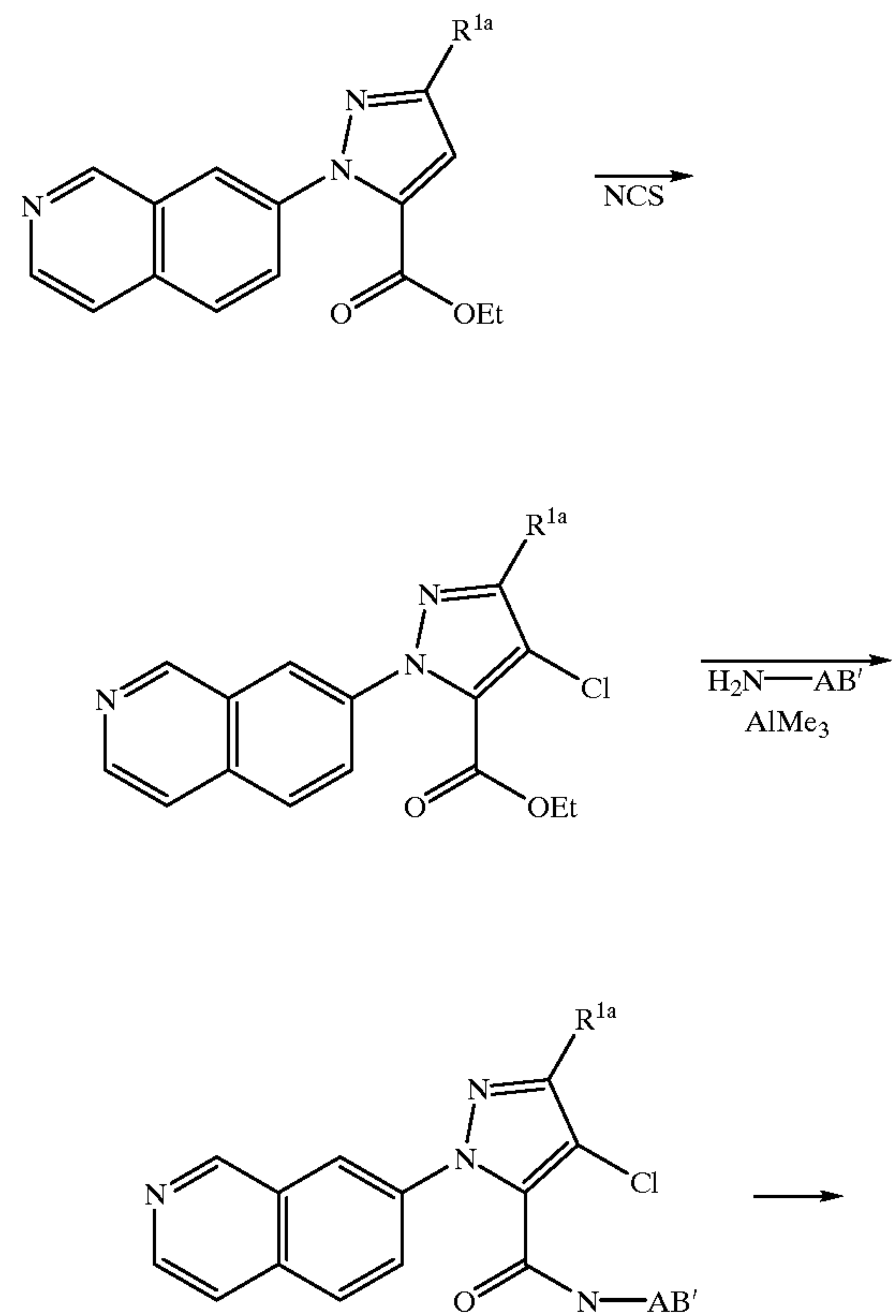
SCHEME 40
