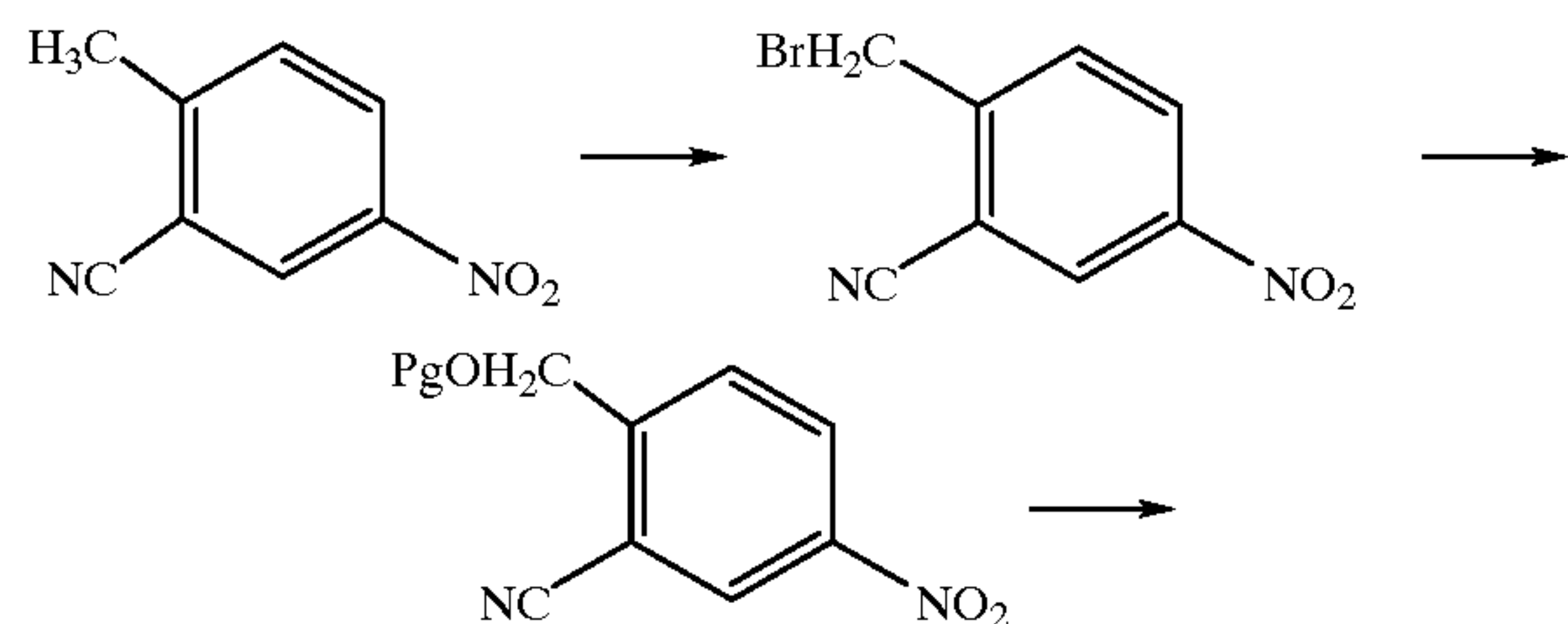
SCHEME 10
