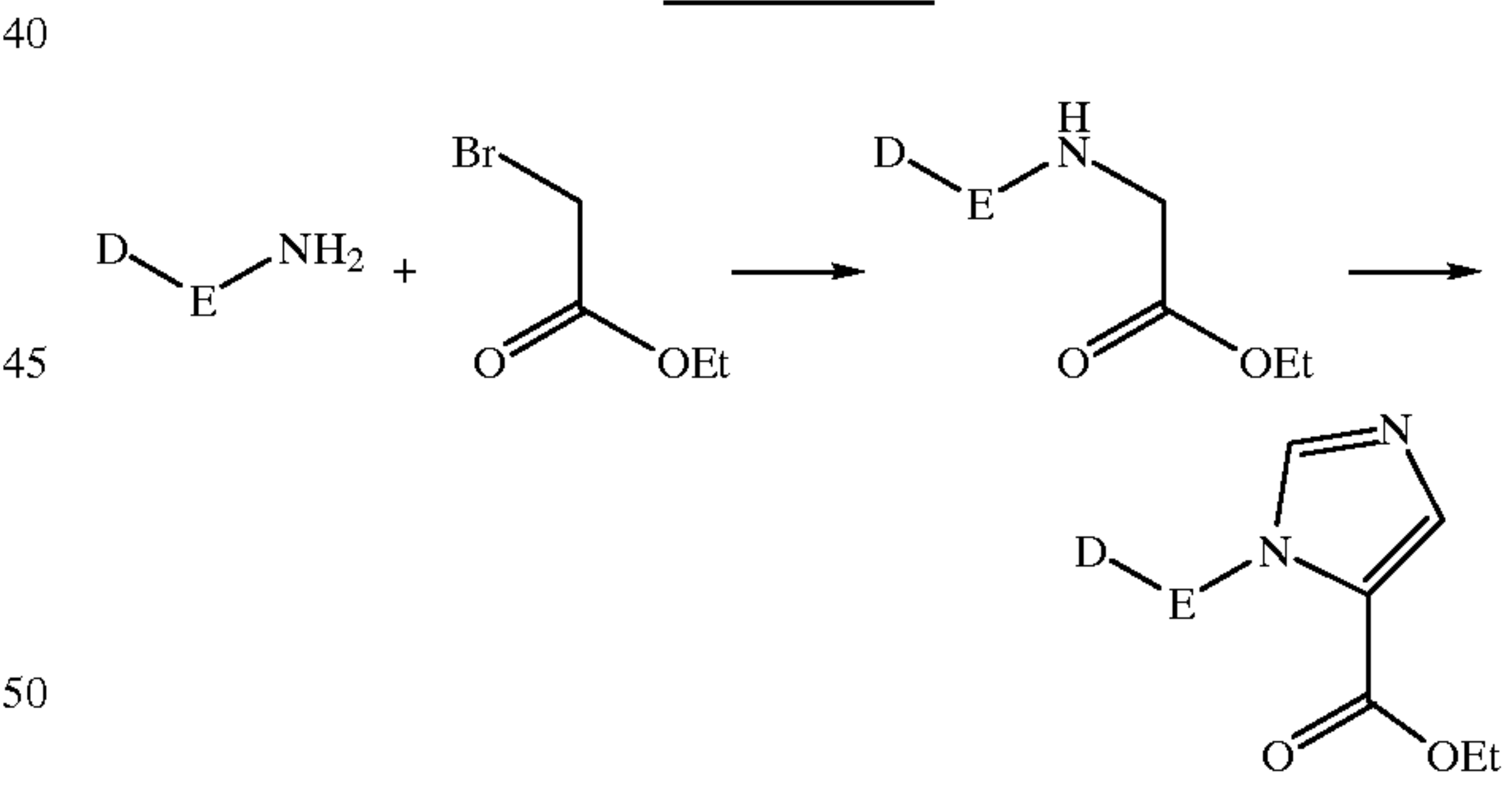
SCHEME 18
