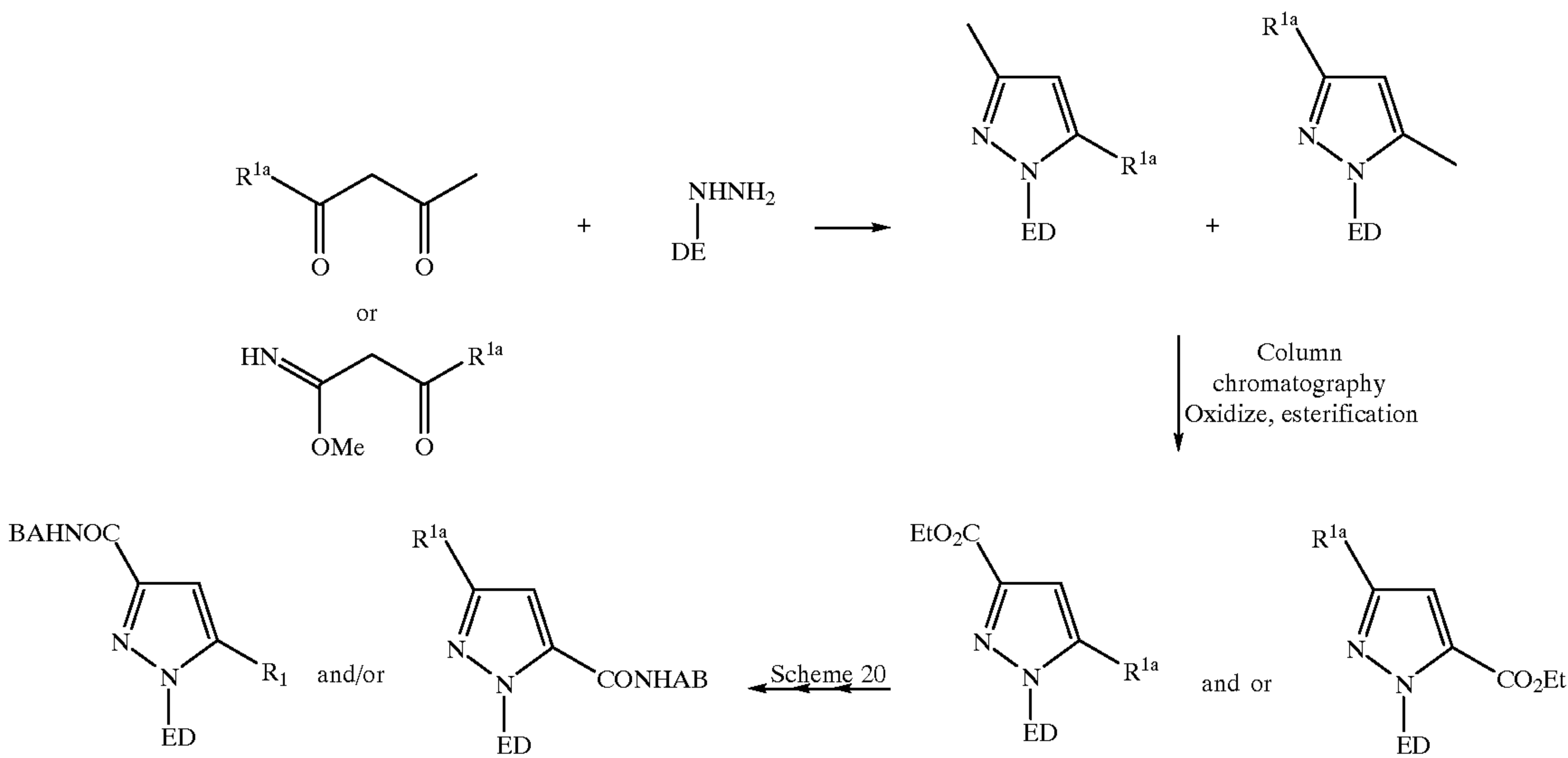
SCHEME 21
