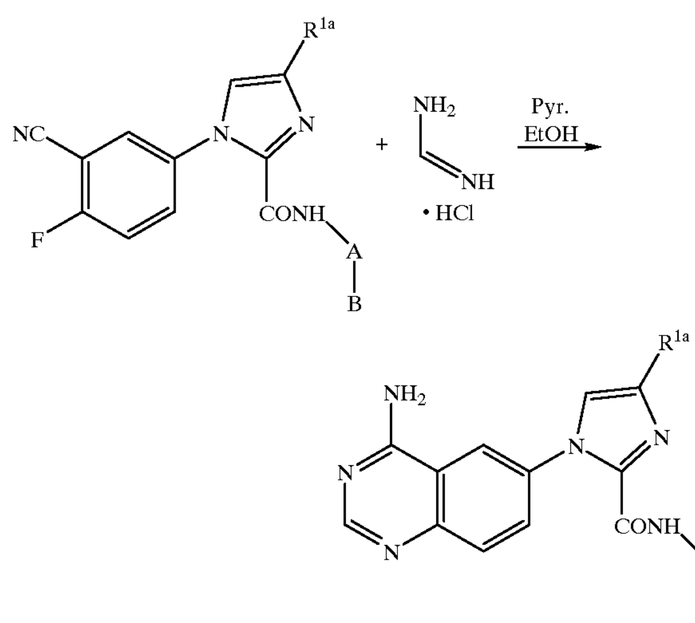
SCHEME 61
