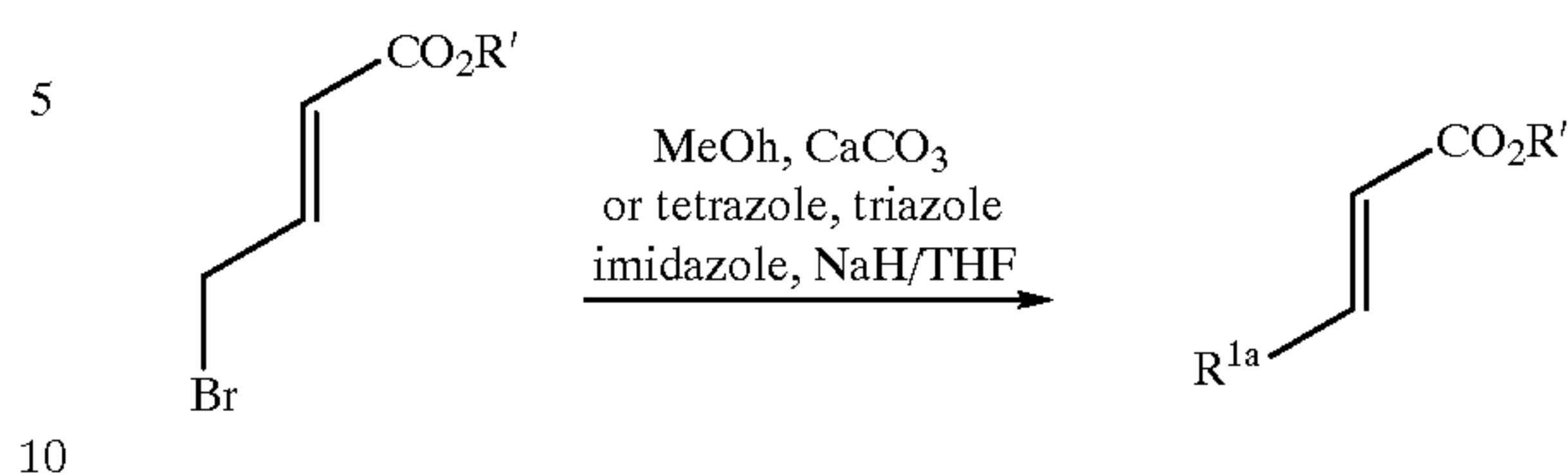
SCHEME 31
