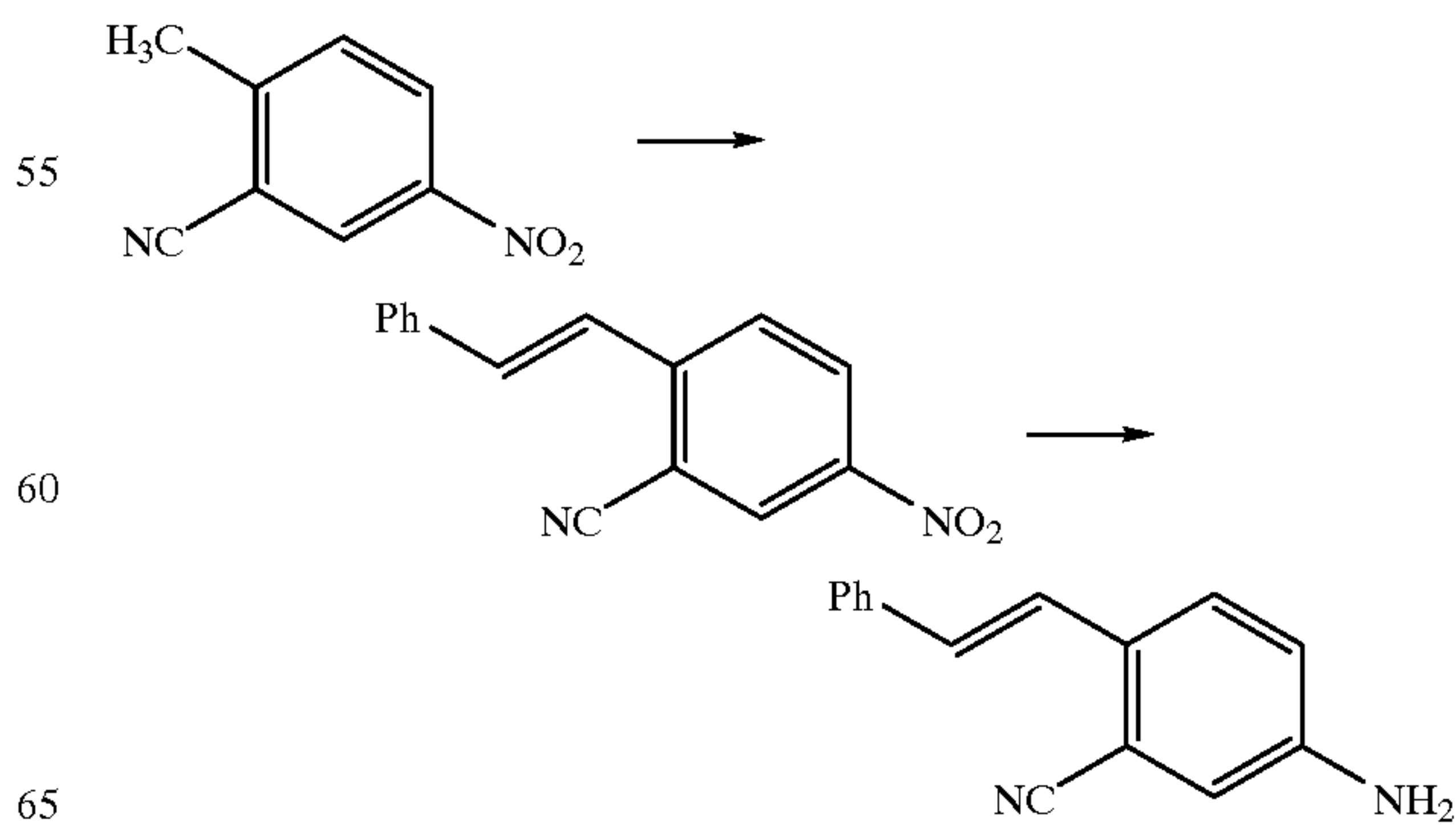
SCHEME 8
