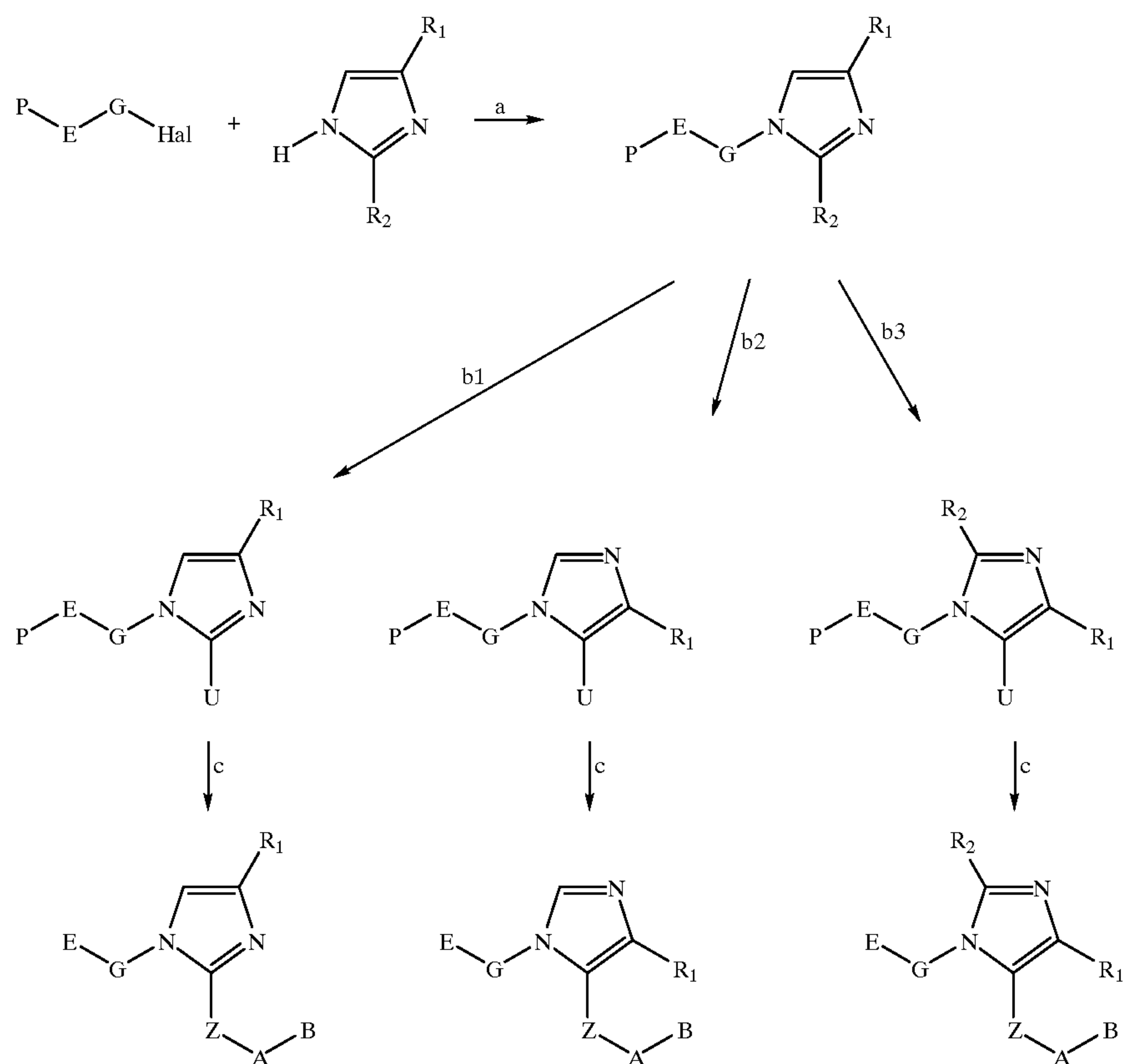
SCHEME 18a
