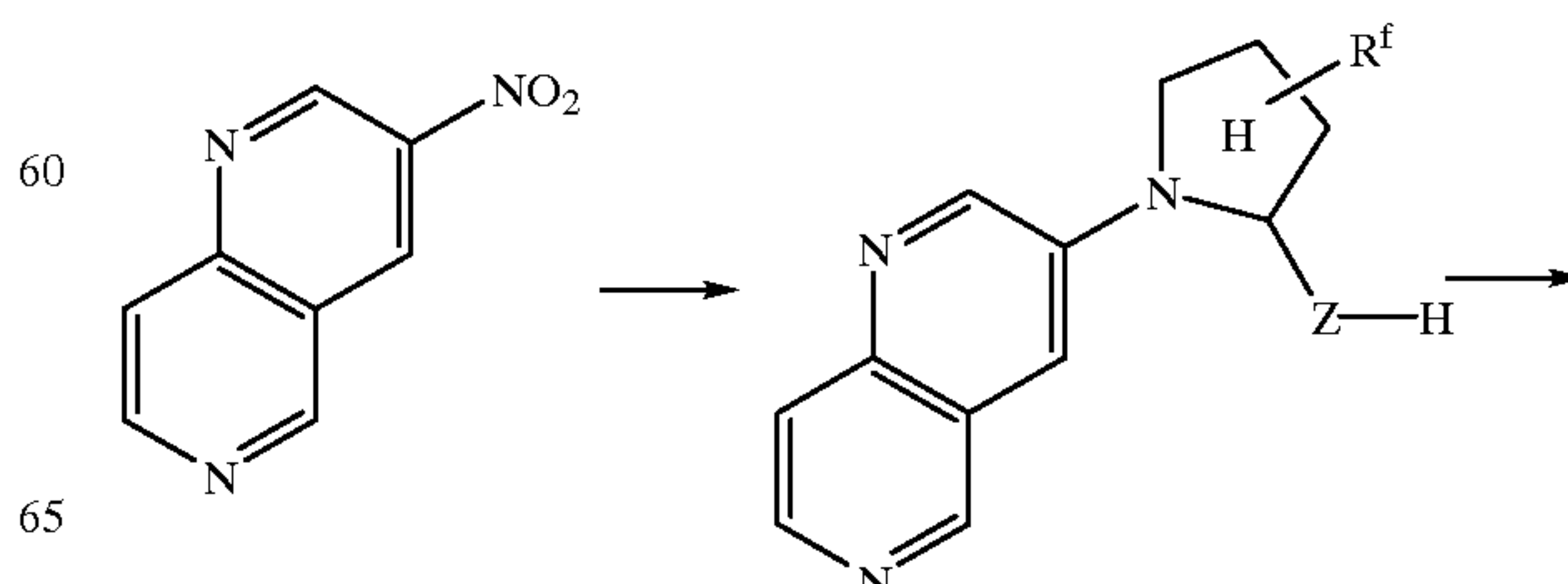
SCHEME 2b
