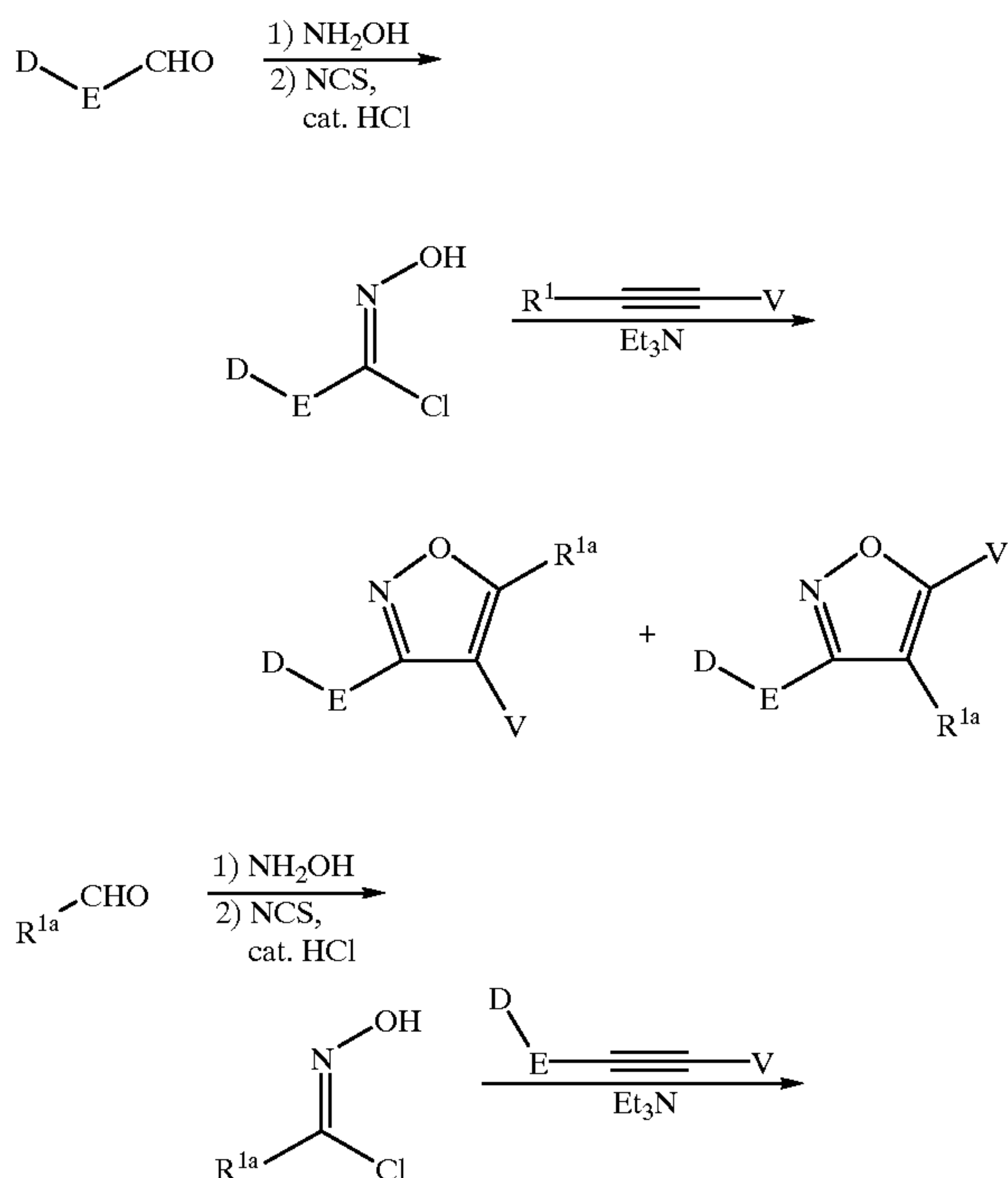
SCHEME 36
