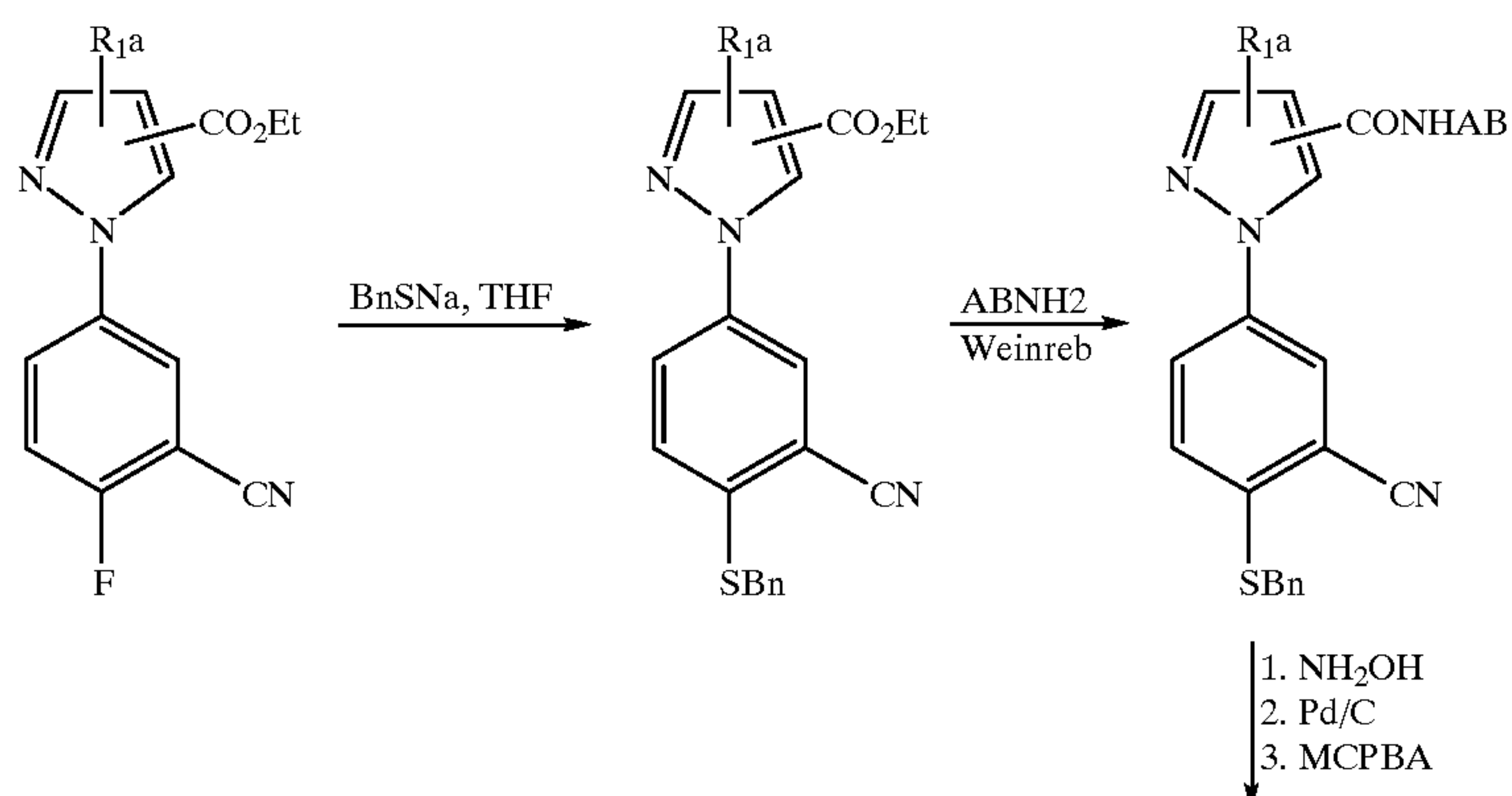
SCHEME 13
