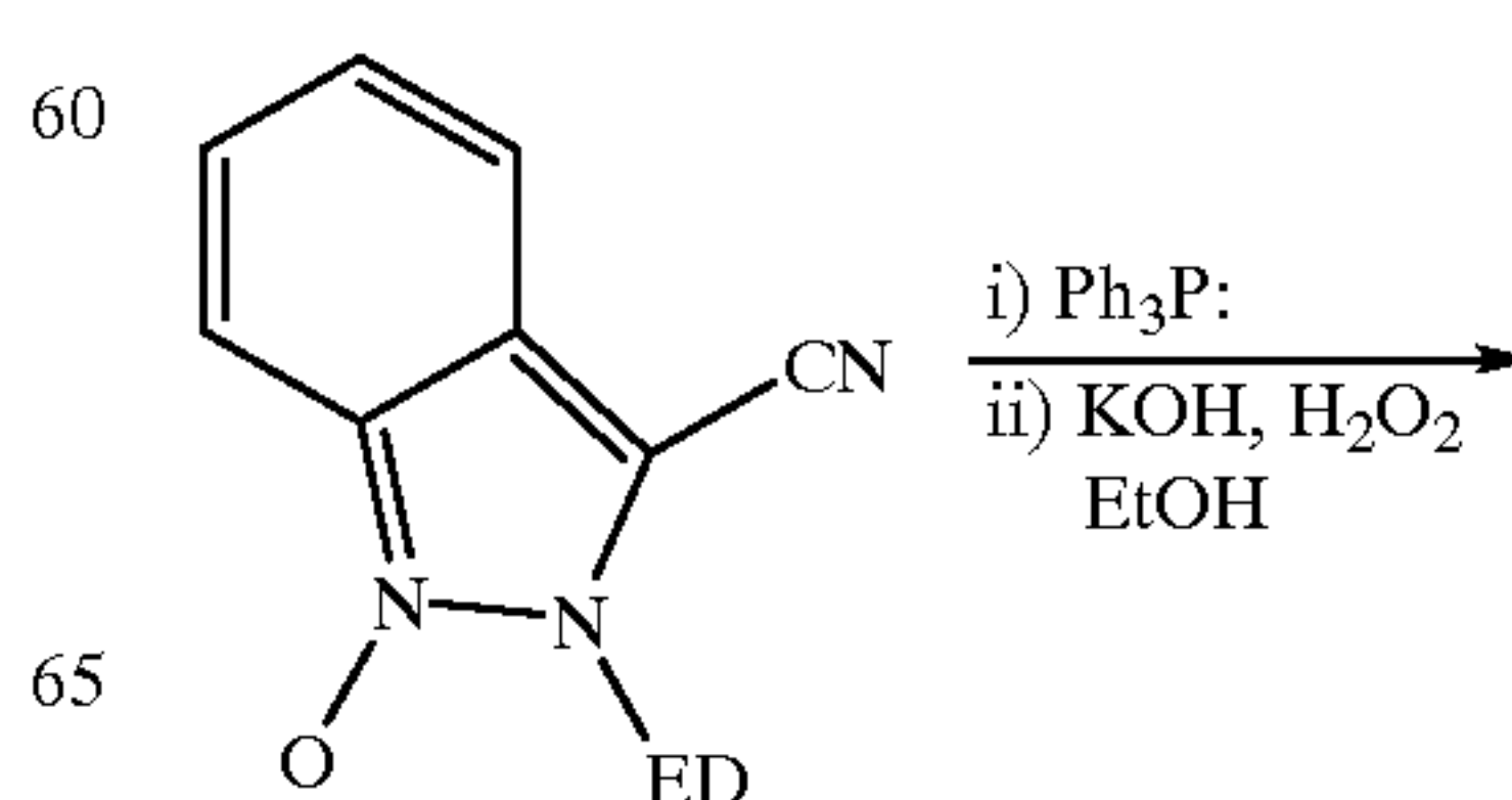
SCHEME 62
