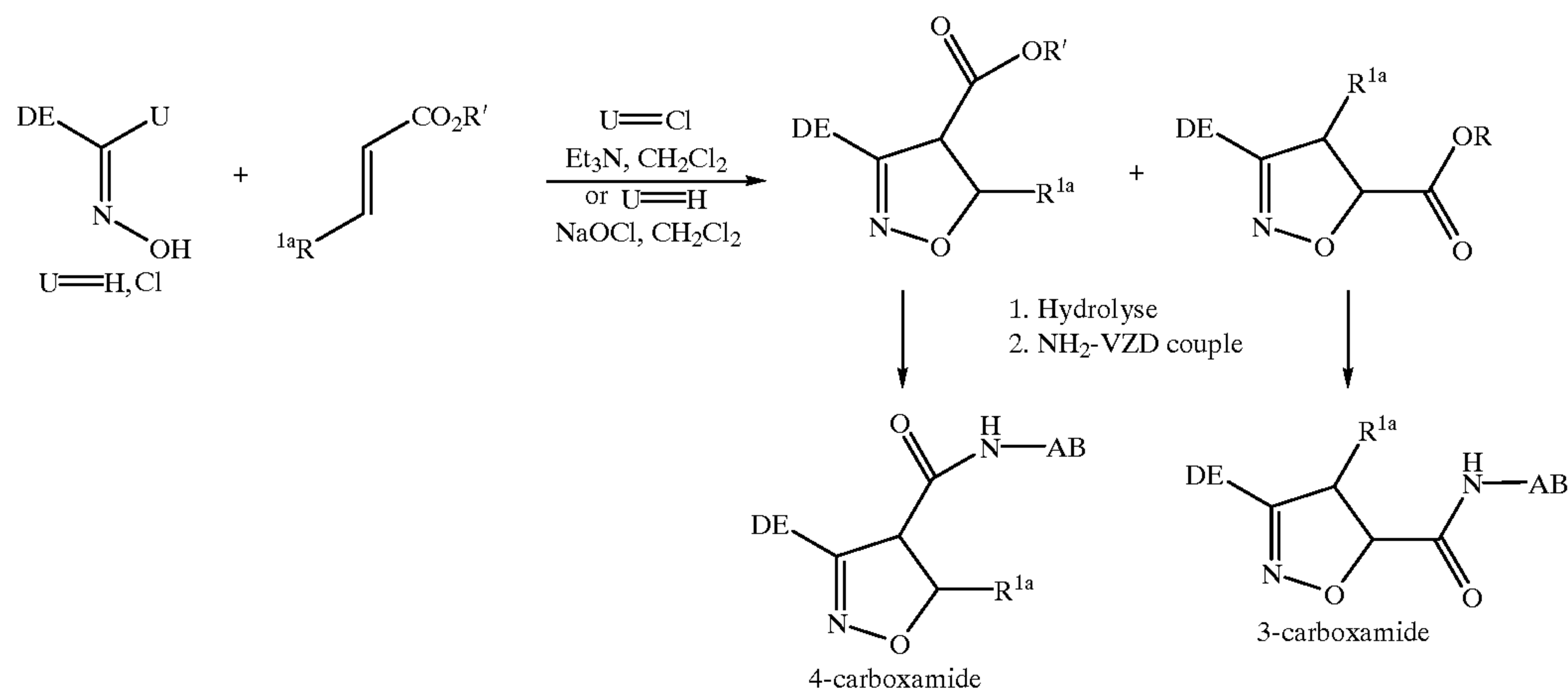
SCHEME 30
