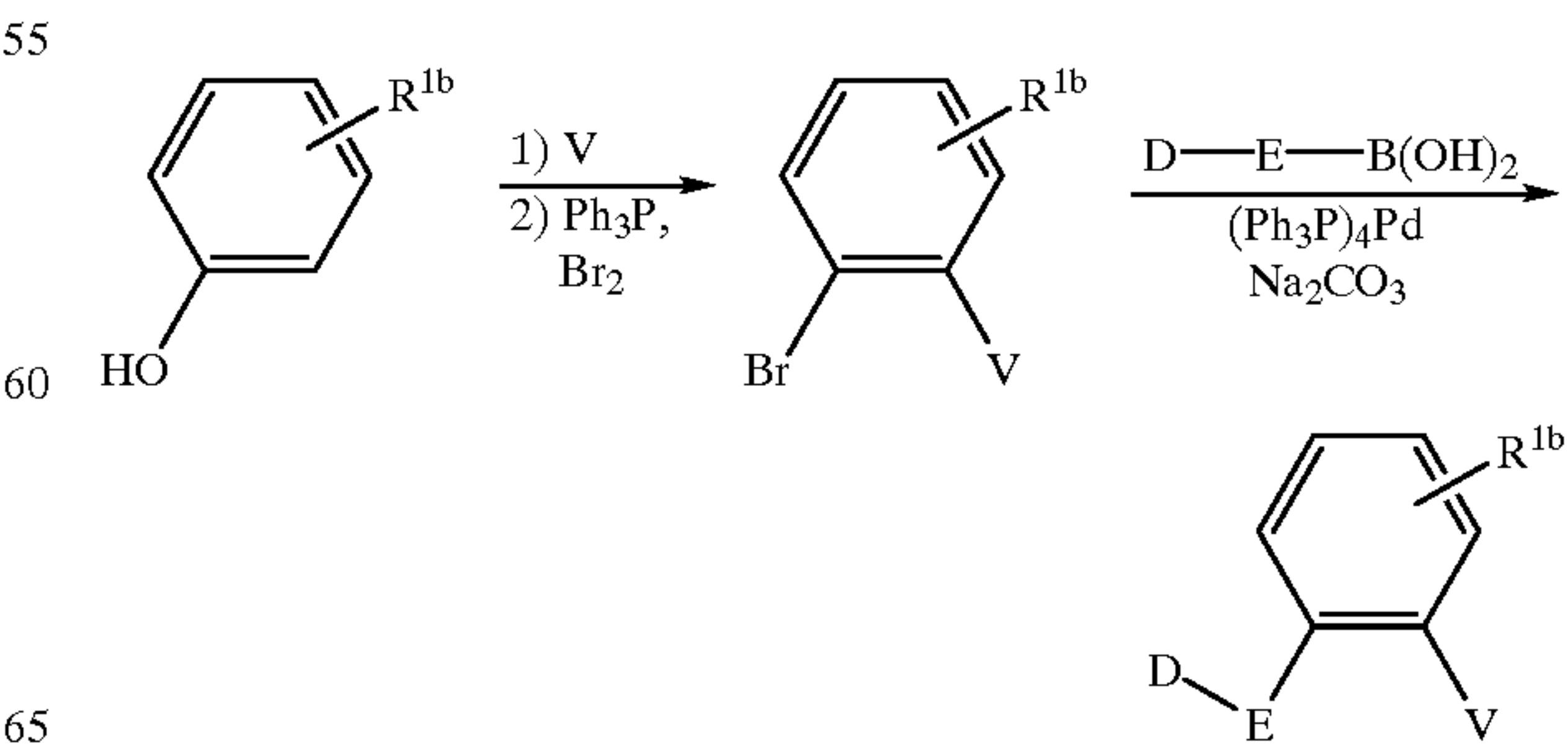
Scheme 41
