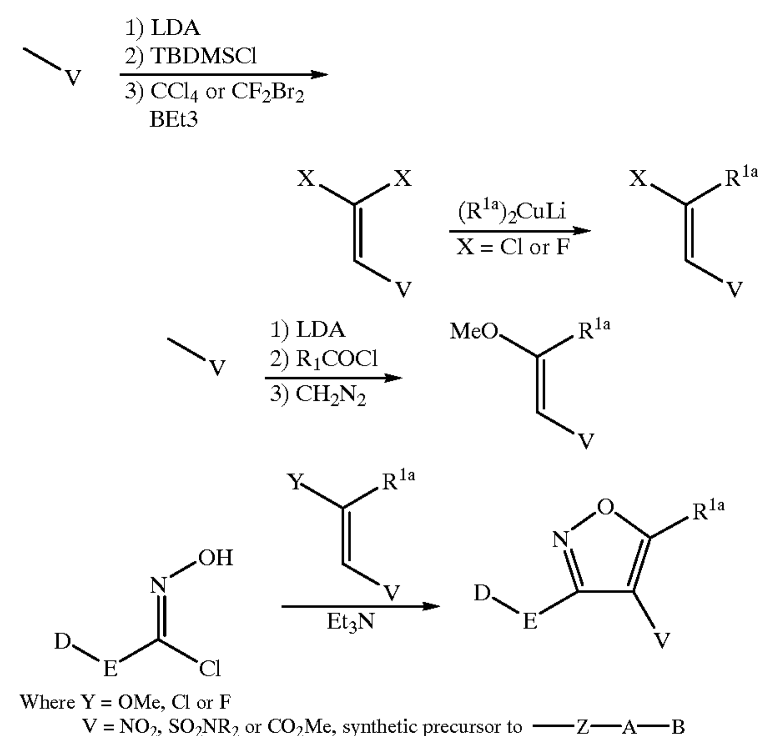
SCHEME 37
