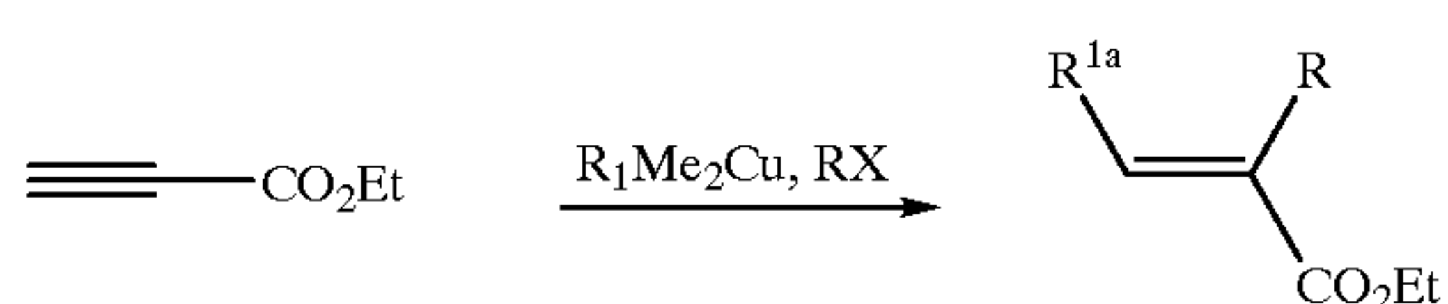
SCHEME 32
