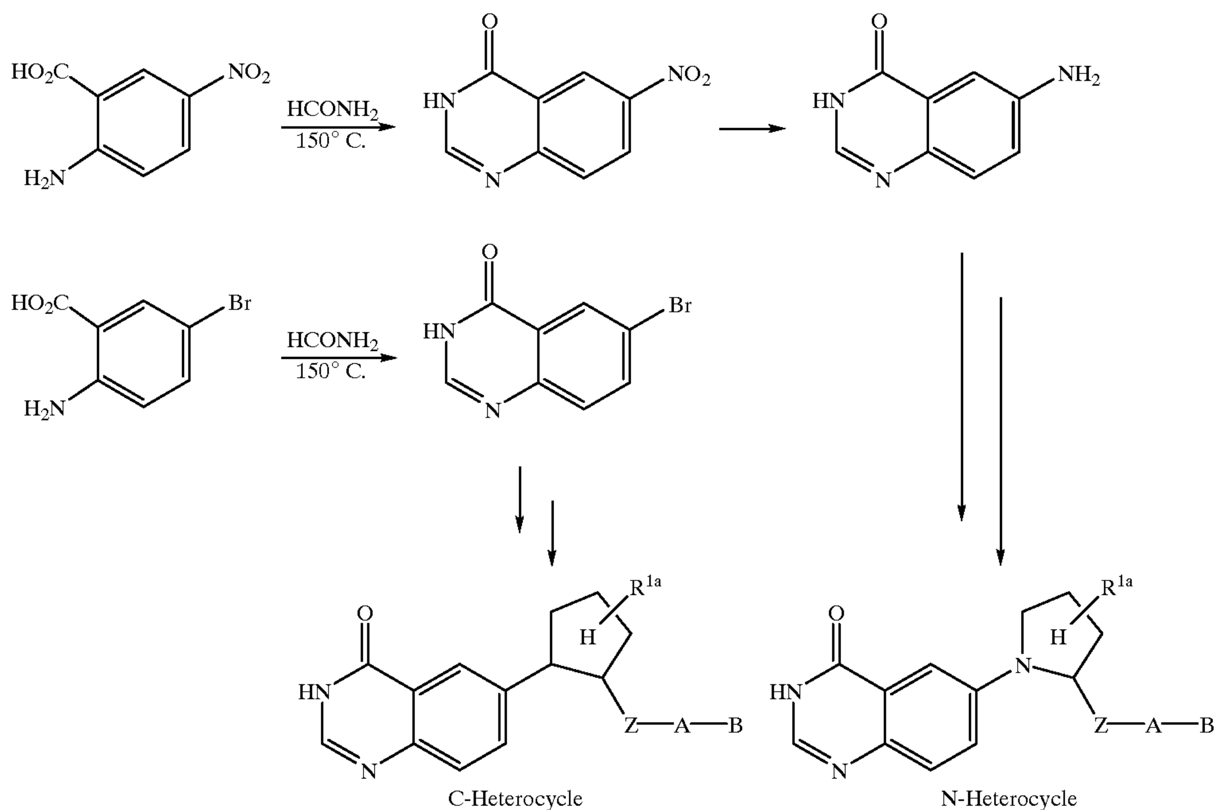
SCHEME 11
