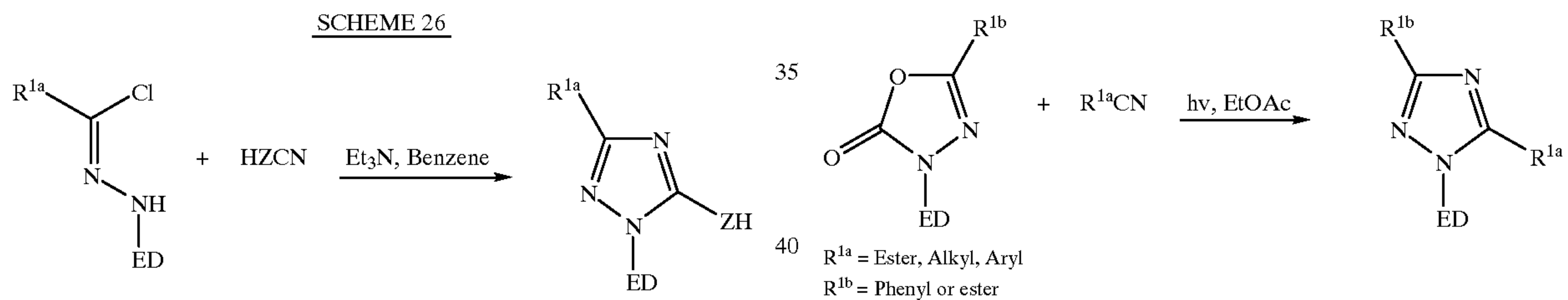
SCHEME 28
