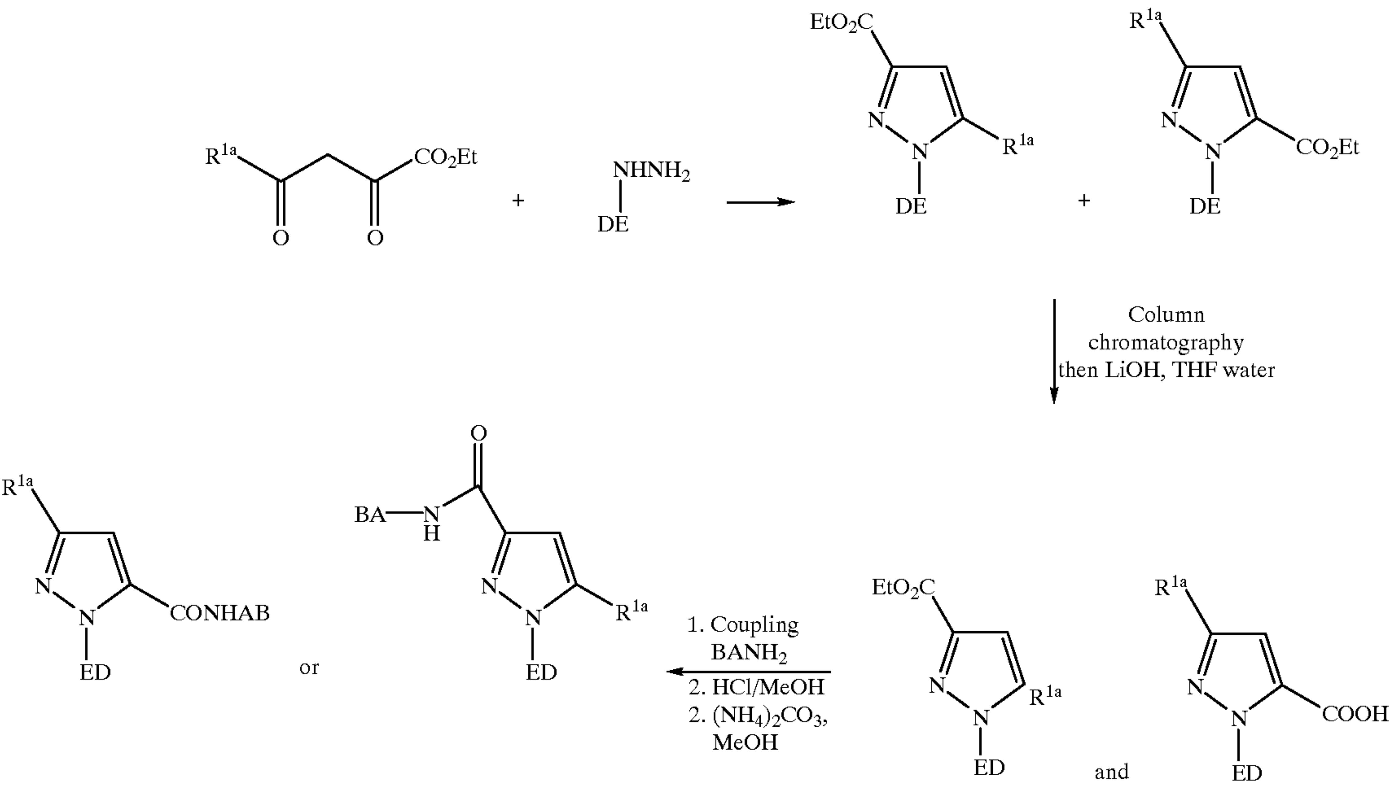
SCHEME 20
