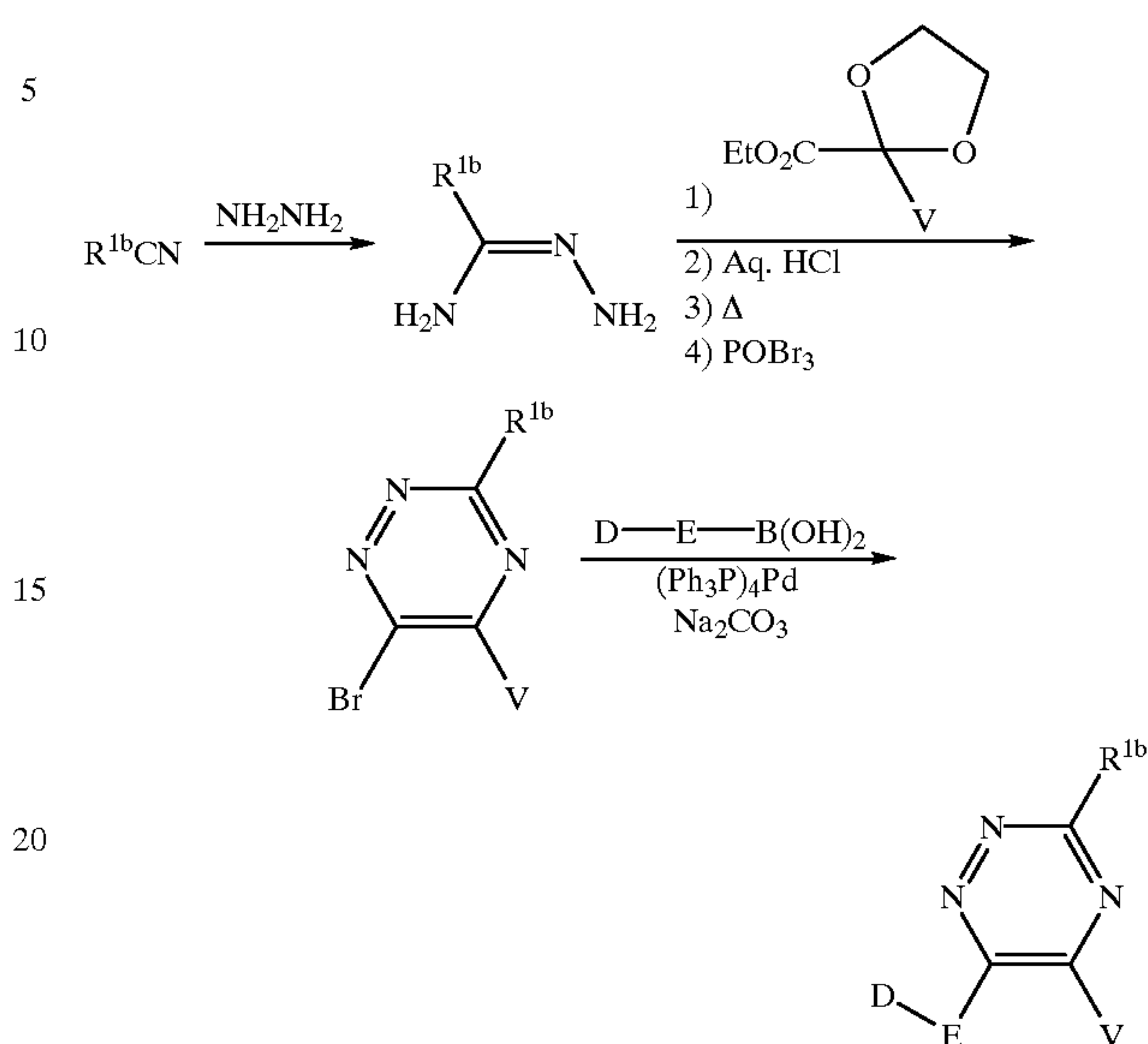
Scheme 55
