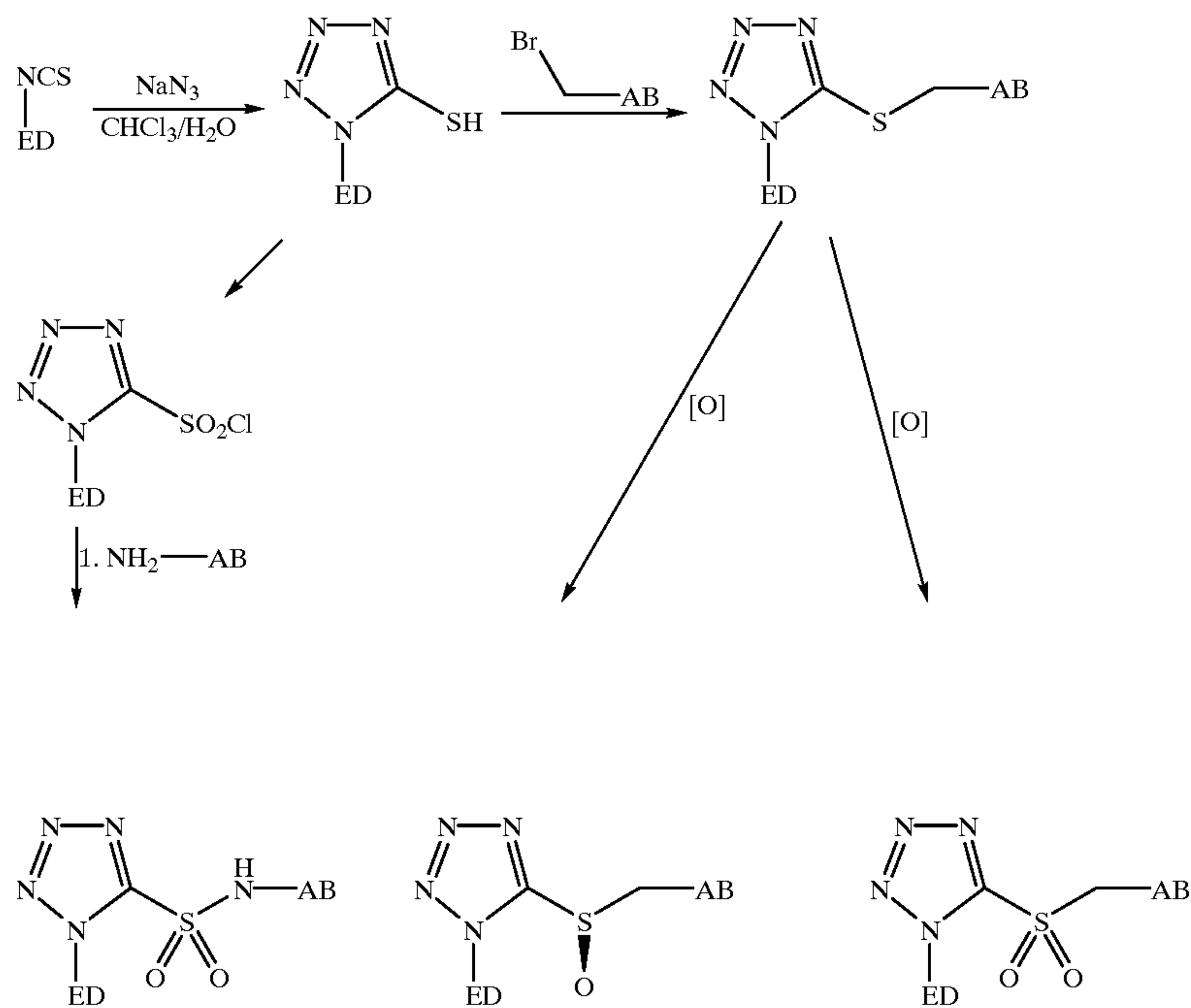
SCHEME 16
