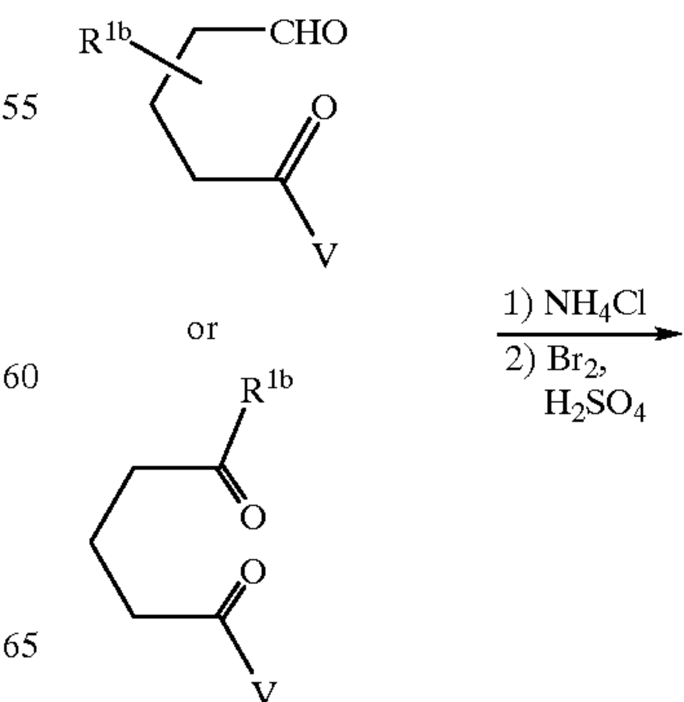
Scheme 45
