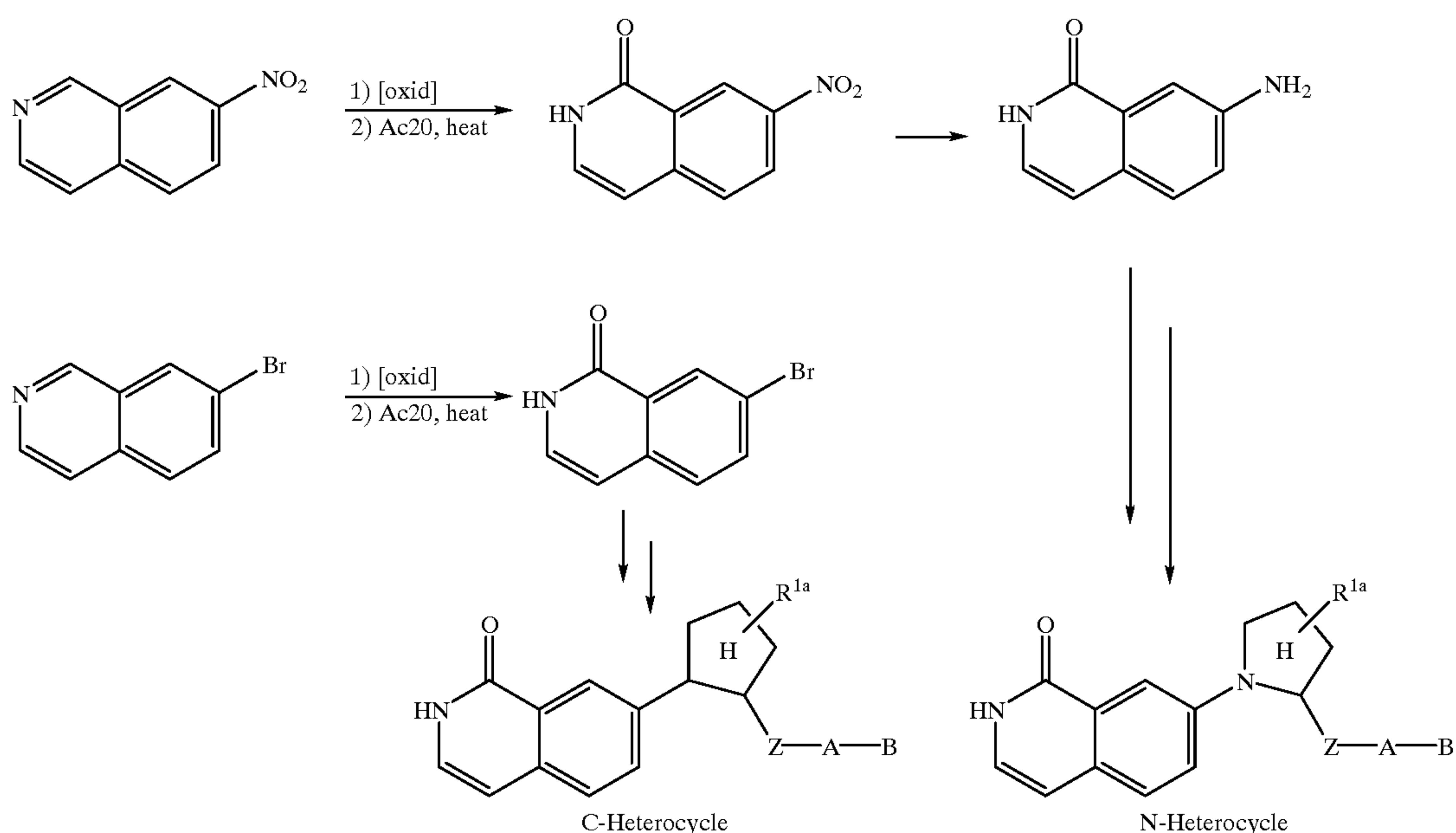
SCHEME 12
