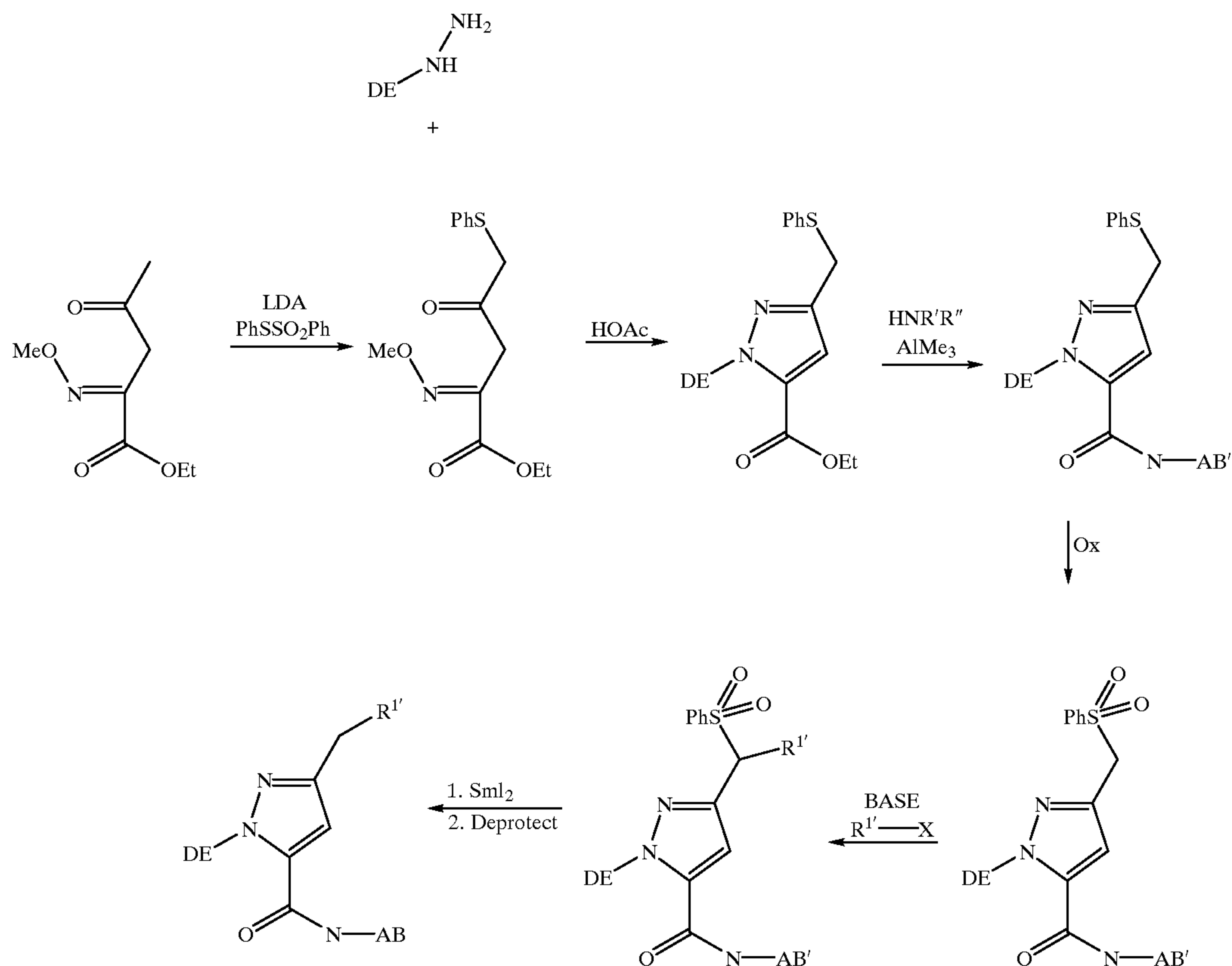
SCHEME 38
