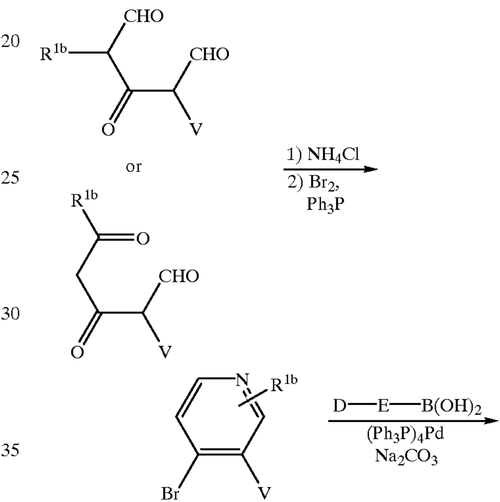
Scheme 44
