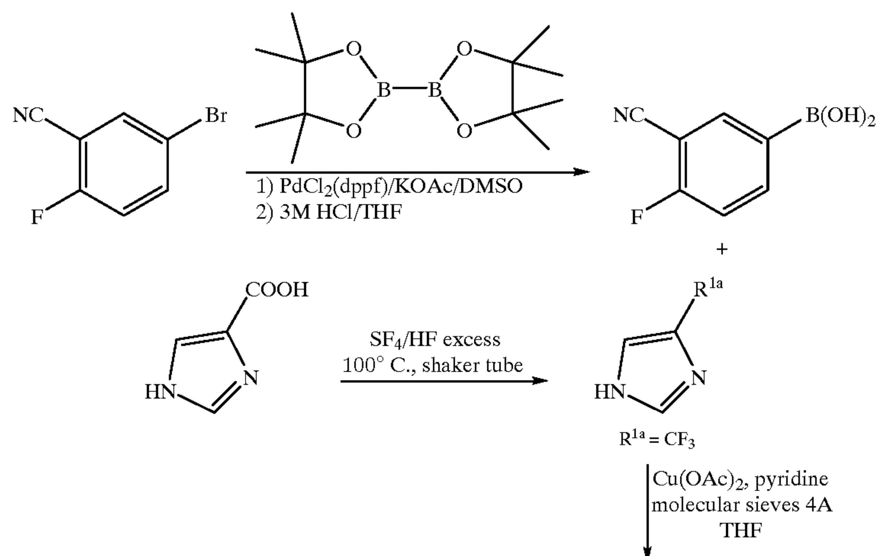
SCHEME 60
