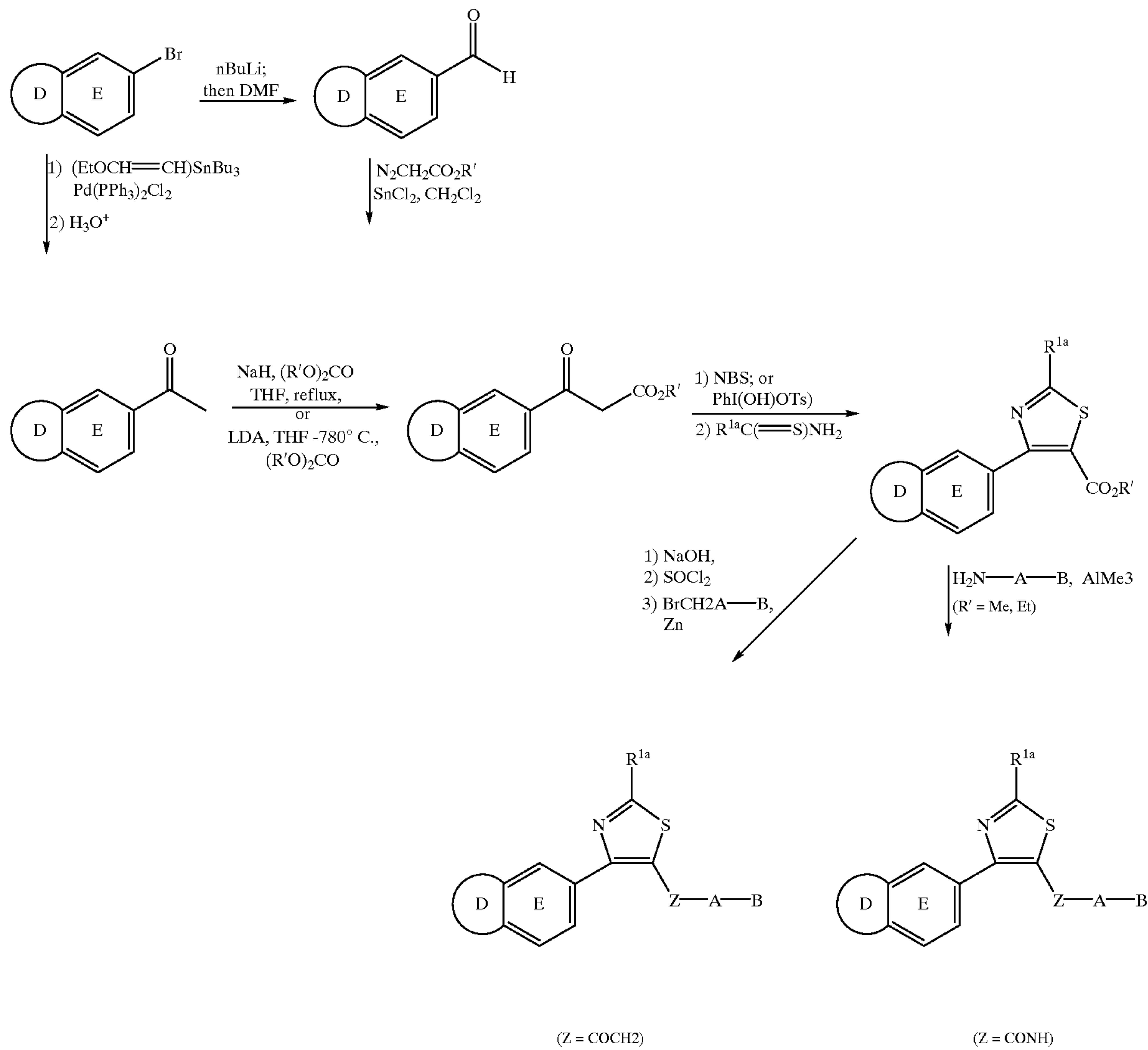
SCHEME 14
