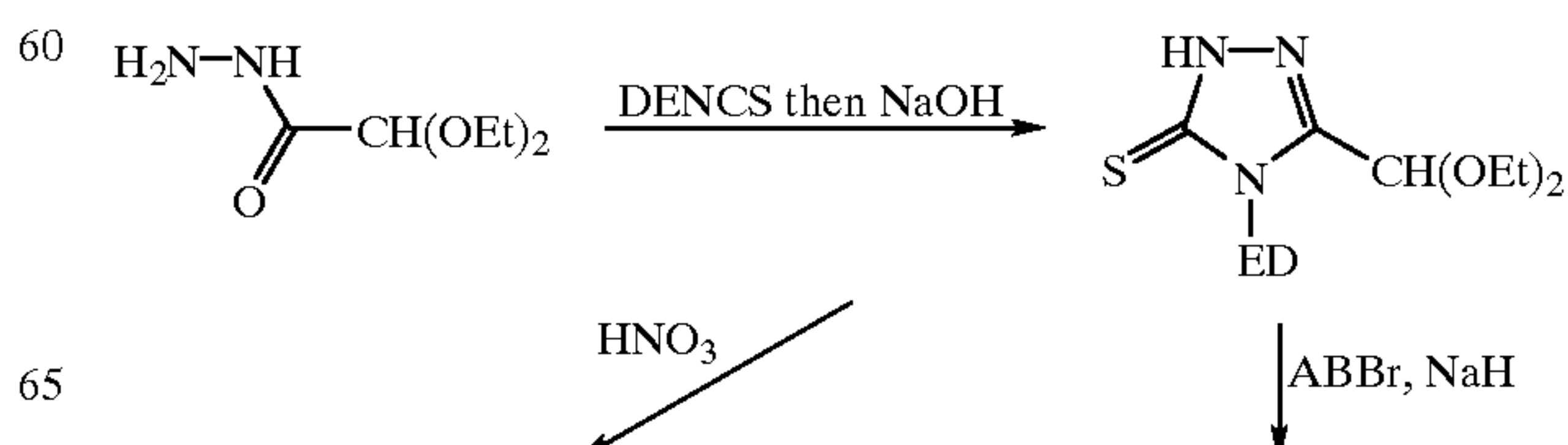
SCHEME 33
