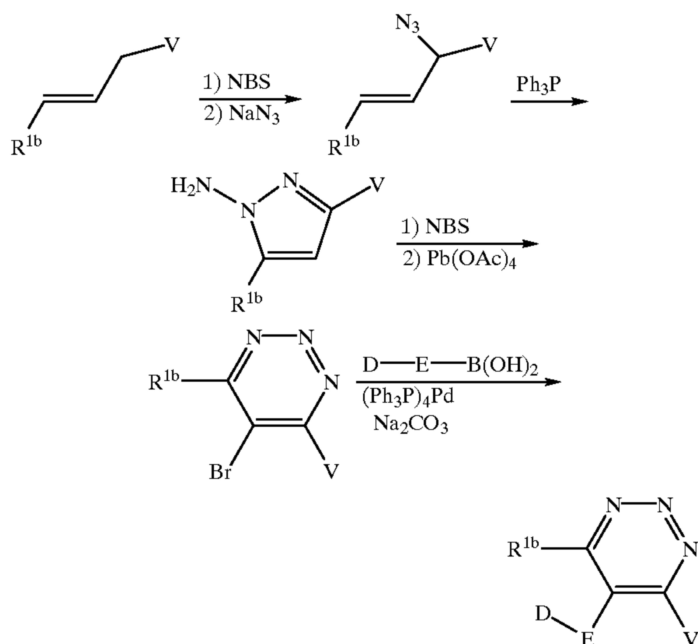
Scheme 53
