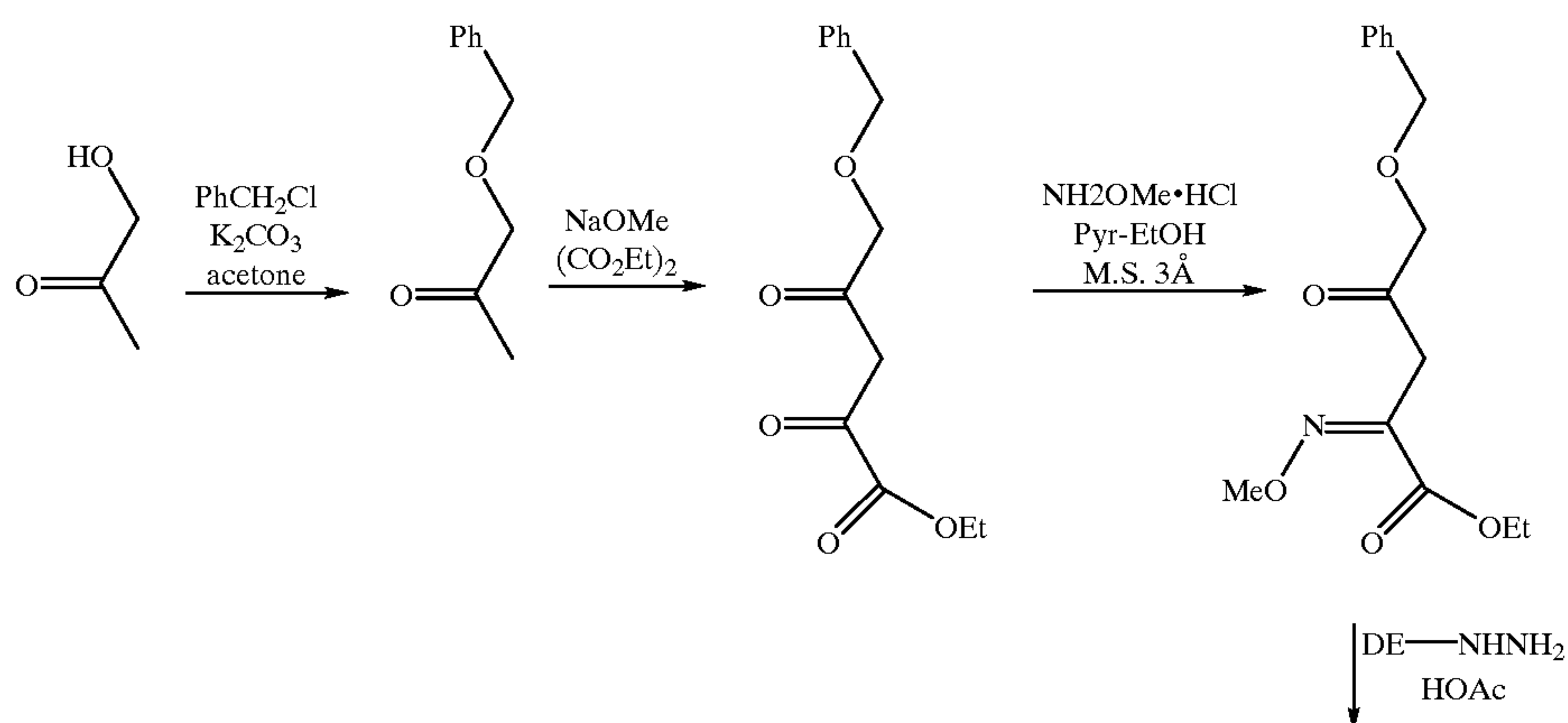
SCHEME 39
