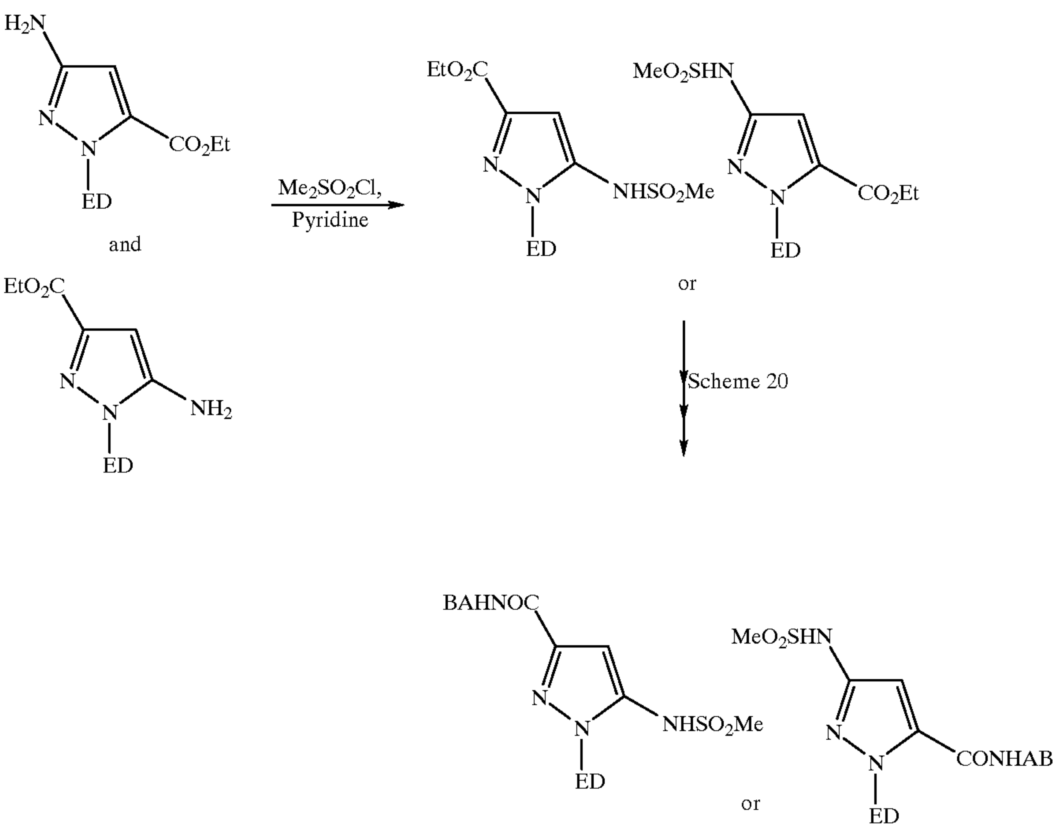
SCHEME 22
