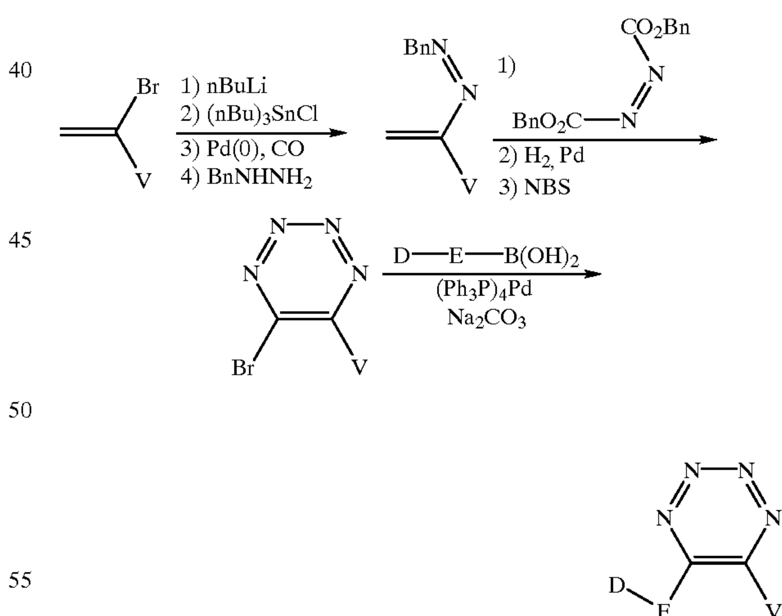
Scheme 56
