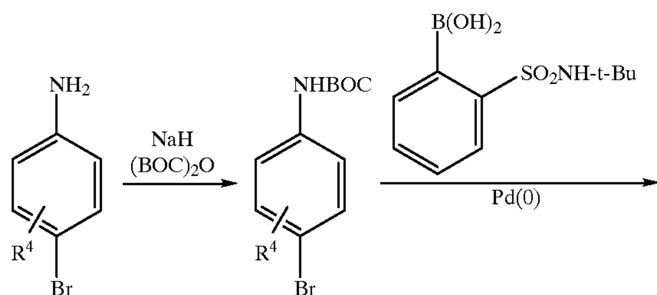
Scheme 58
