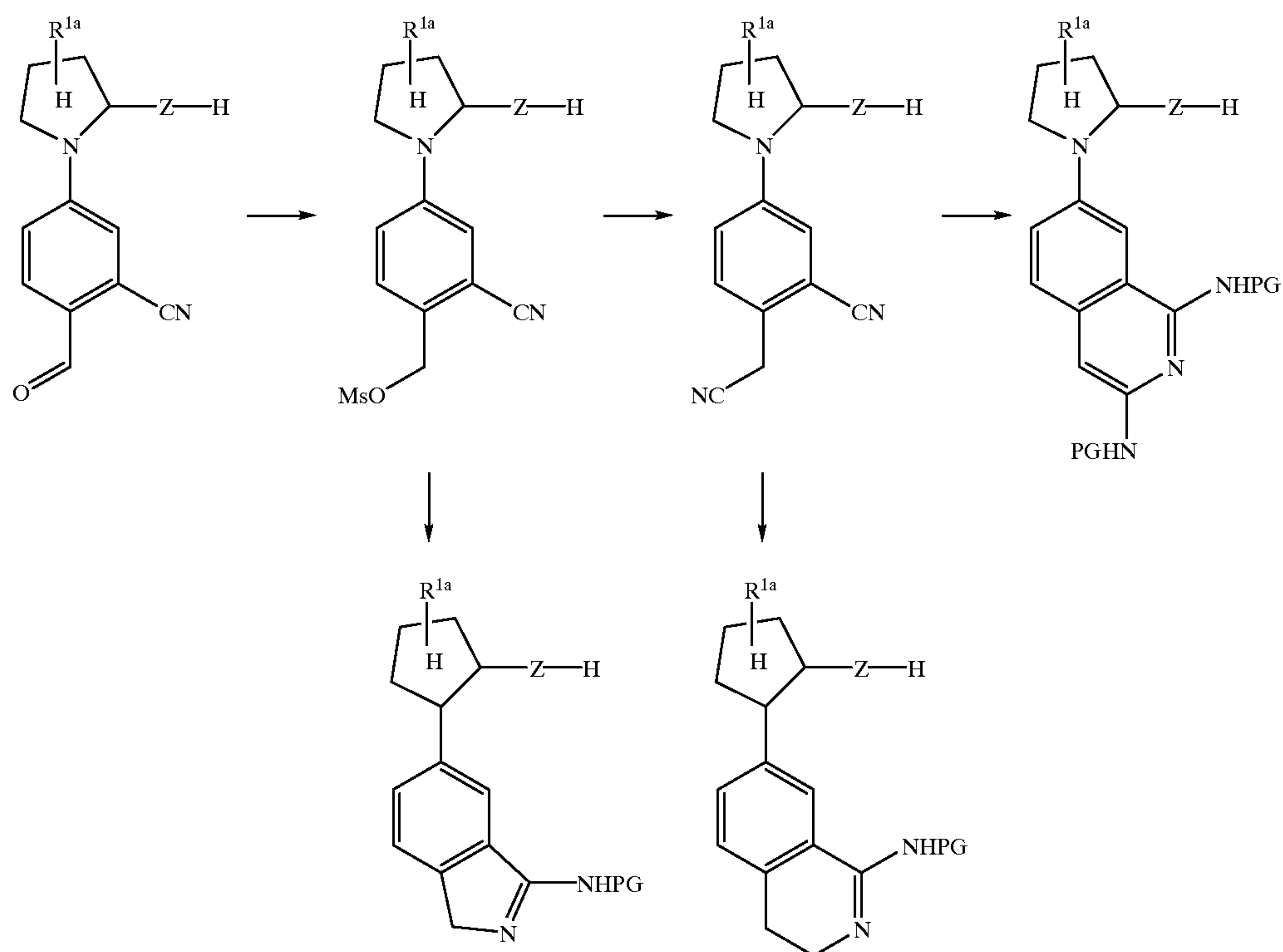
SCHEME 9
