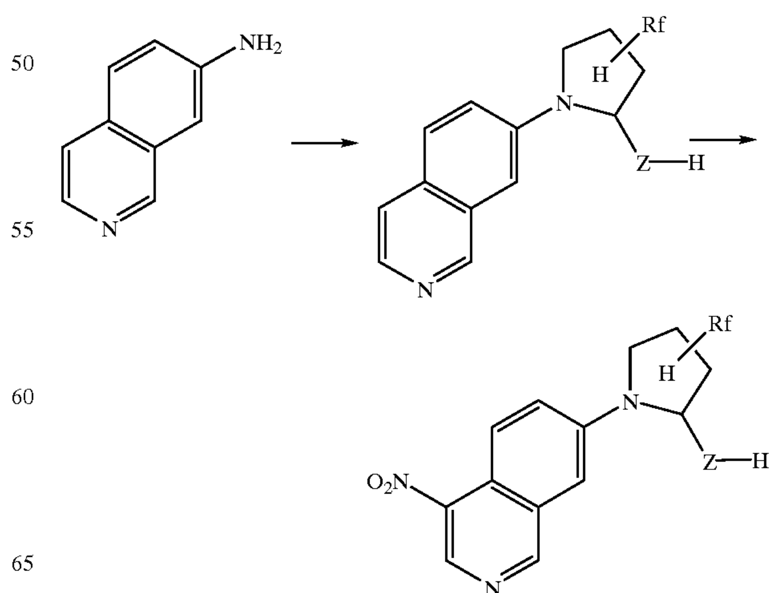
SCHEME 2d
