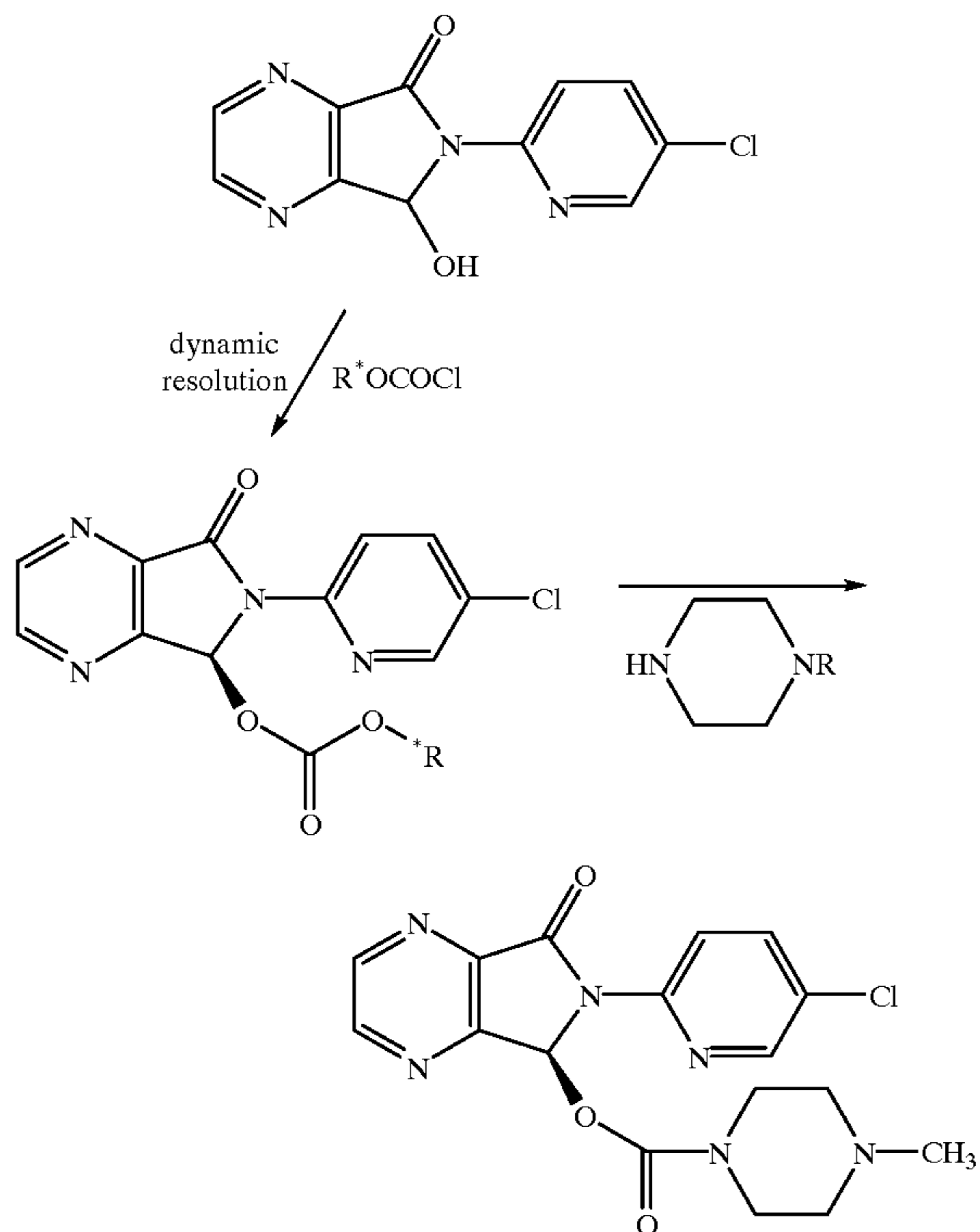
Scheme 6
