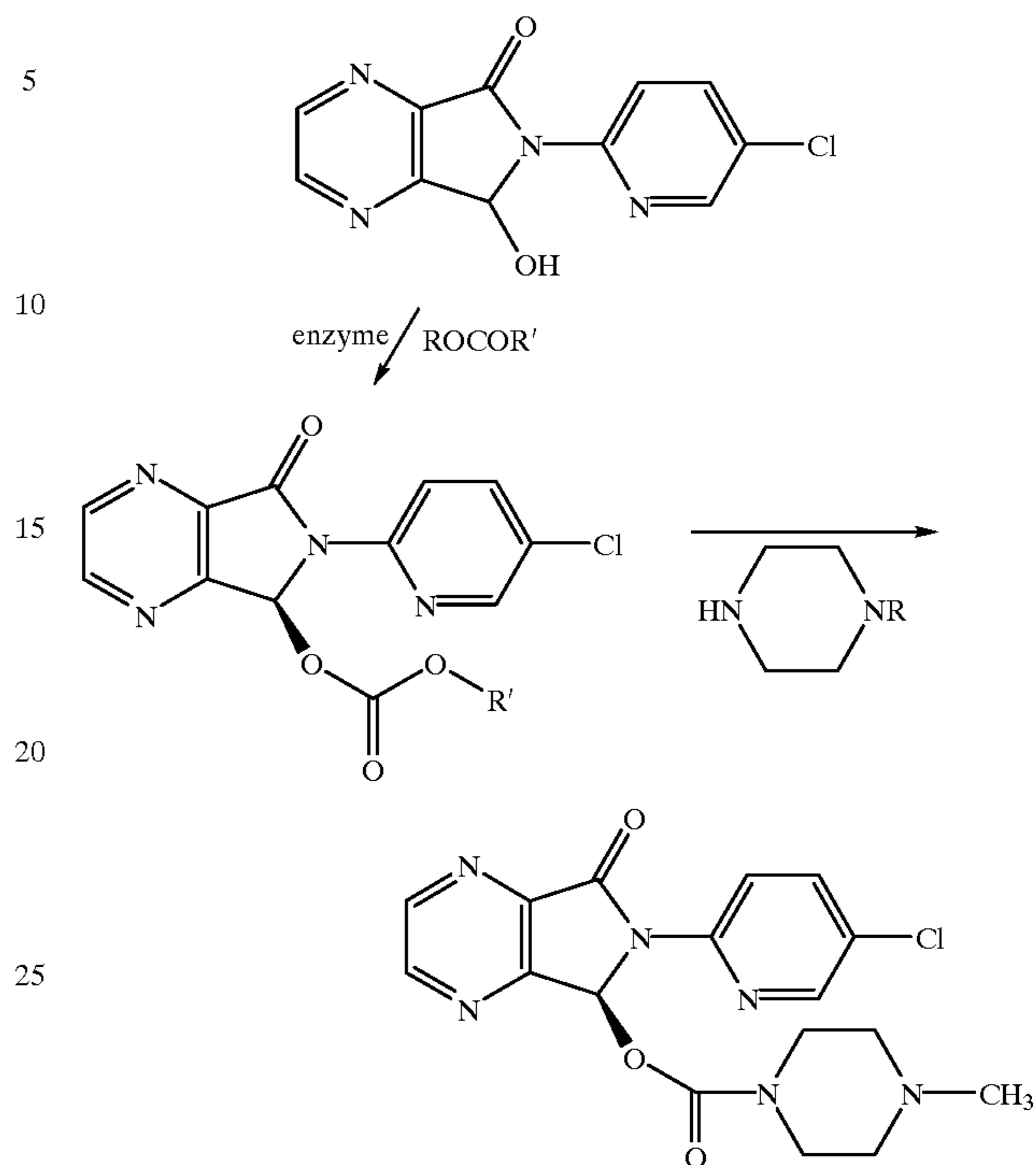
Scheme 7
