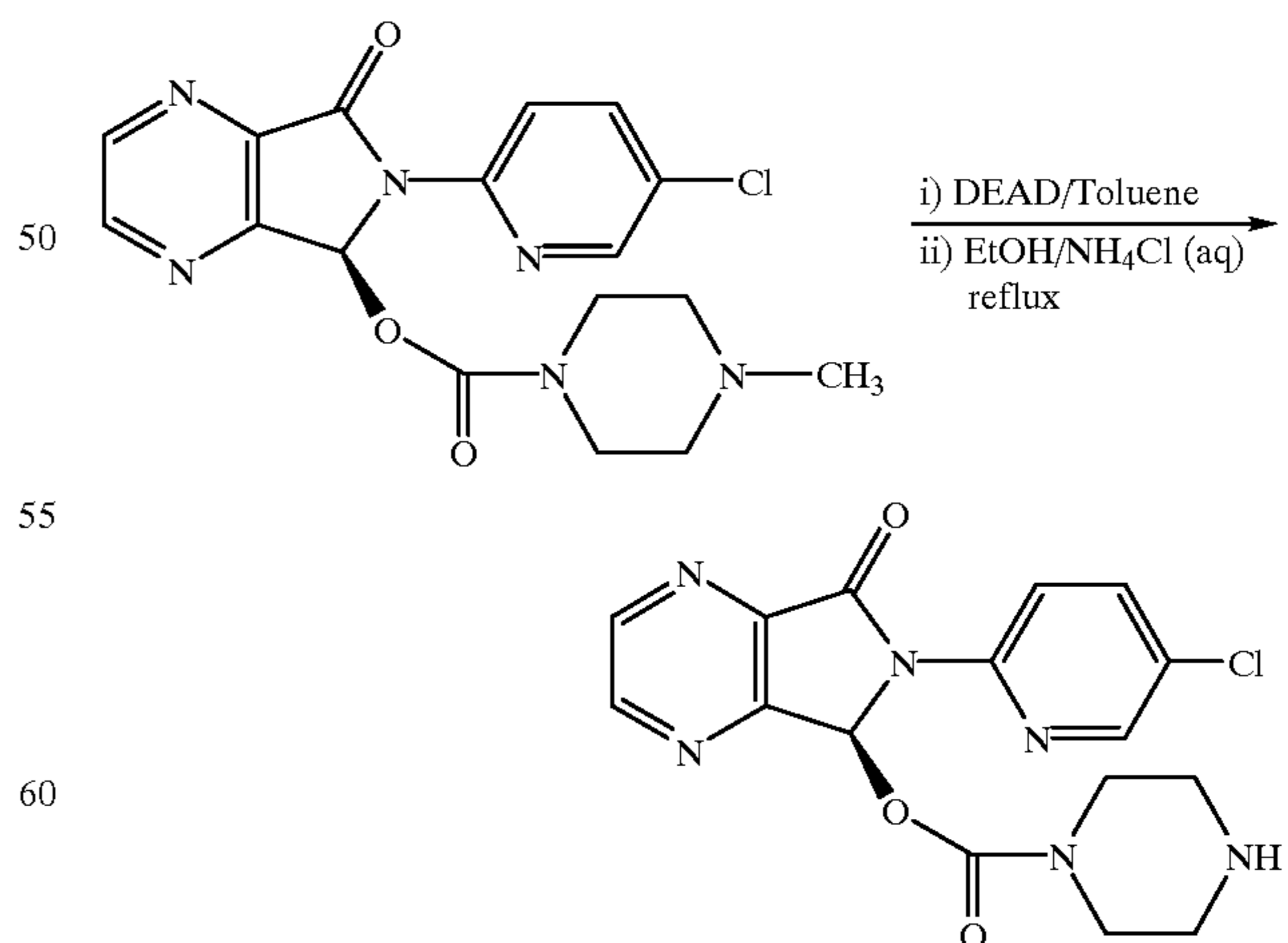
Scheme 8
