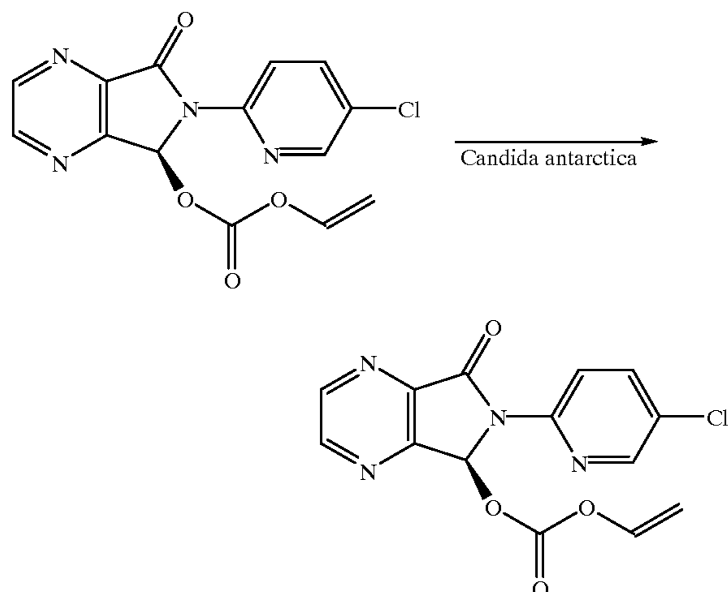
Scheme 3
