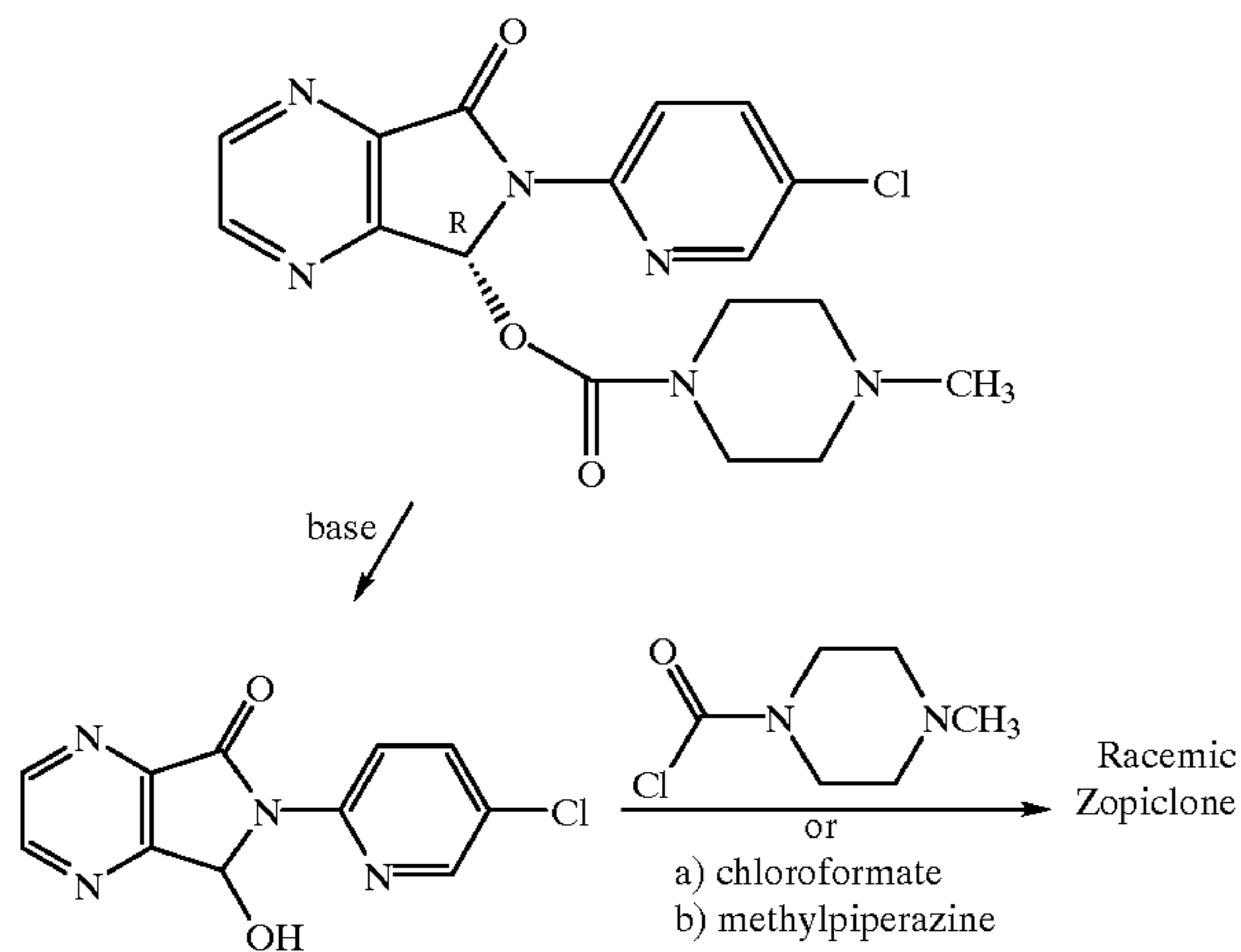
Scheme 5
