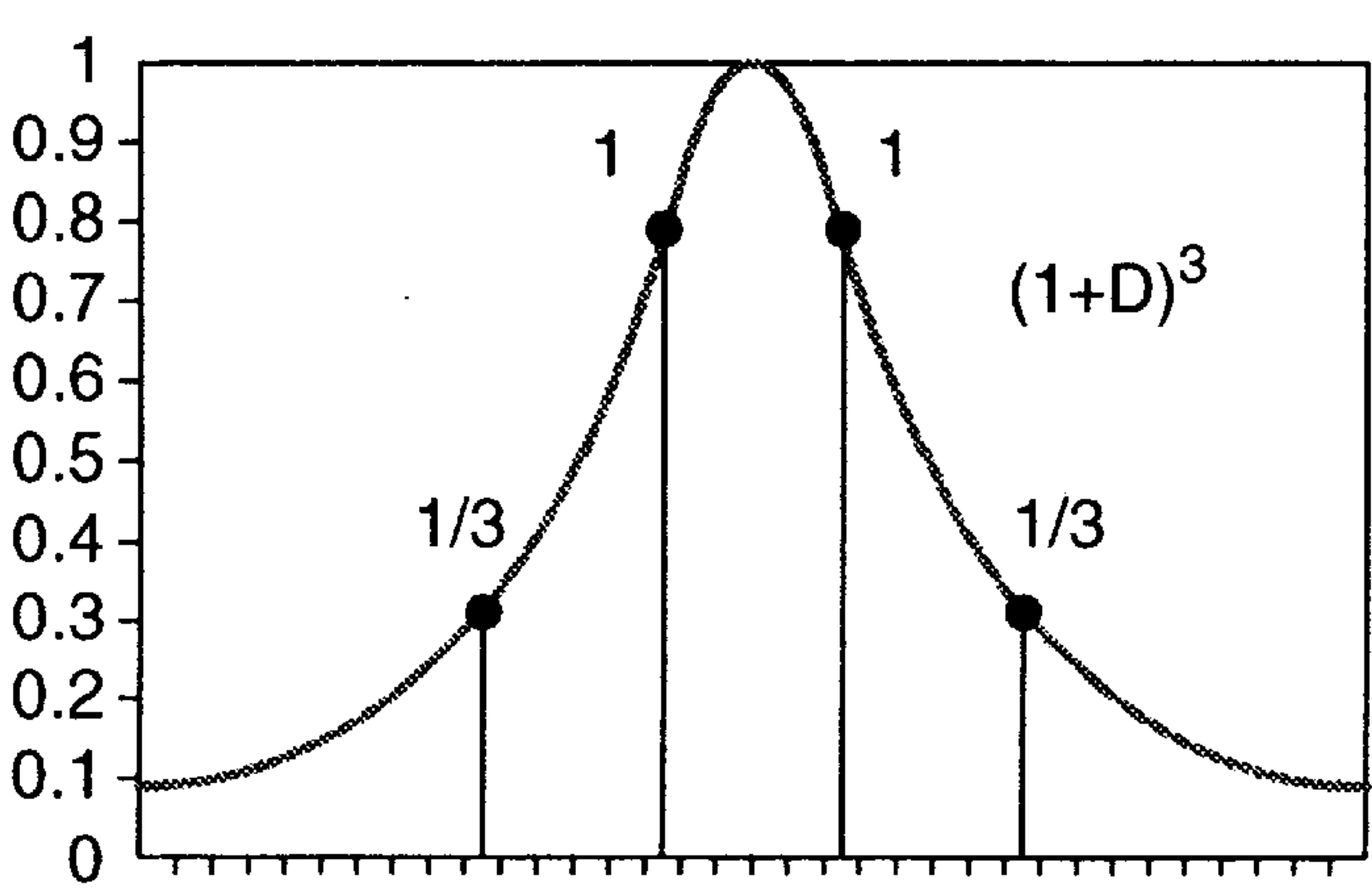
FIG.3C PRIOR ART
