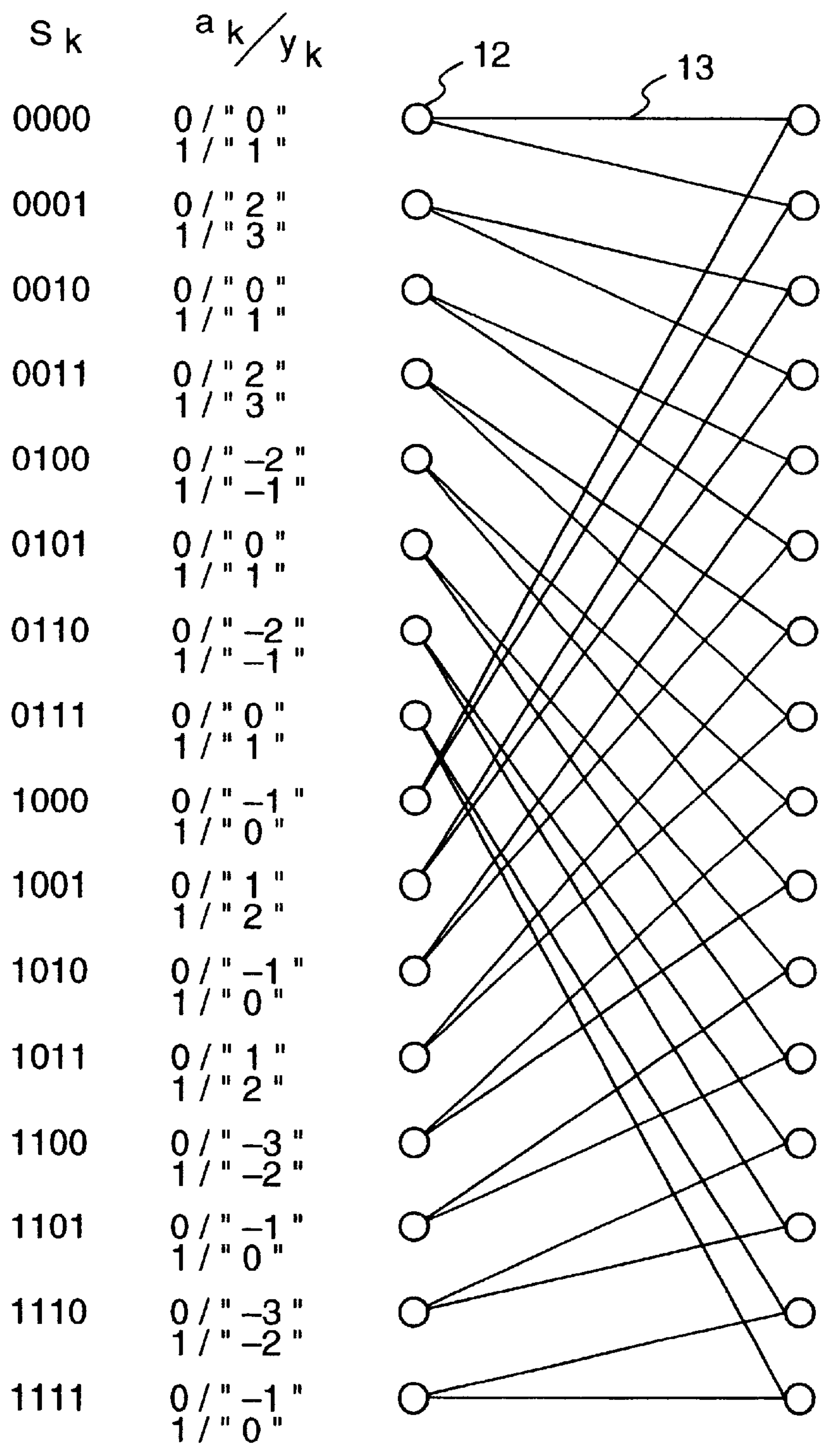
FIG.5 PRIOR ART
